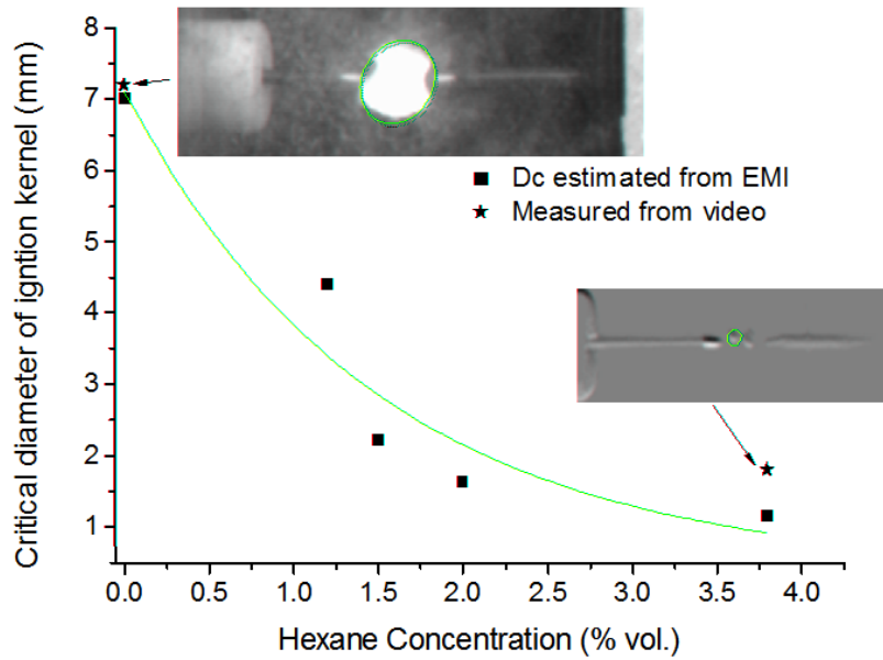
Figure 1.5. Estimated critical kernel sizes of sunflower-oilcakes and hexane mixtures using Equation 1.6 (Khalili et al., 2012)
