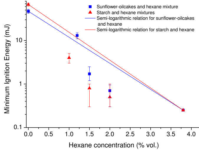
Figure 1.1. Behaviour of the Minimum Ignition Energy of hybrid mixtures of sunflower-oilcakes/hexane and starch ( d_{50} = 70 \mu\text{m} )/hexane according to the hexane content (Khalili et al., 2012)
