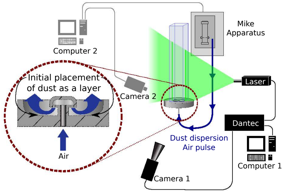
Figure 3.4. Diagram showing experimental setup for Particle Image Velocimetry (PIV) analysis in a square-section vertical tube.
