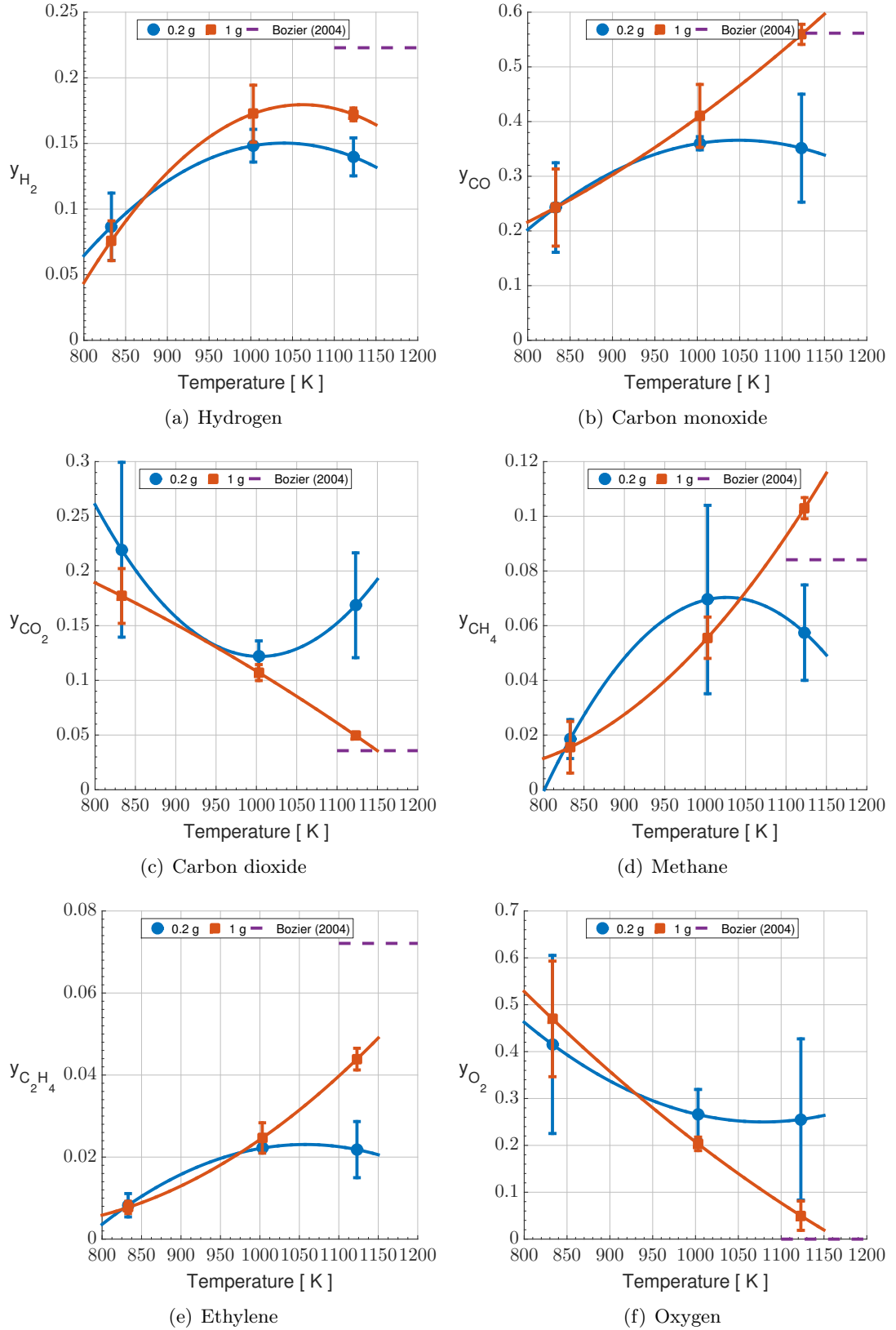
Figure 2.3. Molar concentrations of the gas products from the flash pyrolysis of starch. The masses in the legends are those of starch introduced in the chamber prior dispersion. The error bars represent confidence intervals of 95%. \Delta P = 0.03 bar.
