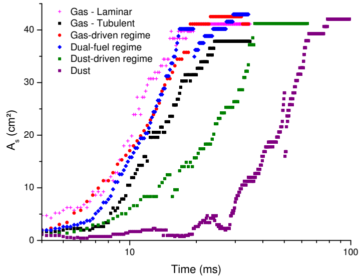
Figure 4.13. Cross section area of flame in terms of time
