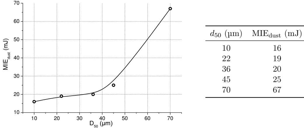
Figure 1.2 and Table 1.1 Minimal Ignition energies of sieved samples of starch (Khalili et al., 2012)
