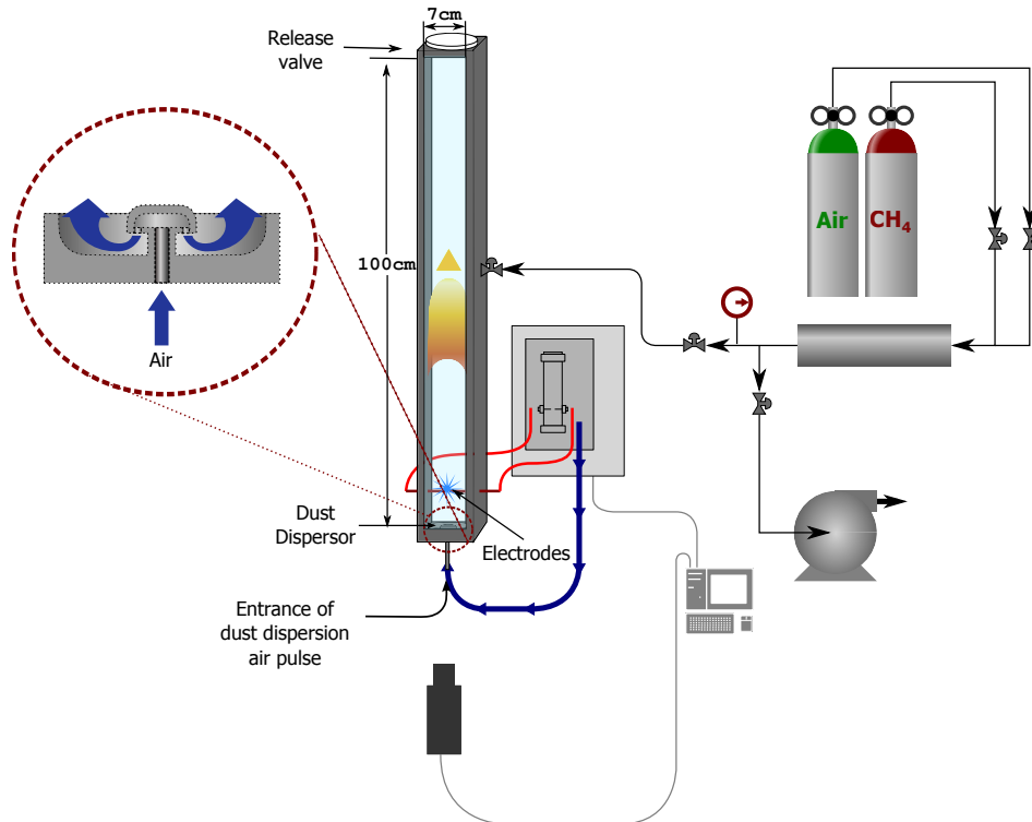
Figure 4.1. Equipment for flame propagation measurements
