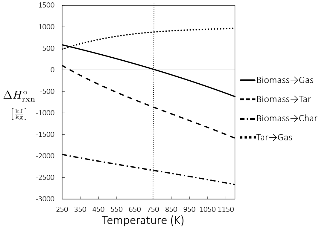
Figure 2.9. Enthalpies of reaction of biomass pyrolysis. Calculated with the values in Table 2.3
