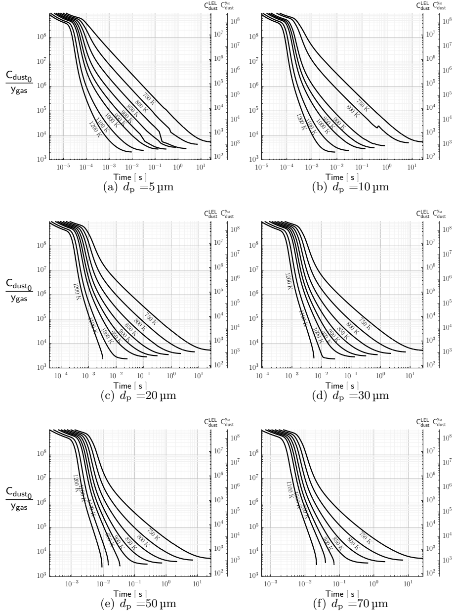
Figure C.38. Initial C_{\text{dust}} necessary to reach a concentration of y_4 in pyrolysis gases at time t using to Chan kinetics, auxiliary axes on the left show the initial concentration necessary to reach the LEL = 7.8% and the stoichiometric concentration (23%) of pyrolysis gases. Units for C_{\text{dust}} are in \frac{\text{g}}{\text{m}^3}
