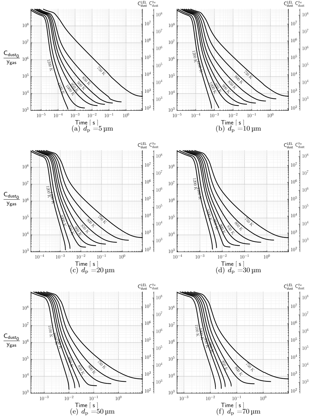
Figure 2.18. Initial C_{dust} necessary to reach a concentration of y_4 in pyrolysis gases at time t using to Wagenaar kinetics, auxiliary axes on the left show the initial concentration necessary to reach the LEL = 7.8% and the stoichiometric concentration (23%) of pyrolysis gases. Units for C_{dust} are in \frac{g}{m^3}
