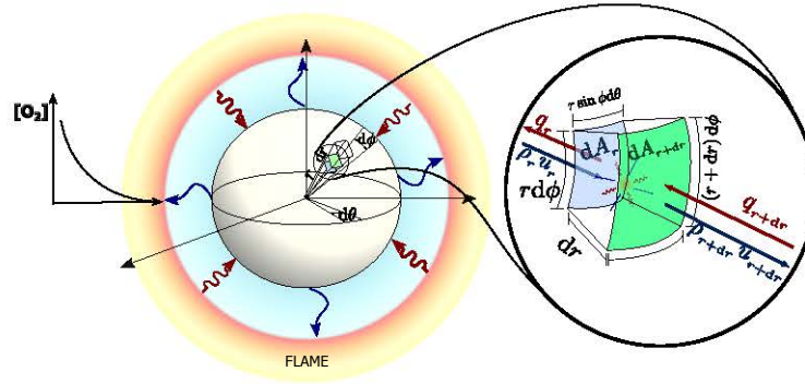
Figure 2.8. Representation of the discrete volume for solution of the pyrolysis of a sphere of biomass
