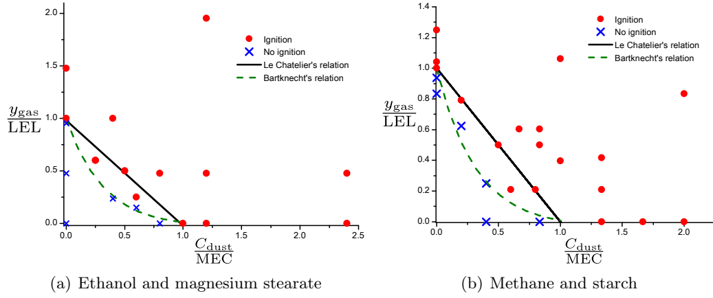
Figure 1.7. Representation of hybrid mixture explosive limits, using Bartknecht and Le Chatelier models
