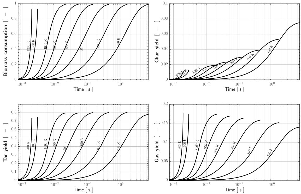
Figure 2.17. Component yields using Di Blasi and Branca kinetics. d_p = 20 \mu\text{m}
