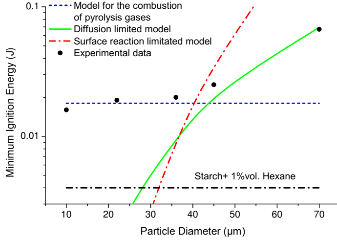
Figure 1.3. Influence of the particle size on the MIE of starch samples (Khalili et al., 2012)
