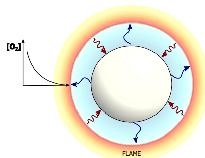
Figure 2.1. Representation of the pyrolysis of an organic particle inside a flame due to lack of oxygen
