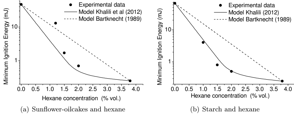
Figure 1.6. Minimum Ignition Energy for sunflower-oilcakes and starch with hexane compared to Bartknecht's (1989) and Khalili's (2012) models, Equations 1.1 and 1.15 respectively
