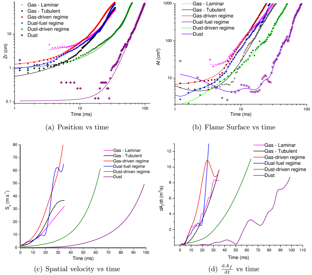
Figure 4.6. Behaviour of flame position, surface, spatial velocity, and rate of flame surface change in time
