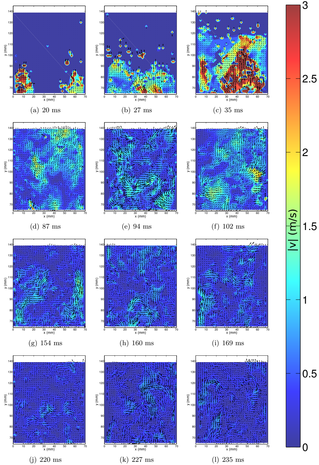
Figure 3.9. Velocity vector fields for the PIV analysis of 78 mg of wheat starch. Results from a same dust dispersion are grouped in columns.
