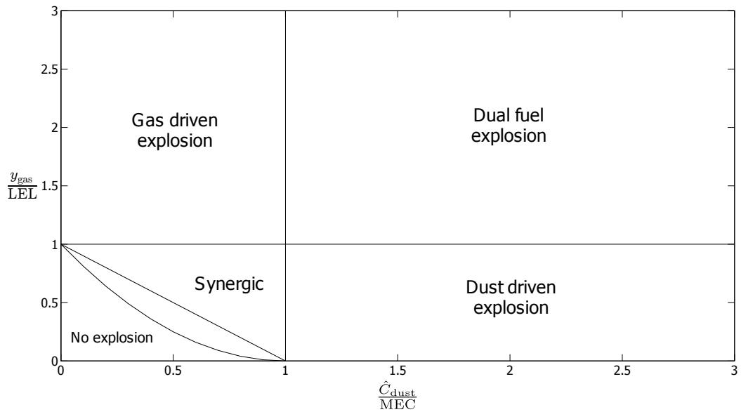
Figure 1.11. Explosion regimes of hybrid mixtures according to their composition as proposed by Garcia-Agreda et al. (2011) and Sanchirico et al. (2011)
