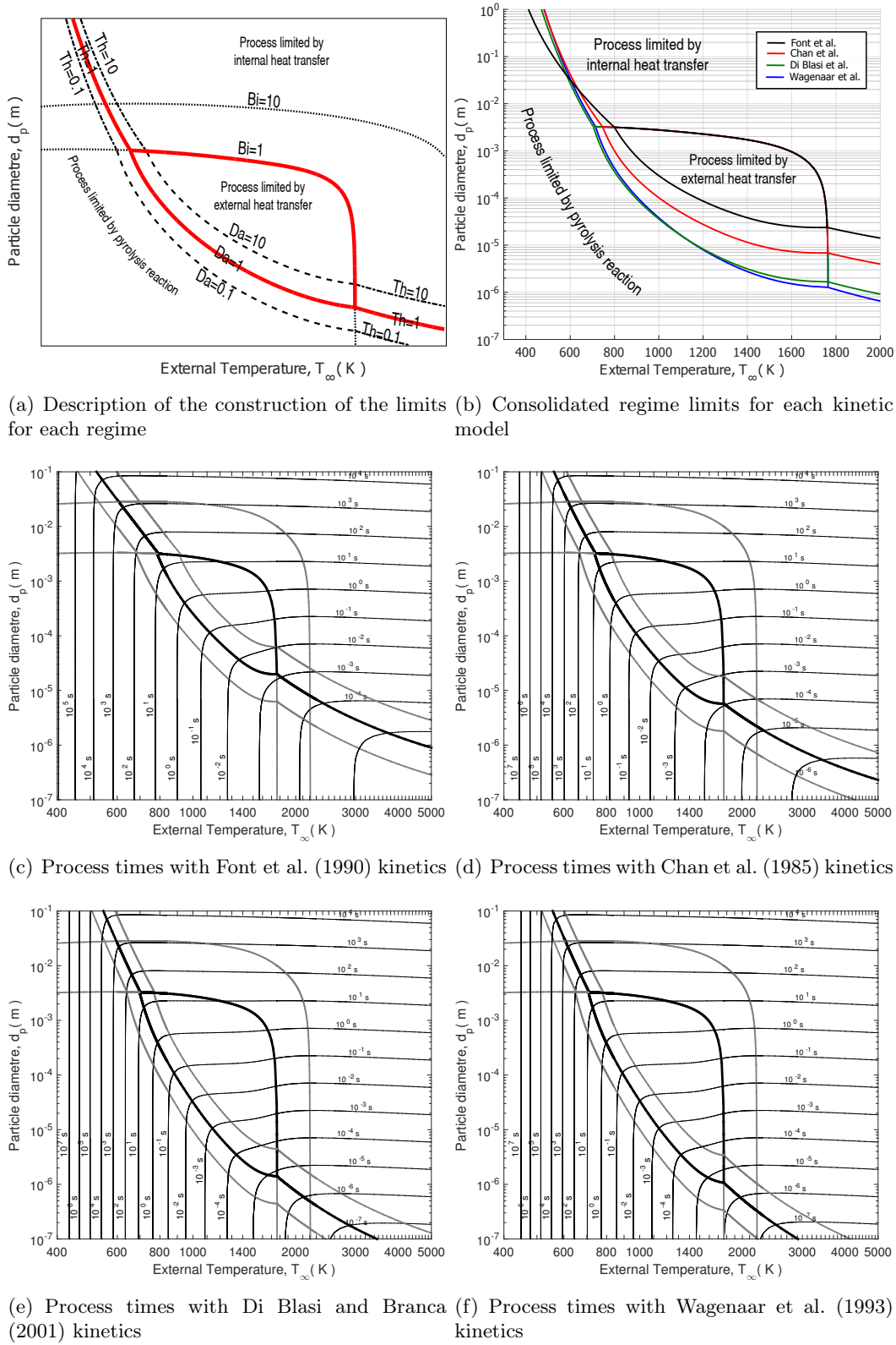
Figure 2.13. Pyrolysis limiting regimes according to the particle size, the external temperature and the kinetic model. Time contours in subfigures (c) to (f) represent the addition of the characteristic times; \tau_{ext} , \tau_{int} and \tau_{pyro}
