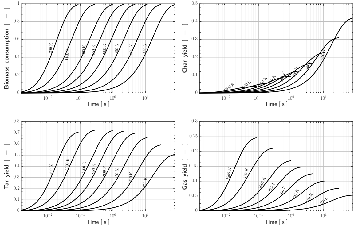
Figure 2.15. Component yields using Font et al. kinetics. d_p = 20 \mu\text{m}
