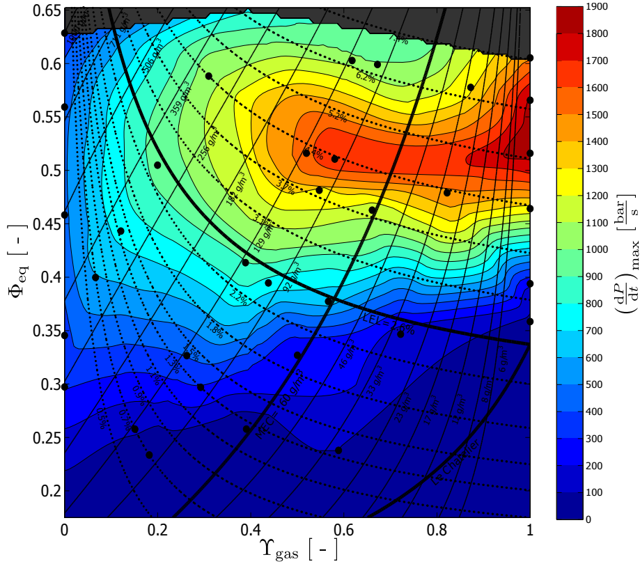
Figure 1.12. Rate of pressure rise map for the niacin/acetone mixtures with t_v = 60 ms. \gamma_{\text{gas}} and \Phi_{\text{eq}} are defined by Equations 1.25 and 1.28 respectively. y_{\text{gas}} and C_{\text{dust}} are represented by the pointed and solid lines respectively. (Sanchirico et al., 2011)
