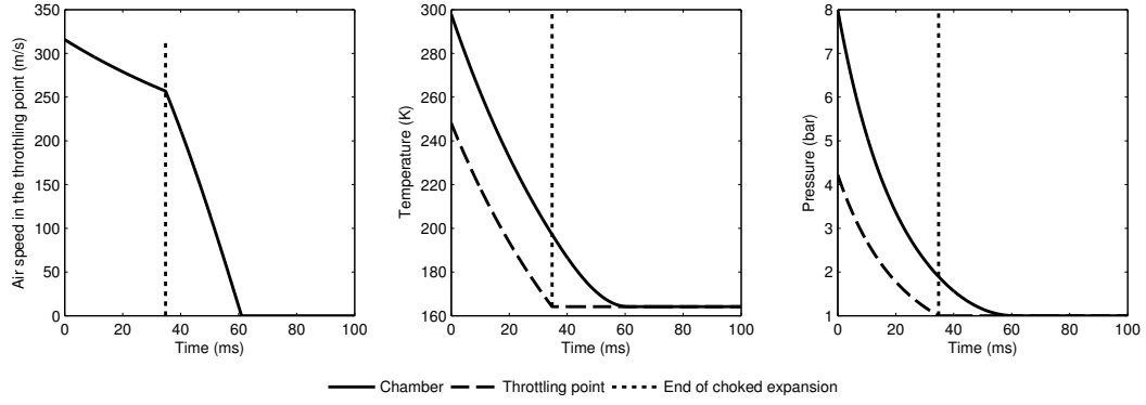
Figure 3.7. Behaviour of speed, pressure and temperature for the isentropic decompression of air in a 50 mL chamber through an orifice with a 3.23 mm diameter, with initial pressure of 8 bar. The end of the choked expansion happens at 35 ms whereas the whole expansion finishes after 61 ms
