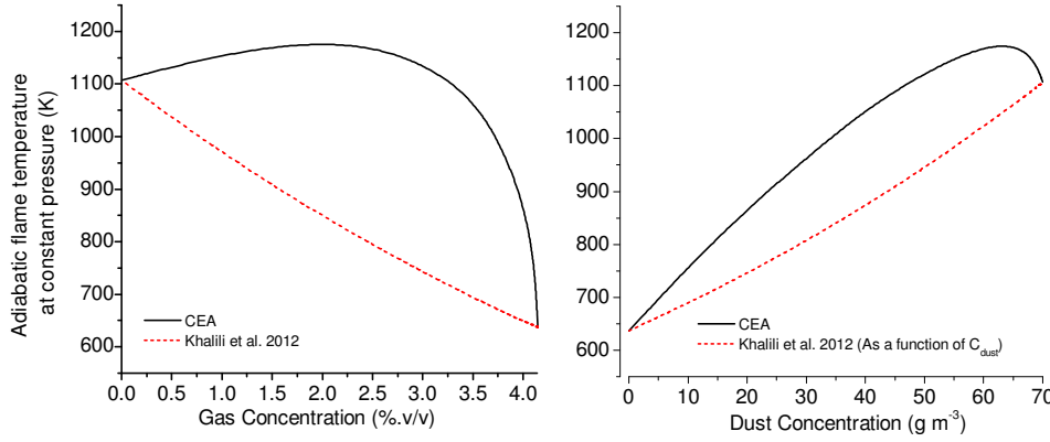
Figure 1.10. Adiabatic flame temperature at constant pressure for mixtures of hydrogen-starch. The black line represents values calculated with the CEA software using gas and dust concentrations reported by Hertzberg and Cashdollar (1987) and presented in Figure 1.9 † . The red pointed line at the left represents Khalili's model in Equation 1.19 and the right one represents Equation 1.19
