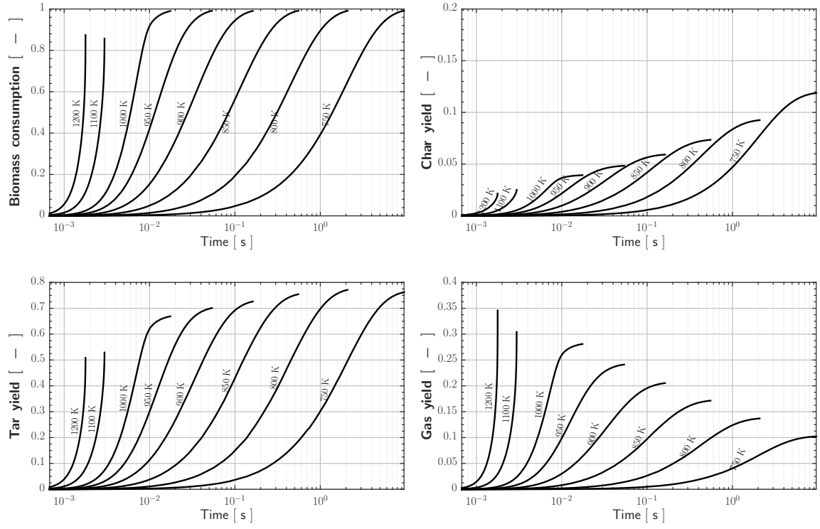
Figure 2.16. Component yields using Wagenaar et al. kinetics. d_p = 20 \mu\text{m}
