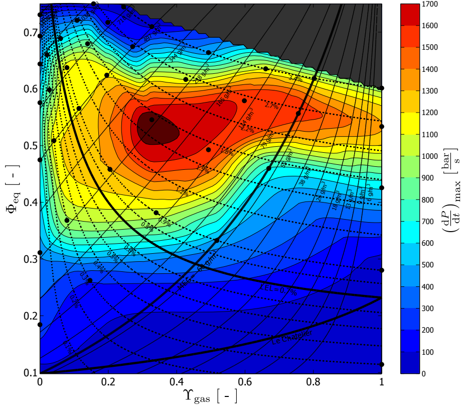
Figure 1.15. Rate of pressure rise map for the niacine/diisopropyl-ether mixtures. \Upsilon_{\text{gas}} and \Phi_{\text{eq}} are defined by Equations 1.25 and 1.28 respectively. y_{\text{gas}} and C_{\text{dust}} are represented by the pointed and solid lines respectively. (Dufaud et al., 2009)
