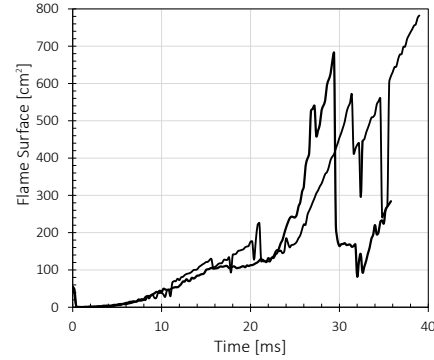
Figure 4.5. Estimation of the surface of the flame using the MOSES for two videos of flames in dual-fuel regime
