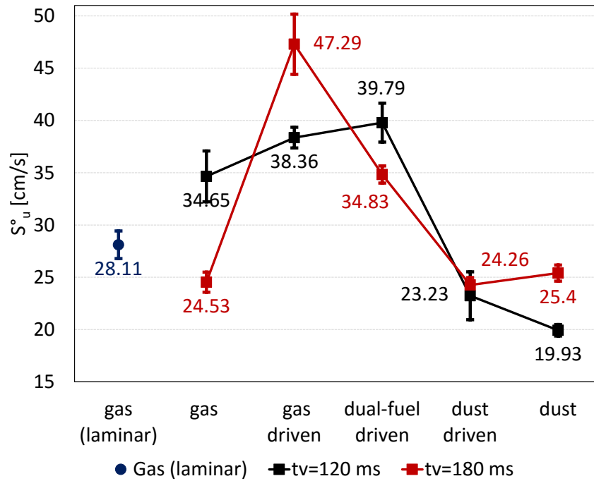
Figure 4.14. Burning velocities of methane/starch mixtures deduced from video analysis of flame propagation
