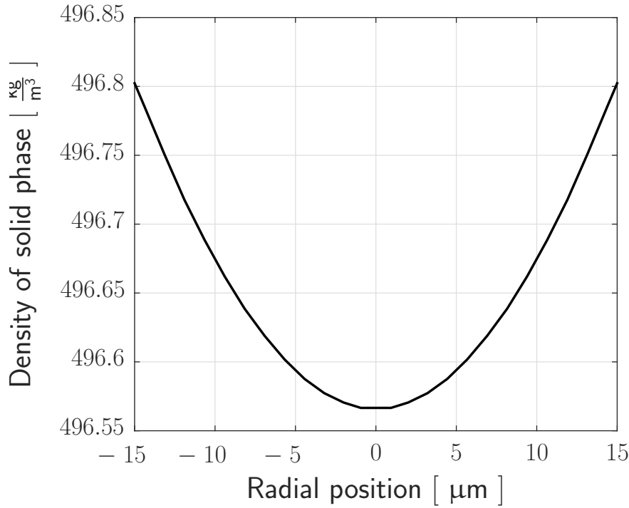
Figure 2.12. Density of solid phase of a 30 \mu\text{m} particle after 150 ms. Pyrolysis at 850 K using Wagenaar et al., 1993 constants and external velocity equal to \sigma_p .
