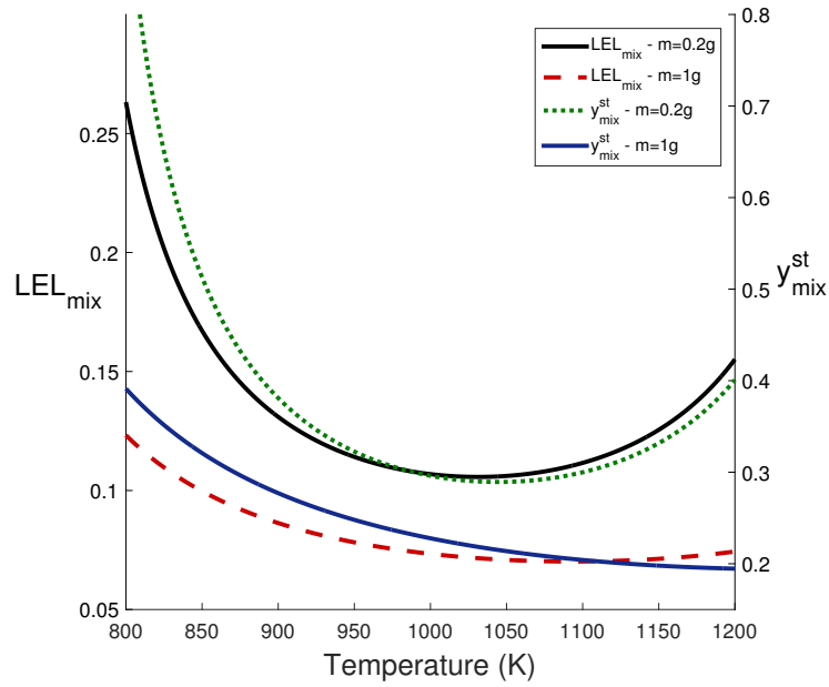
Figure 2.5. Lower explosive limit ( LEL_{mix} ) and stoichiometric concentration ( y_{mix}^{st} ) of pyrolysis gases from flash volatilization of starch in air.
