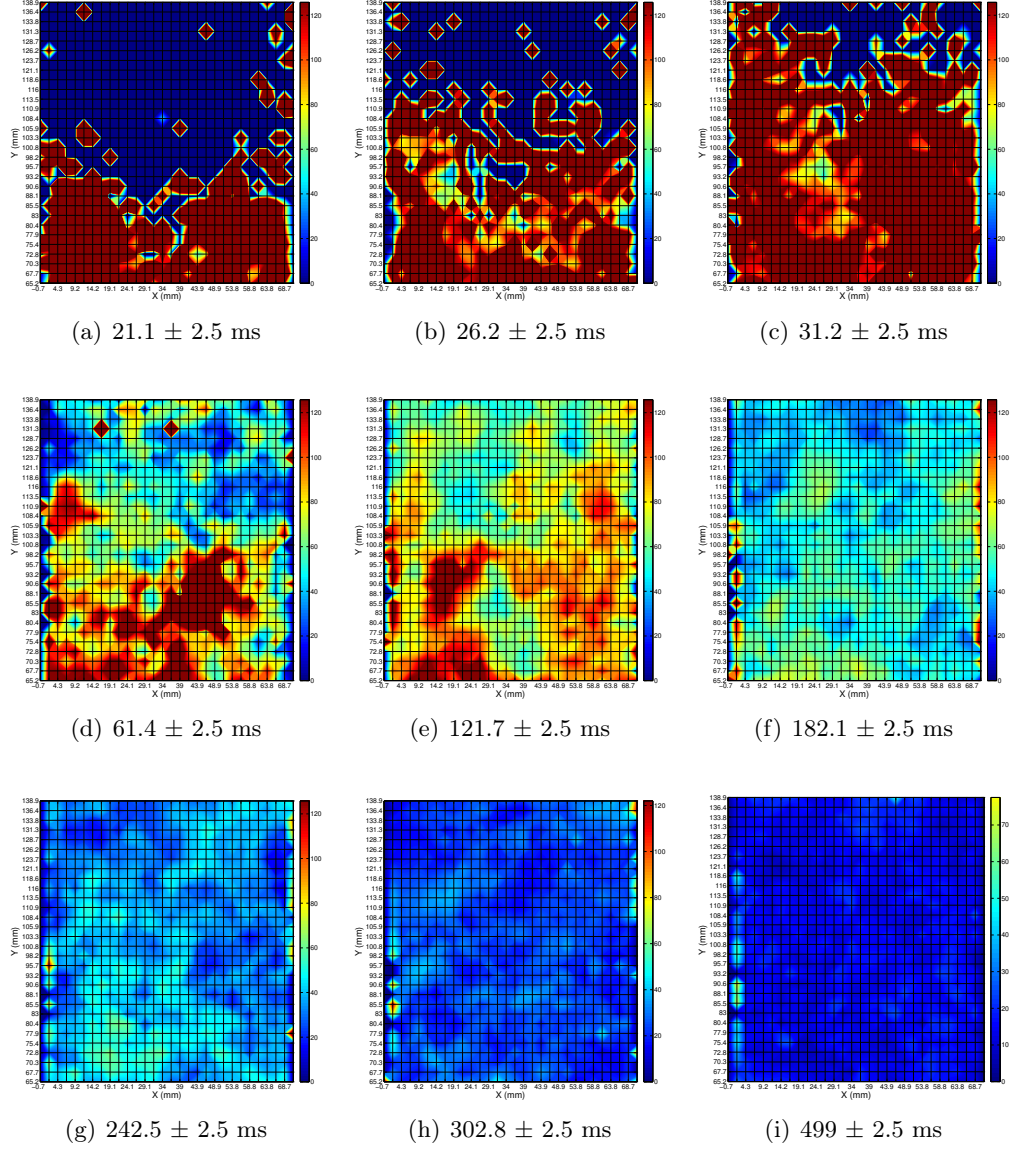
Figure 3.11. Turbulence intensity map for different times
