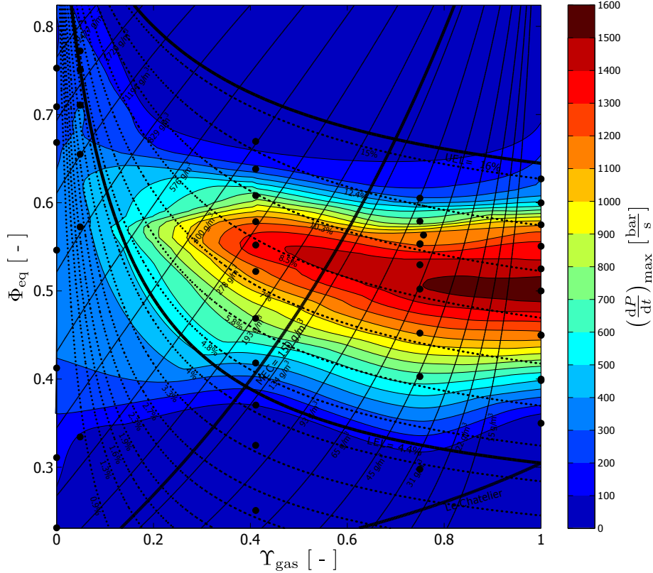
Figure 1.16. Rate of pressure rise map for the starch/methane mixtures. \Upsilon_{\text{gas}} and \Phi_{\text{eq}} are defined by Equations 1.25 and 1.28 respectively. y_{\text{gas}} and C_{\text{dust}} are represented by the pointed and solid lines respectively
