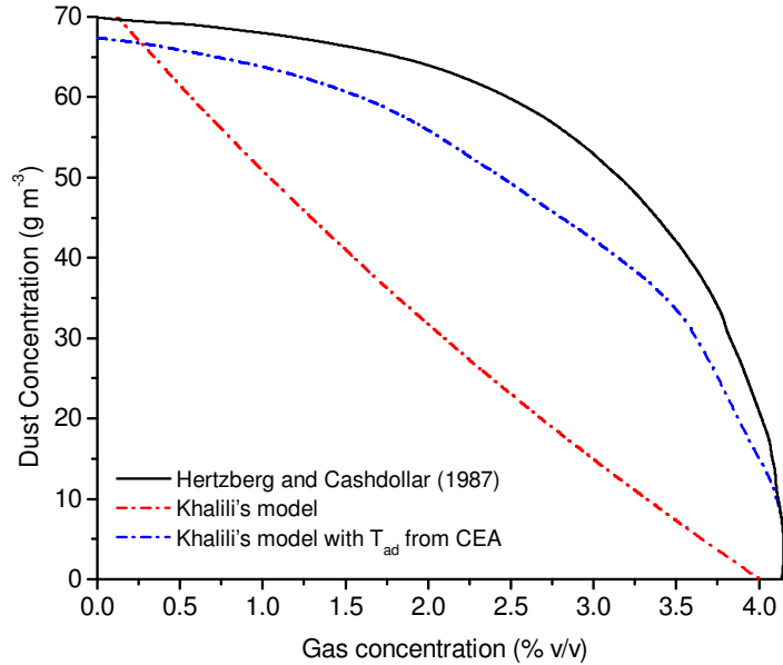
Figure 1.9. Lower concentration flammability limits of hydrogen and corn-starch
