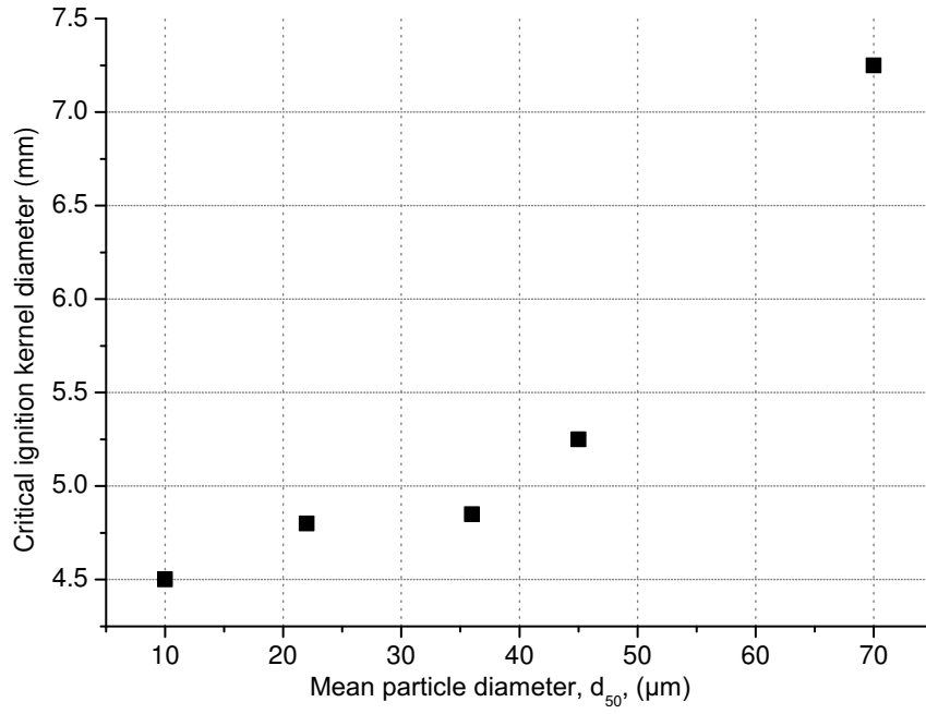
Figure 1.4. Estimated critical kernel sizes vs. starch particle diameter using Equation 1.6 and the data from Table 1.1 (Khalili et al., 2012)
