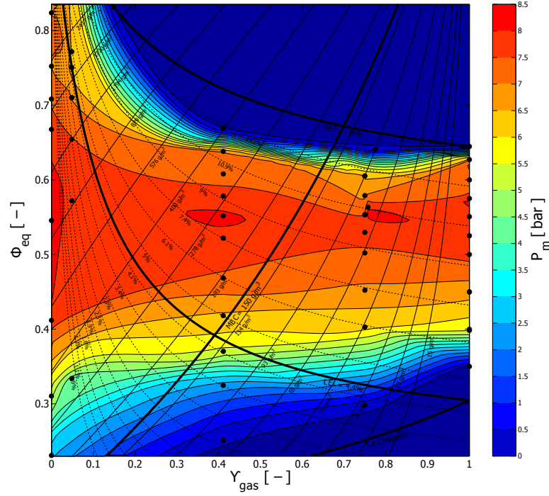
Figure 1.18. Overpressure map for the starch/methane mixtures. Y_{gas} and \Phi_{eq} are defined by Equations 1.25 and 1.28 respectively. y_{gas} and C_{dust} are represented by the pointed and solid lines respectively
