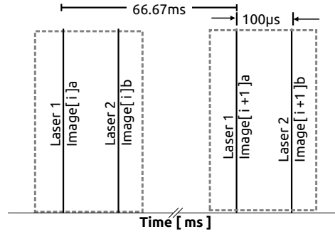
Figure 3.5. PIV laser and image shot setup for the set of experiments of glass beads described in Table 3.1 Dark lines represent the first and second pulse of the laser as well as the respective pictures a and b. The pointed gray lines enclose the elements of analysis necessary to produce estimate one velocity field
