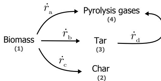
Figure 2.7. General reaction path of flash pyrolysis of Biomass
