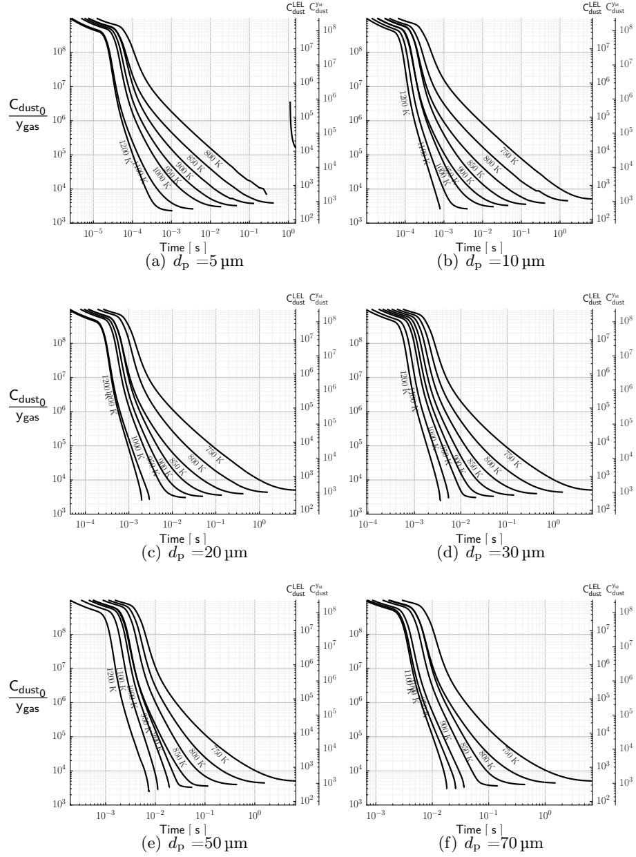
Figure C.19. Initial C_{\text{dust}} necessary to reach a concentration of y_4 in pyrolysis gases at time t using to DiBlasi kinetics, auxiliary axes on the left show the initial concentration necessary to reach the LEL = 7.8% and the stoichiometric concentration (23%) of pyrolysis gases. Units for C_{\text{dust}} are in \frac{\text{g}}{\text{m}^3}
