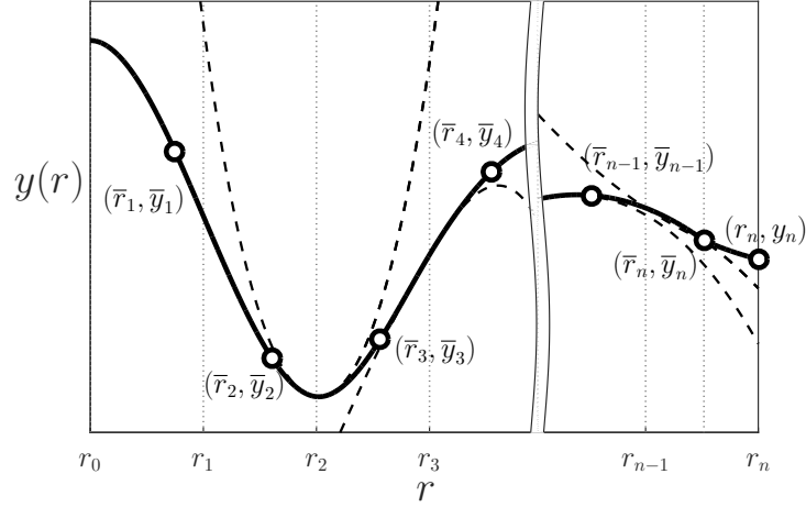
Figure B.1. Representation of a spline function. The thick continuous line represents the spline function \mathbb{Y}(r) , while the dashed lines represent any of the polynomials Y_i(r) that compose it. Vertical lines represent the points at which the polynomials are interrupted. \bar{y}_i(r) are the values of Y(r) at the centre of mass of the interval (r_{i-1}, r_i) .
