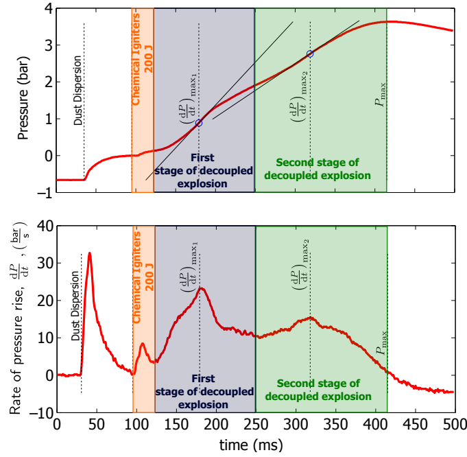
Figure 1.19. Decoupled explosion in synergic regime. Explosion produced in the 20L with a hybrid mixture of starch at 106.6 \frac{\text{g}}{\text{m}^3} and methane at 3.41 %vol, t_v = 60 \text{ ms} and chemical igniters of 200 J.
