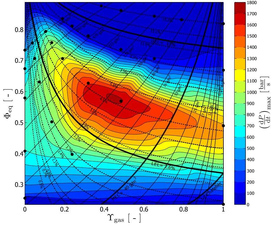
Figure 1.13. Rate of pressure rise map for the telithromycine-acetone mixtures. \Upsilon_{\text{gas}} and \Phi_{\text{eq}} are defined by Equations 1.25 and 1.28 respectively. y_{\text{gas}} and C_{\text{dust}} are represented by the pointed and solid lines respectively. (Traore, 2007)
