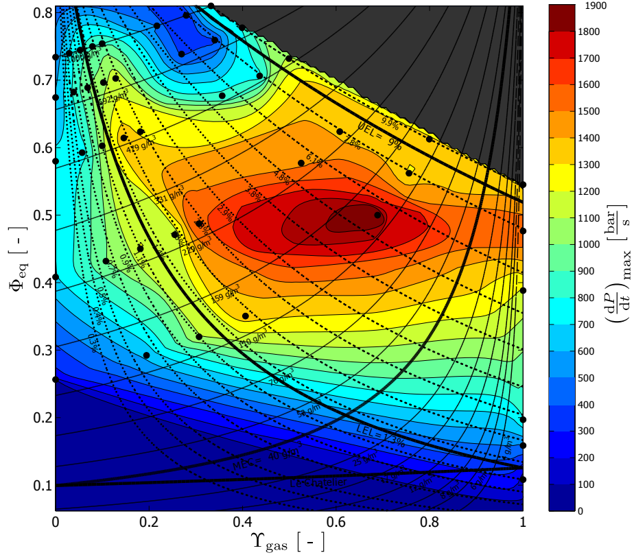
Figure 1.14. Rate of pressure rise map for the telithromycine/toluene mixtures. \Upsilon_{\text{gas}} and \Phi_{\text{eq}} are defined by Equations 1.25 and 1.28 respectively. y_{\text{gas}} and C_{\text{dust}} are represented by the pointed and solid lines respectively. (Dufaud et al., 2009)
