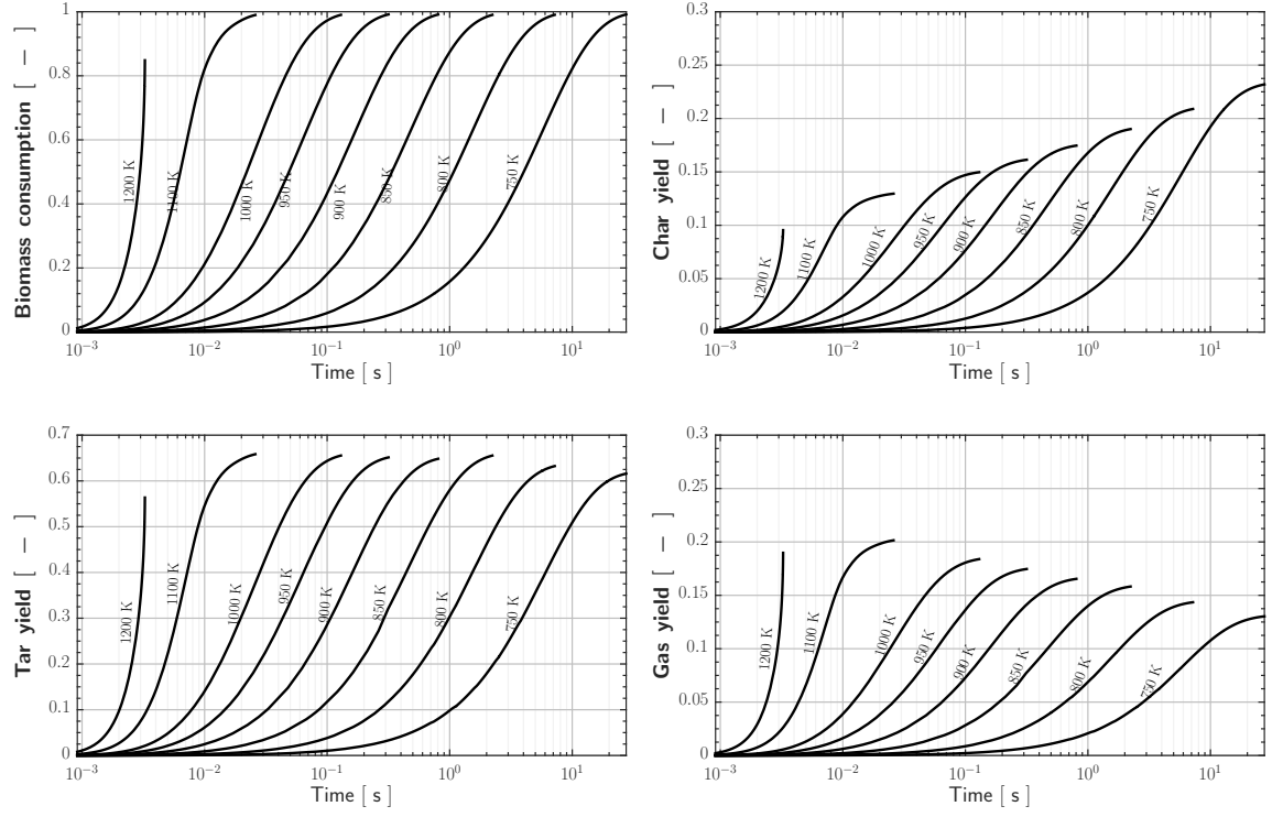
Figure 2.14. Component yields using Chan et al. kinetics. d_p = 20 \mu\text{m}
