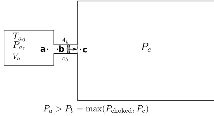
Figure 3.6. Representation for the free isentropic expansion of a pressurized chamber through a leak
