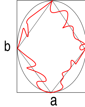
Figure D.2. Representation of the rectangle, the ellipse and the rhombus with equivalent height and width to that of the flame's profile
