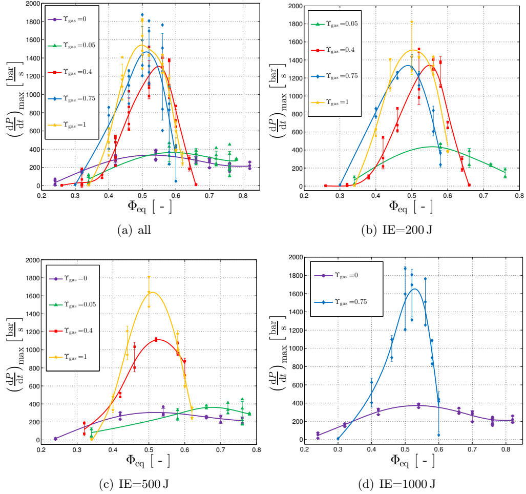
Figure A.1. Experimental results of pressure rise rate, \left(\frac{dP}{dt}\right)_{\max} for starch-methane mixtures, separated according to the ignition energy of the chemical igniters used
