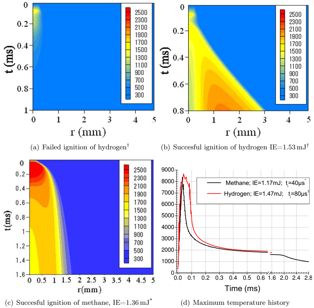
Figure 2.19. Behaviour of temperature during and after spark ignition of methane * and hydrogen † according to simulations involving detailed chemistry. * Han et al. (2010) † Han et al. (2011)
