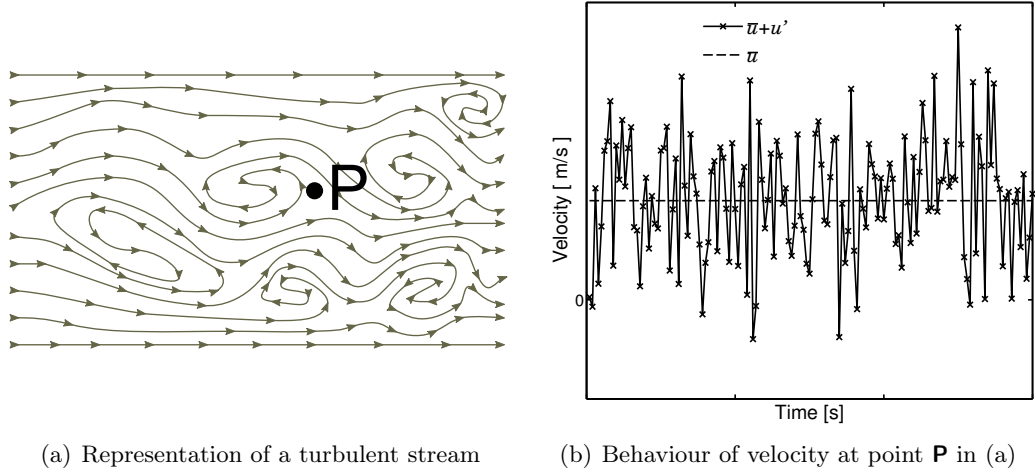
Figure 3.8. Representation of the behaviour of the velocity in a fixed point of a turbulent stream. Velocity is represented in (b) with the solid crossed line and is composed of its mean value \bar{u} (pointed line) and the velocity fluctuations u' .
