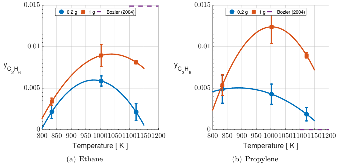
Figure 2.4. Molar concentrations of the gas products from the flash pyrolysis of starch. The masses in the legends are those of starch introduced in the chamber prior dispersion. The error bars represent confidence intervals of 95%. \Delta P = 0.03 bar.
