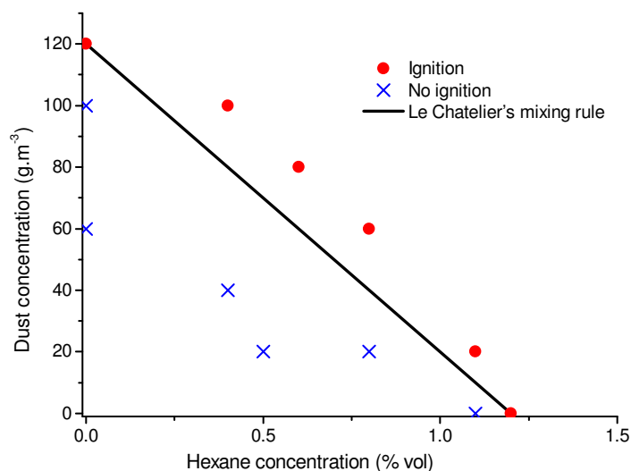
Figure 1.8. Explosive limits of sunflower-oilcakes and hexane
