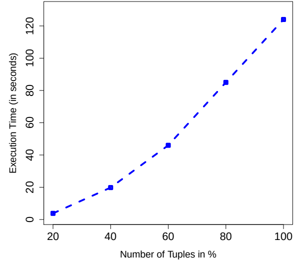
(b) Runtime for Building \mathcal{L}_{YAGO}
