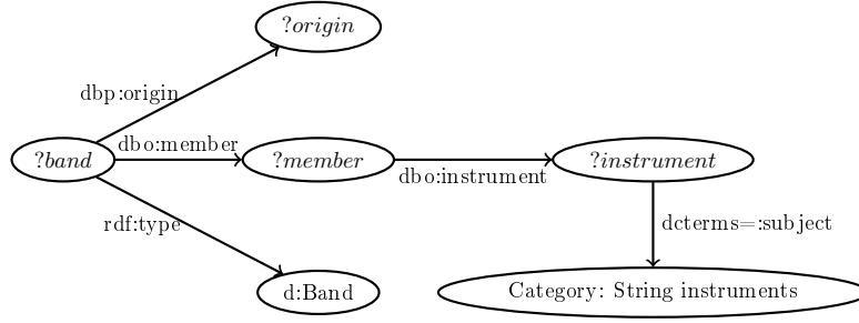
Figure 2.3: Basic Graph Pattern for query in Listing 2.1 from DBpedia matched against the RDF graph in Figure 2.2. The prefixes dbo:, db:, dbp: stand for dbpedia-owl:, dbpedia: and dbpprop: respectively.
