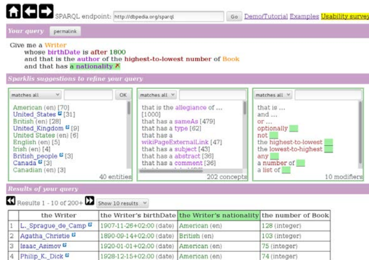
Figure 2.8: SPARKLIS Query Builder.
