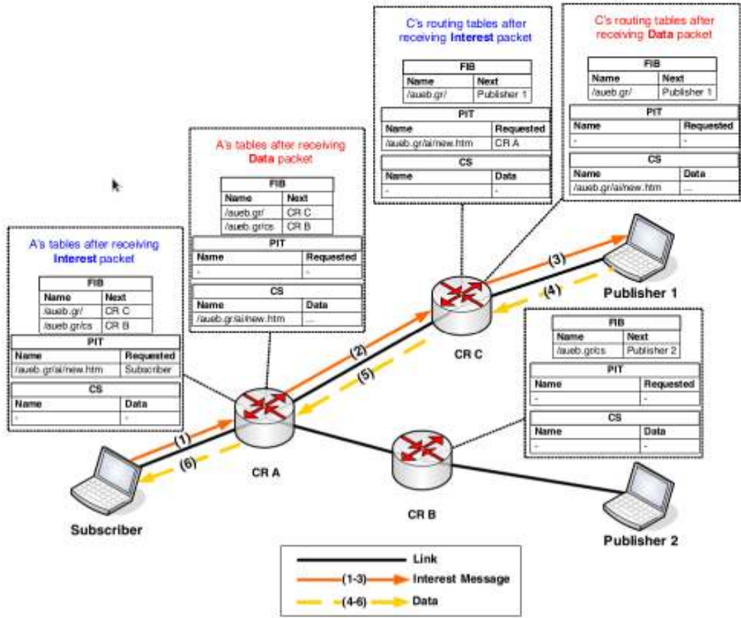
Figure 2.1: CCN Architecture, extracted from [20]
