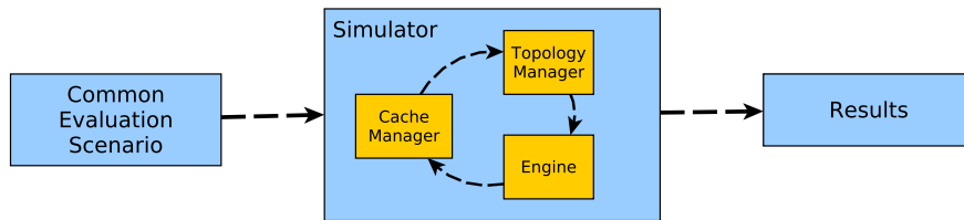
Figure 4.3: Simulator architecture
