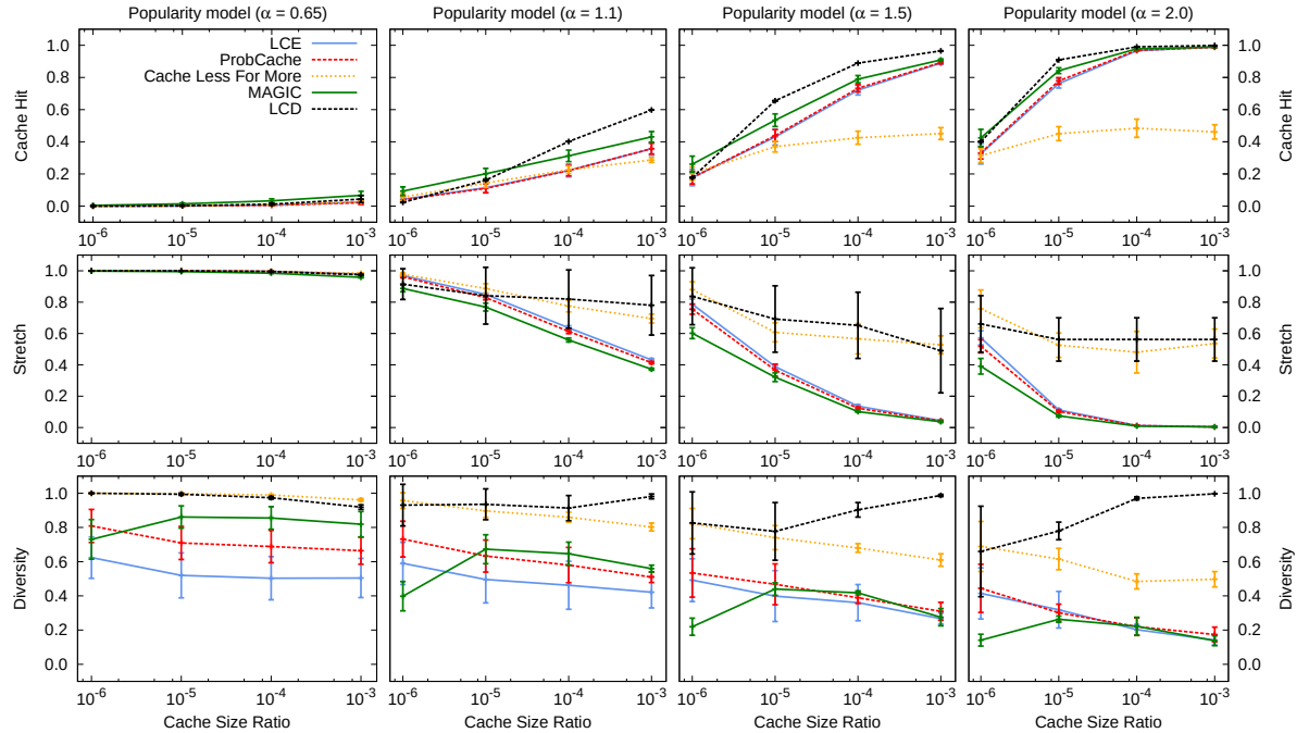
Figure 4.4: Comparison of the Caching Strategies
