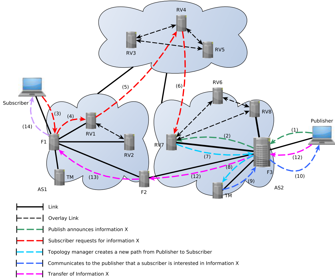
Figure 2.2: The PURSUIT Architecture
