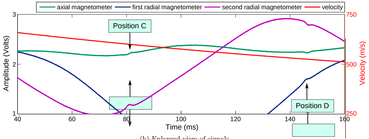
(b) Enlarged view of signals
