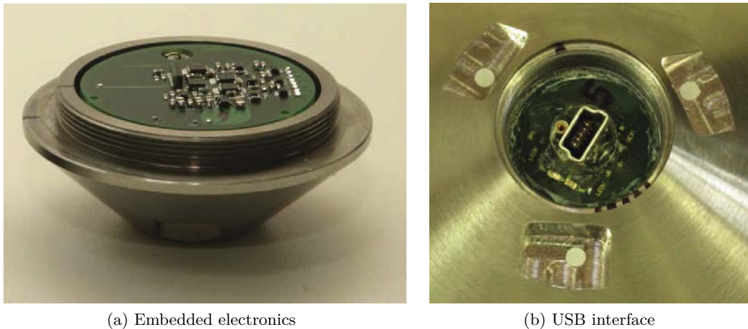
Figure 1.5: Electronic package of the space probe model
