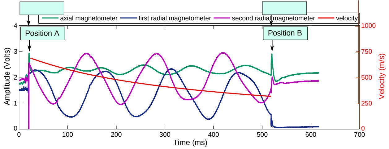
(a) Magnetometer and radar signals
