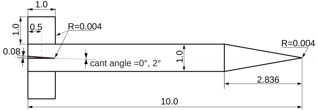
Figure 1.2: Schematic of the Basic Finner projectile
