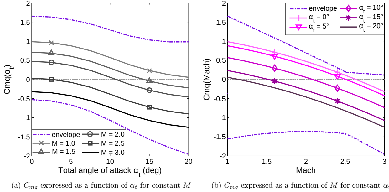
Figure 4.12: Estimated pitch damping coefficient C_{mq} based on multiple data series and the lower and upper curves of the constraint envelope
