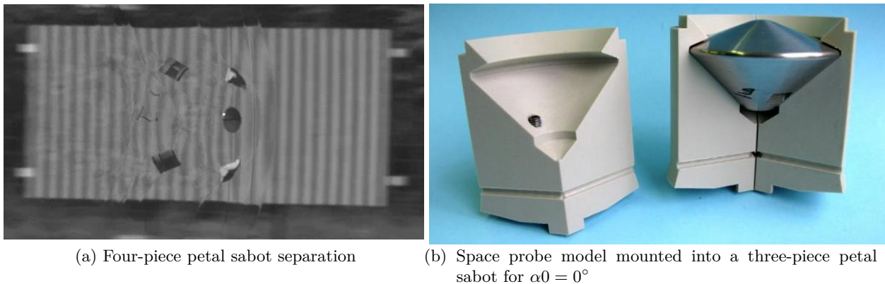
Figure 1.3: Sabot for a space probe model
