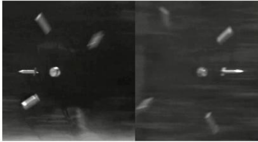
Figure 4.25: Snapshots of sabot separation obtained from the two trajectory trackers
