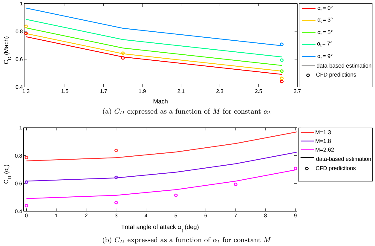
Figure 4.29: Estimated drag coefficient C_D based on multiple data series compared to CFD predictions
