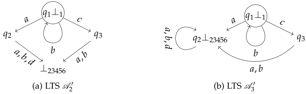
Figure 3.14: Reduction sequence \mathcal{A}'_1 \subseteq_{op} \mathcal{A}'_2 \subseteq_{op} \mathcal{A}'_3
