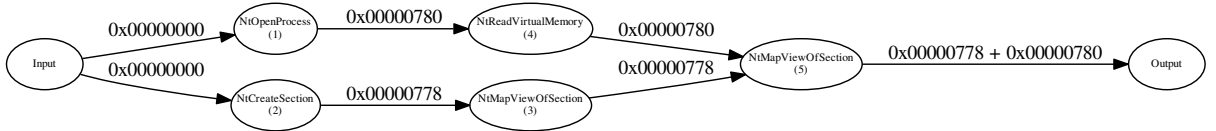
Figure 5.7: Code injecting string diagram
