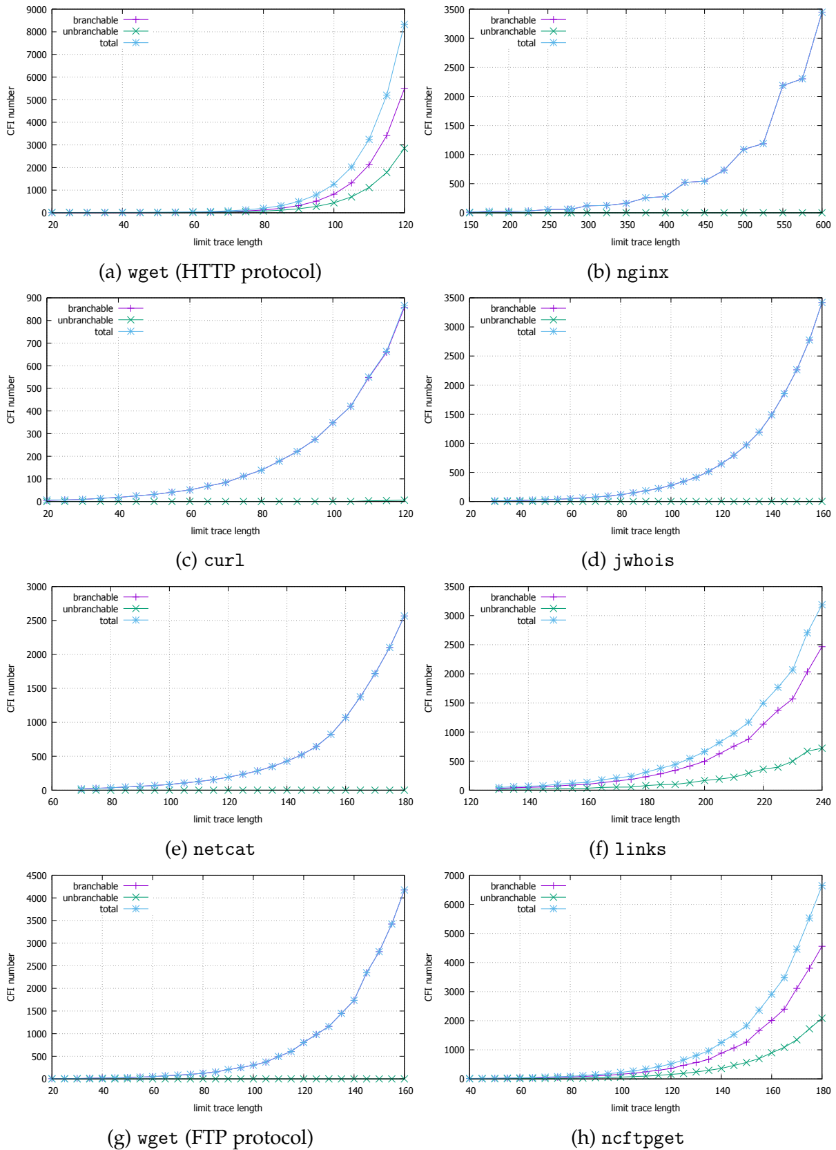
Figure 4.13: Exponential growth of CFI(s) in execution trees
