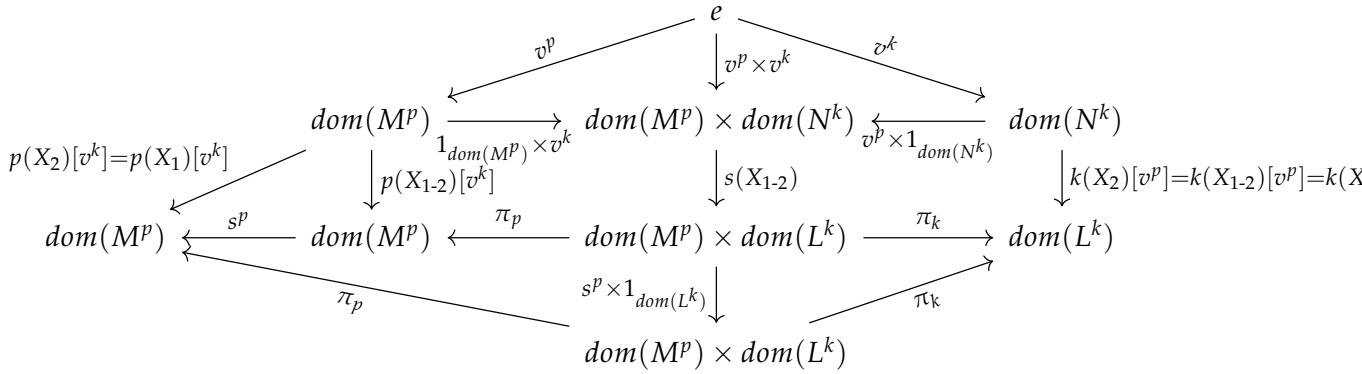
Figure 5.2: Obfuscated path construction
