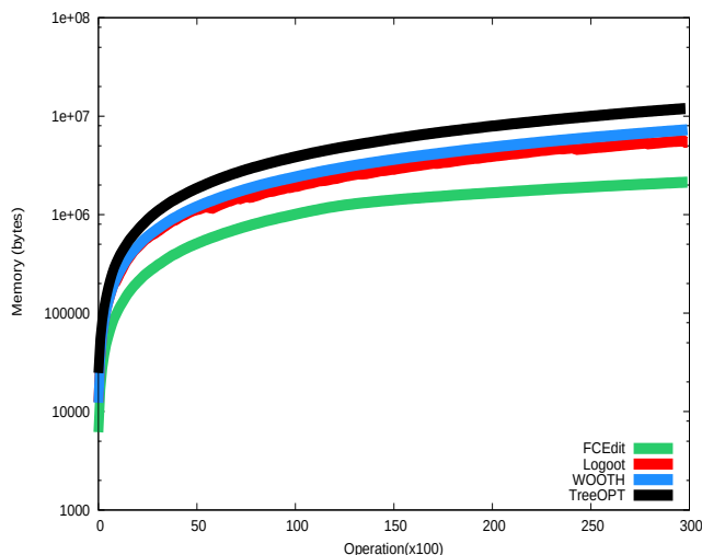
FIGURE 4.19 – L’occupation mémoire.
