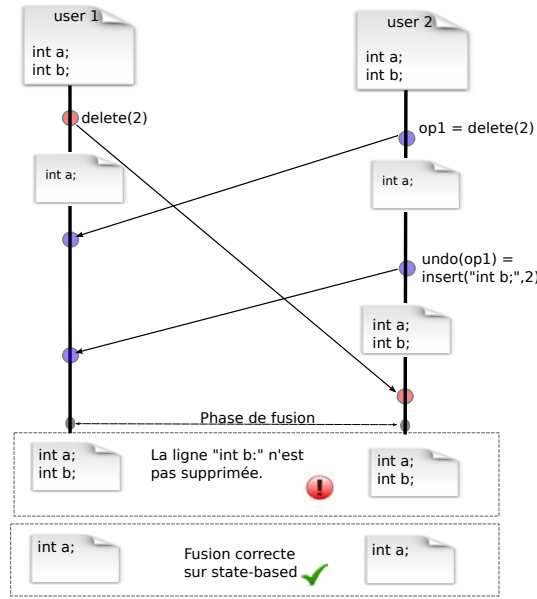
FIGURE 5.5 – opération undo/redo
