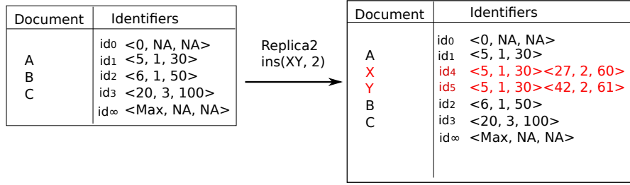
FIGURE 2.16 – Document Logoot.
