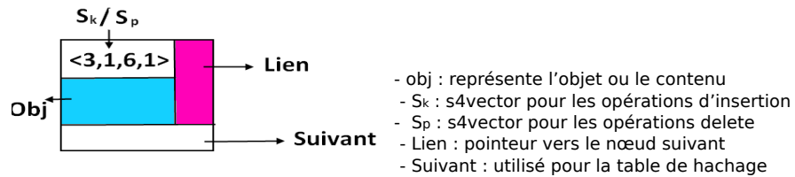
FIGURE 2.13 – S4vector
