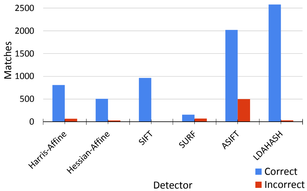
Figure 3-11: Rotation example for the painting dataset, views 0 – 2 (top). In the chart (bottom), correct matches are illustrated in blue, wrong matches in red
