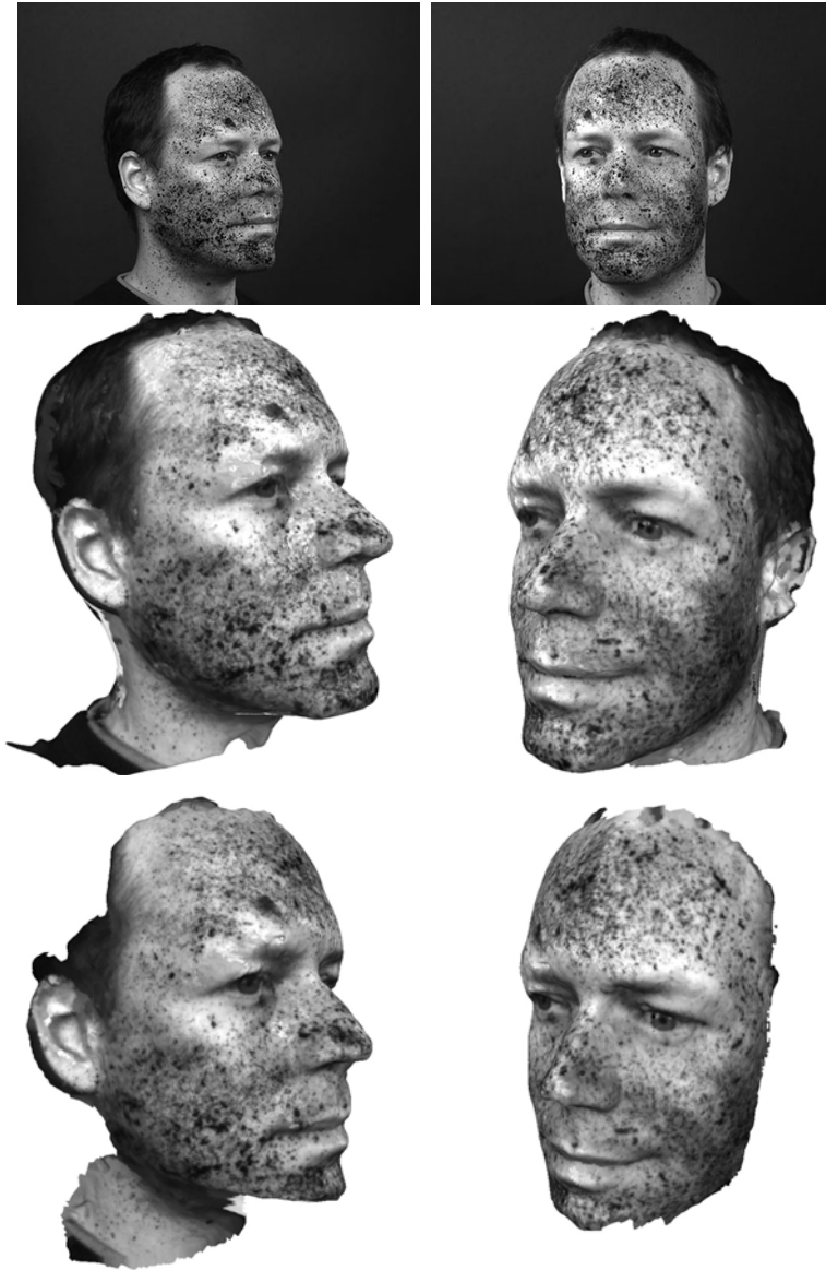
Figure 5-12: Two images from face2 dataset- 6 \times 1.3 MP- (top) reconstructed using our approach (middle) and using variational matching code provided by the authors of [18].
