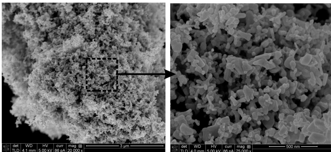
Figure 1.5. SEM photograph of the commercial ZnO nanoparticles (VP AdNano ZnO 20DW, Degussa Co.) used in this thesis. The different morphologies include rods, tetrapods with both pyramidal and round tips.
