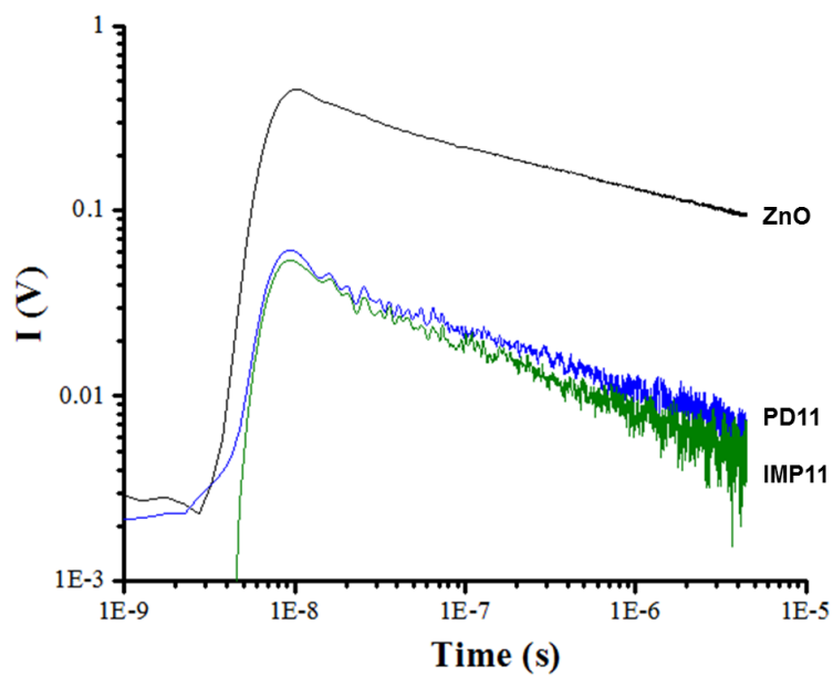
Figure 3.9. TRMC signals after excitation at 435 nm of pure ZnO and Ag/ZnO.
