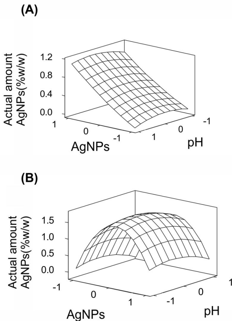
Figure 6.5. 3D surface plot of the effect of actual amount AgNPs and pH on the response of the RSM model of the functionalization of ZnO by the (A) photodeposition and (B) impregnation method.
