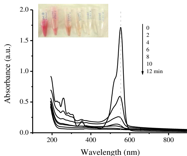
Figure 2.C. Evolution of the UV-Vis spectra of rhodamine-B degradation using Ag/ZnO-PD11 photocatalyst under UV light (test conditions: rhodamine-B =47 mg/L, photocatalyst= 1 g/L, \lambda =254 nm). Photograph of rhodamine-B discoloration in function of time.
