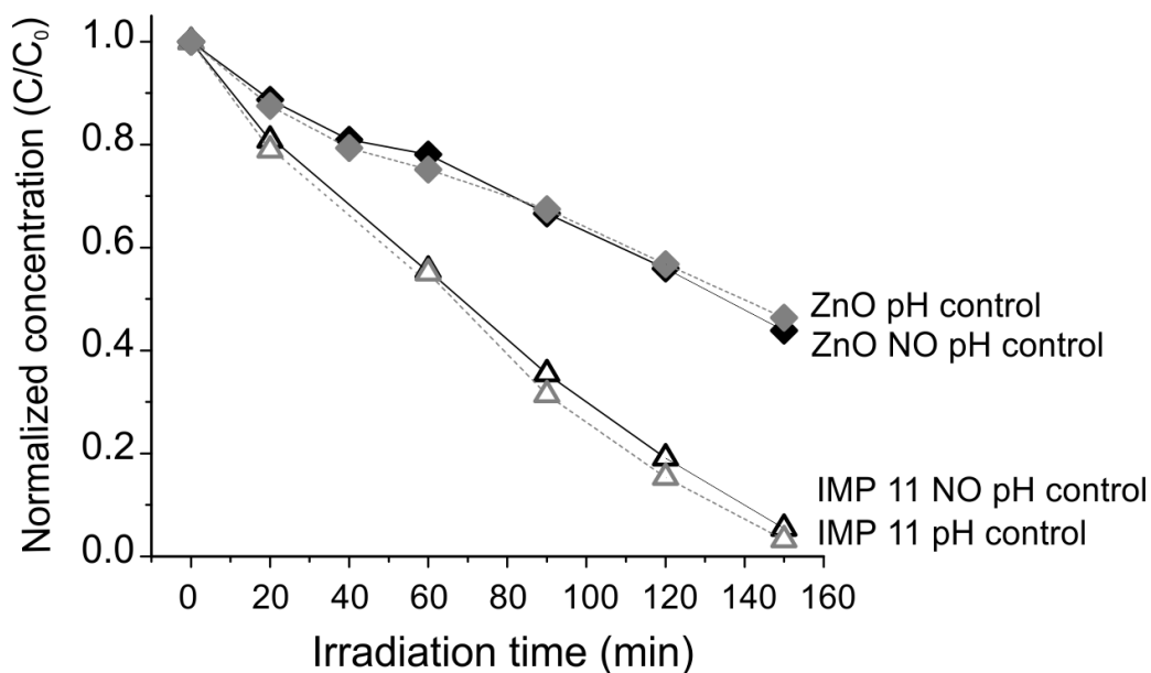
Figure 5.7. Normalized concentration of bisphenol-A at different conditions of pH control using pure ZnO and Ag/ZnO-IMP11 photocatalysts (test conditions: BPA=10 mg/L, photocatalyst= 1 g/L, \lambda =302 nm, pH=10.5).
