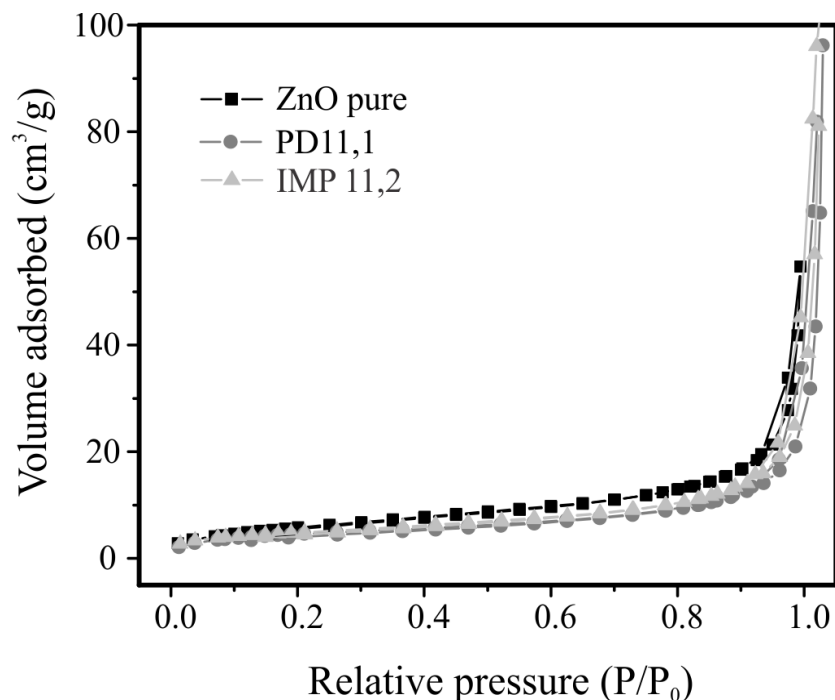
Figure 3.5. N_2 adsorption-desorption isotherm of 1% w/w Ag/ZnO photocatalyst prepared by the photodeposition (PD) and impregnation (IMP) method.
