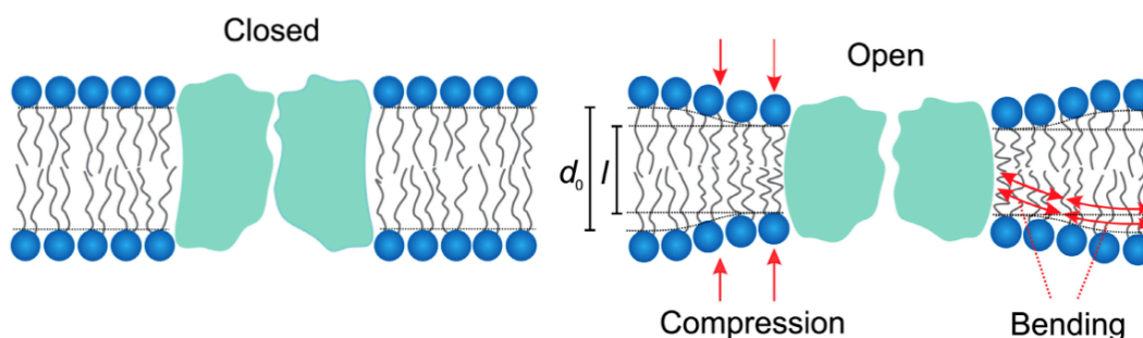
Figure 2.3.2.1. The so-called hydrophobic coupling between a bilayer-spanning membrane protein (ion channel) and its lipid bilayer host. A protein conformational change causes a local bilayer deformation (right). This deformation incurs an energetic cost that should be taken into account when estimating the free energy of an ion channel transition from the closed state (left) to the open one (right). The figure is adapted from [177].
