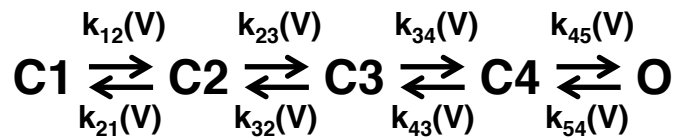
Figure 2.2.4.1. Kinetic model describing the Shaker 's gating [69]. The states from C1 to C4 correspond to different conformation of the voltage sensor (resting and several intermediate) and the closed pore. The O state relates to the activated/open channel. k_{xy}(V) is a kinetic constant, which depends on the applied voltage V .
