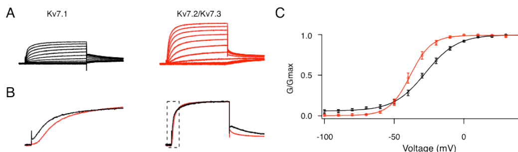
Figure 4.3.5.4. Comparing properties of the Kv7.1 (black) and Kv7.2/Kv7.3 (red) channels. A. Currents elicited by a family of depolarizing pulses. B. Time-courses of current onset; left shows expanded view of dashed boxed region. C. The G/V curves.
