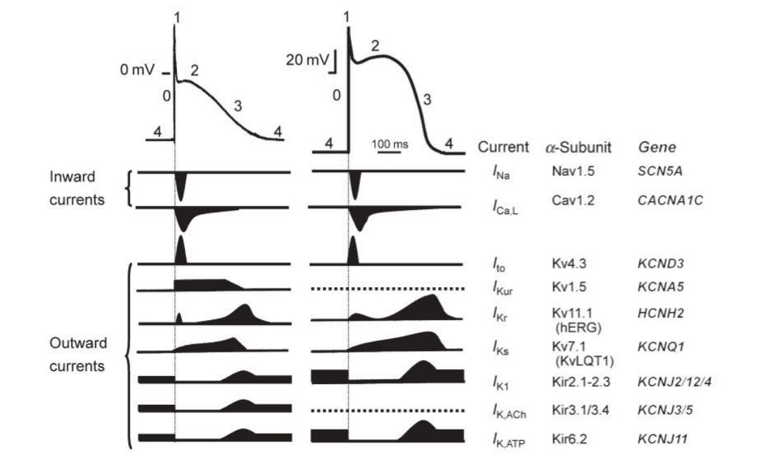
Figure 2.2.1.2. Cardiac action potential: atrial (top left panel) and ventricular (top right panel). The three other panels specify the current name, the ion channel responsible for it and the gene, encoding the ion channel, respectively. The figure is adapted from [65].
