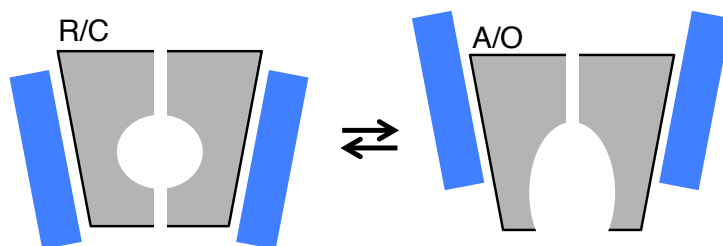
Figure 2.2.3.2. The two most populated conformational states of a voltage-gated ion channel with strong coupling between the pore domain and the voltage sensors: resting/closed (R/C) and activated/open (A/O).
