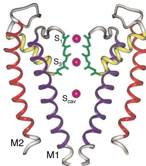
Figure 2.1.7.1. The crystal structure of the bacterial pH-dependent potassium channel KcsA. The extracellular side is at the top and the intracellular side is at the bottom. The main structural elements are the outer helix M2 (in red), the pore helix (in yellow), the selectivity filter (in green) and the inner helix M1 (in purple). Three potassium ions located at the outer and inner sites of the selectivity filter (S 1 and S 3 ) and at the center of the aqueous cavity (S cav ) are shown in magenta. The figure is adapted from [57].
