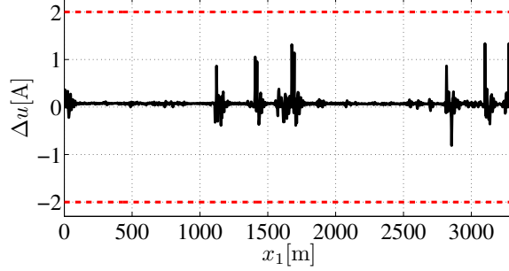
Figure 5.36: Control law \Delta u(k) of the explicit algorithm. Red dashed lines: \Delta u_{\min}(k) and \Delta u_{\max}(k) . Solid black line: control law \Delta u(k) .
