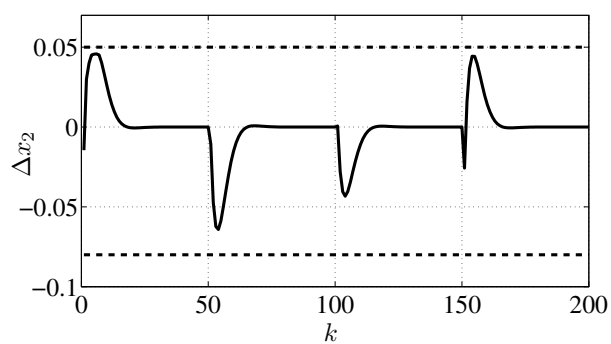
Figure 3.9: Tracking error \Delta x_2(k) . Solid line: tracking error \Delta x_2(k) . Dashed line: time-invariant constraints X_\Delta for \Delta x_2(k) .
