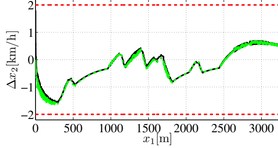
Figure 5.12: Closed-loop tracking error \Delta x_2(k) with a mass variation of 20%. Red dashed lines: \Delta x_{2min}(k) and \Delta x_{2max}(k) . Solid black line: tracking error \Delta x_2(k) of the on-line solution of the problem (5.16) at each execution time. Green dashed line: tracking error \Delta x_2(k) of the Algorithm 3.
