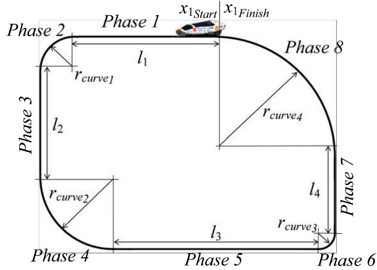
Figure 2.6: Example of a track with straight lines and curves. l_i[\text{m}] is the length of the i -th straight line and r_{curve_j}[\text{m}] is the radius of the j -th curve.
