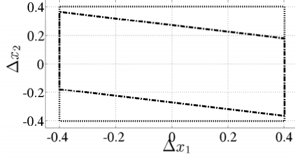
Figure 4.4: Constraints for k < 30 . Dotted line: constraint X_{\Delta}(k) . Dash-dotted line: constraint \mathcal{X}_{\Delta}(k) .
