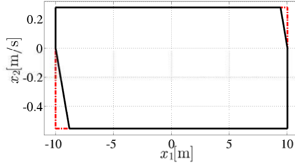
Figure 3.12: Maximal invariant set. Red dash-dotted line: closed-loop constraints \mathcal{X}_\Delta . Solid line: final invariant set \Omega .
