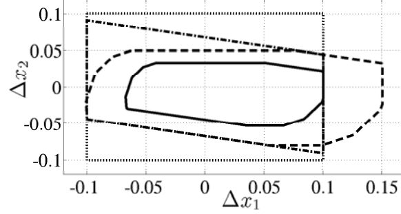
Figure 4.7: Homothetic transformation for 30 \leq k < 90 or k \geq 140 . Dotted line: constraint X_\Delta(k) . Dash-dotted line: constraint \mathcal{X}_\Delta(k) . Dashed line: nominal invariant set \hat{\Omega} . Solid line: \alpha(k)\hat{\Omega} with \alpha(k) = 0.67 .
