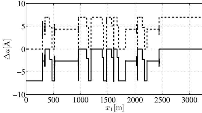
Figure 4.16: Time-varying tracking constraints U_\Delta(k) with respect to the vehicle's position. Solid line: \Delta u_{min}(k) . Dashed line: \Delta u_{max}(k) .
