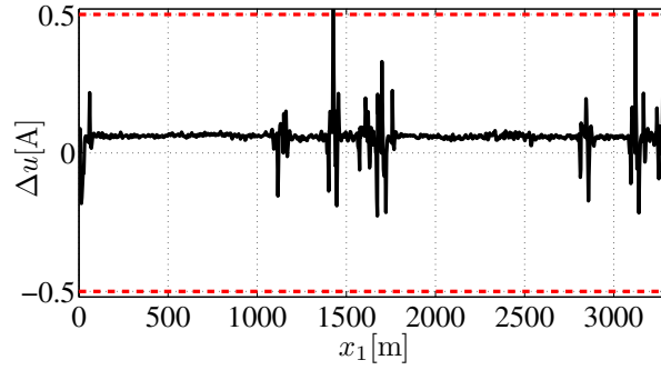
Figure 5.31: Control law \Delta u(k) of the explicit algorithm. Red dashed lines: \Delta u_{min}(k) and \Delta u_{max}(k) . Solid black line: control law \Delta u(k) .
