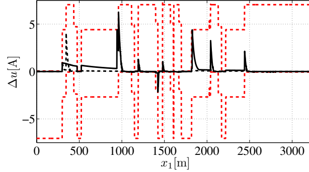
Figure 4.22: Closed-loop tracking error \Delta u(k) . Red dashed lines: \Delta u_{min}(k) and \Delta u_{max}(k) . Dashed line: tracking input \Delta u(k) of the nonlinear system with a mass variation of 10%. Solid line: tracking input \Delta u(k) of the nonlinear system with a mass variation of 50%.
