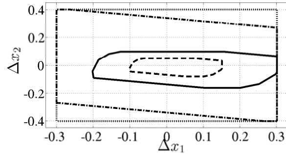
Figure 4.9: Homothetic transformation for 90 \leq k < 140 . Dotted line: constraint X_\Delta(k) . Dash-dotted line: constraint \mathcal{X}_\Delta(k) . Dashed line: nominal invariant set \hat{\Omega} . Solid line \alpha(k)\hat{\Omega} with \alpha(k) = 2 .
