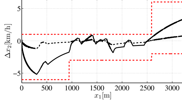
Figure 4.21: Closed-loop tracking error \Delta x_2(k) . Red dashed lines: \Delta x_{2min}(k) and \Delta x_{2max}(k) . Dashed line: tracking error \Delta x_2(k) of the nonlinear system with a mass variation of 10%. Solid line: tracking error \Delta x_2(k) of the nonlinear system with a mass variation of 50%.
