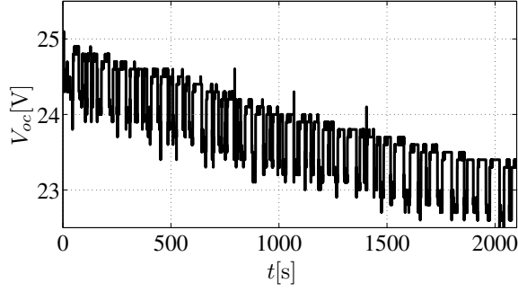
Figure 6.9: Open circuit voltage of the battery V_{oc} . The total variation in the voltage of the battery V_{oc} during all the race, corresponds to a variation of 4.16% of the voltage of the battery fully charged.
