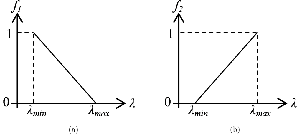
Figure 2.10: Functions of the vertices of the polytopic LPV representation. (a) f_1(\lambda(k)) . (b) f_2(\lambda(k)) .
