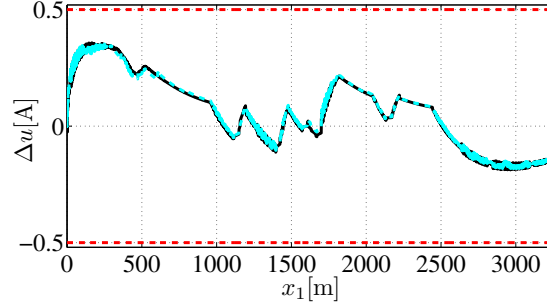
Figure 5.25: Closed-loop tracking error \Delta u(k) with a mass variation of 20%. Red dashed lines: \Delta u_{min}(k) and \Delta u_{max}(k) . Solid black line: tracking input \Delta u(k) of the on-line solution of the problem (5.45) at each execution time. Cyan dashed line: tracking input \Delta u(k) of Algorithm 4.
