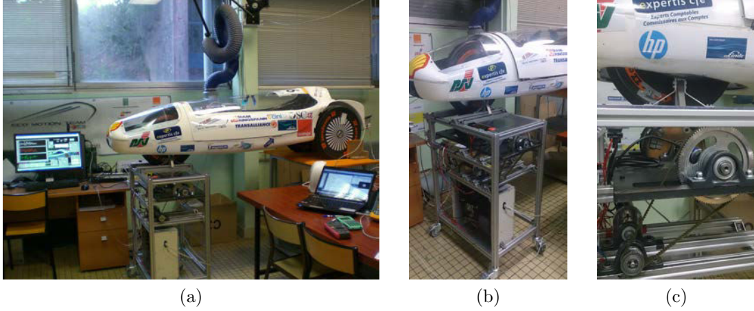
Figure 2.12: Benchmark in the year 2014. (a) Vir'Volt vehicle and benchmark. (b) Detail of the Benchmark. (c) Inertial cylinder and electric motor.
