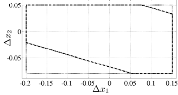
Figure 3.4: Polytopic constraints. Dashed line: constraints X_{\Delta} . Dash-dotted line: constraints \mathcal{X}_{\Delta} .
