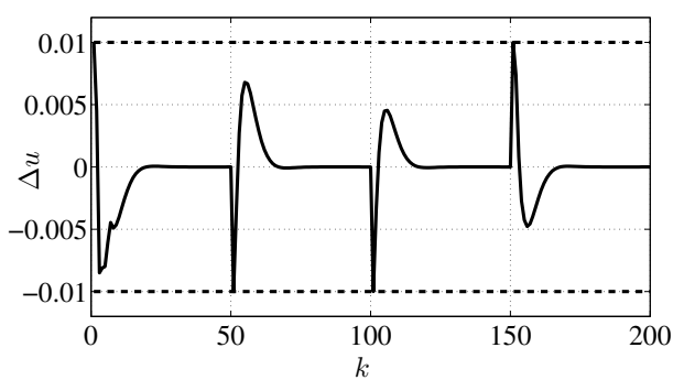
Figure 3.10: Tracking error \Delta u(k) . Solid line: tracking error \Delta u(k) . Dashed line: time-invariant constraints U_\Delta .
