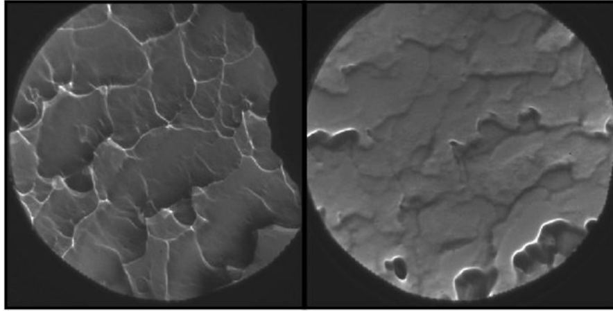
FIGURE 4.21: Contrast from flat features on SG1 (InPd polycrystal) are shown in two different imaging modes. Both images were taken at a 50 \mu\text{m} FOV.
