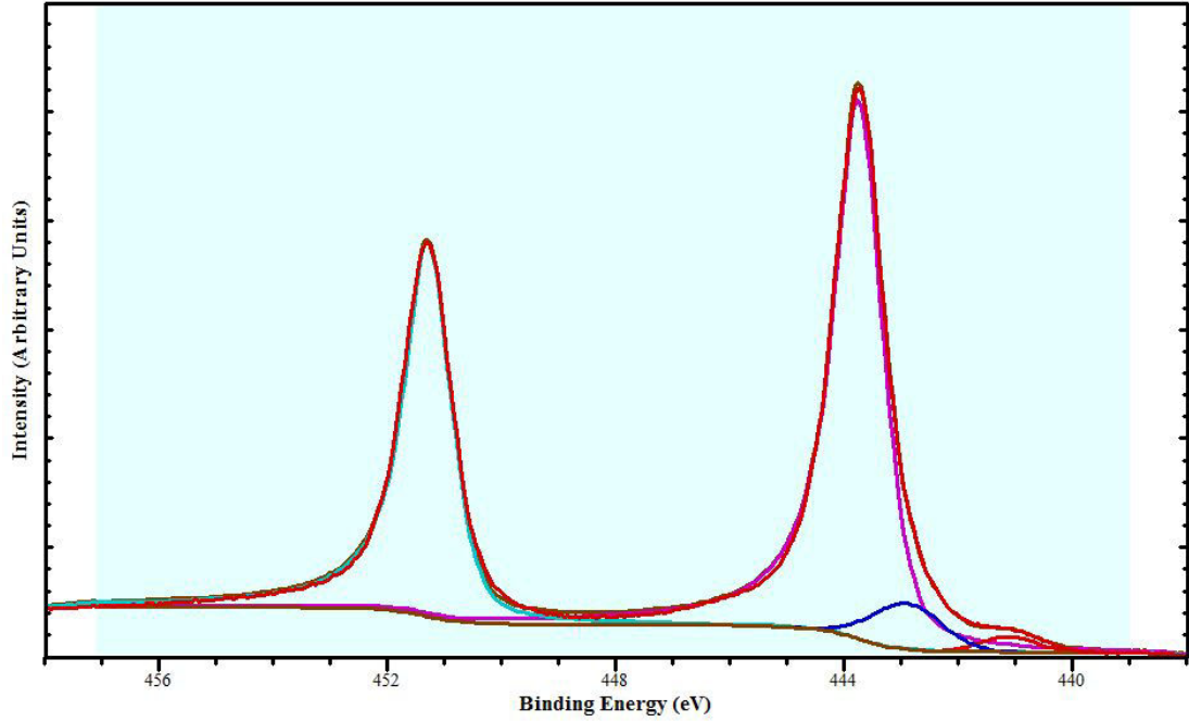
FIGURE 2.5: The selected (blue/gray) region within the In 3d spectrum above, defines the endpoints for removal of a Shirley background. Within this region are two Doniach-Sunjić (In 3d_{3/2} /In 3d_{5/2} , large left/right peaks) and two Gaussian (In 3d_{3/2} K_{\alpha 3} / K_{\alpha 4} , small left/right peaks) peaks.
