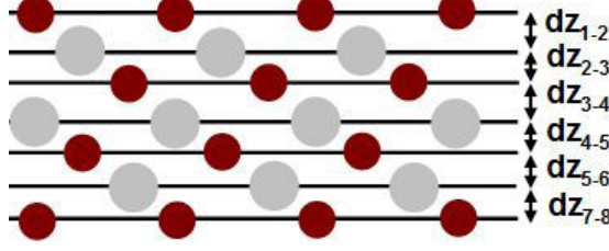
FIGURE 4.19: The above profile of the Pd-rich InPd(111)-(1x1) surface, viewed along the [\bar{1} 0 1] axis, illustrates interlayer spacings in accordance with values of Table 4.2. The expansions/-contractions of planes are slightly exaggerated for clarity.
