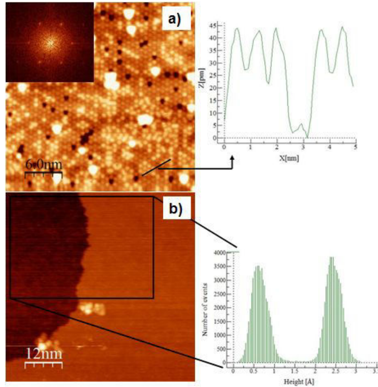
FIGURE 4.17: The above STM images correspond to InPd(111)- (\sqrt{3} \times \sqrt{3})R30^\circ (a) and InPd(111)- (1 \times 1) phases (b). The (\sqrt{3} \times \sqrt{3})R30^\circ phase includes a 1D plot to show the difference between the two main types of contrast. An FFT of the 30 nm x 30 nm image (+1.8 V; 0.09 nA) confirms the hexagonal superstructure defined as a (\sqrt{3} \times \sqrt{3})R30^\circ surface reconstruction. Image (b) (62 nm x 62 nm/+0.5 V; 0.07 nA) shows the step edge between two large terraces.
