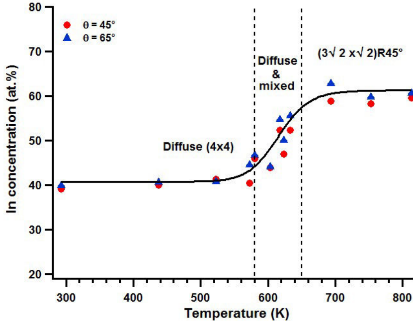
FIGURE 4.5: Concentration measurements after Ar + sputtering (2 keV for 30 minutes) and annealing the InPd(100) surface are deduced from XPS data for two different take-off angles ( \theta is the angle between the surface normal and analyzer). The solid line in this figure is a guide for the eye only.
