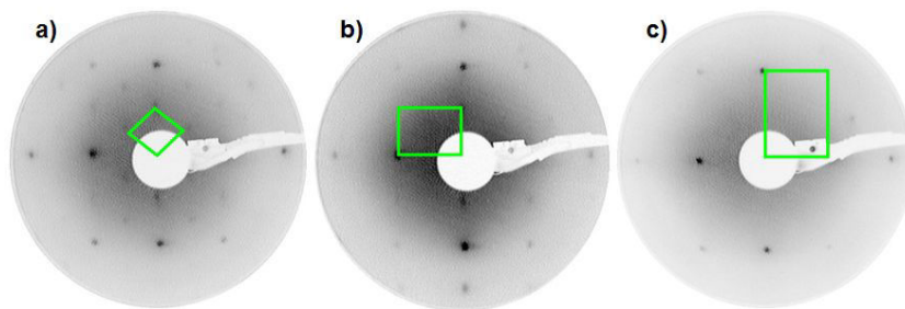
FIGURE 4.12: The above c(4x2) (a), (2x1) (b), and (1x1) (c) LEED patterns are the three reconstructions of the InPd(110) surface. The primitive reciprocal space unit cells for each image, taken at the same beam energy of 63 eV, are shown.
