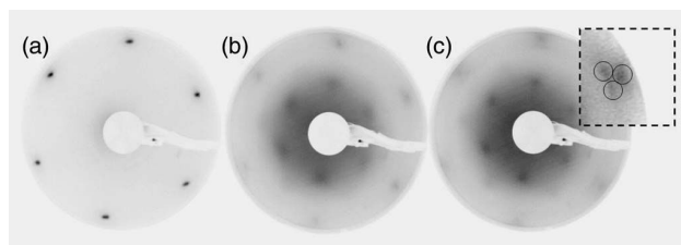
FIG. 2. LEED patterns of (a) the clean Pd(111) surface and after dosing (b) 1 MLE and (c) 2 MLE of In at room temperature. All patterns were recorded at an incident beam energy of 55 eV. The dotted rectangle in (c) is a blow-up of one of the outermost diffraction spots showing that they are actually poorly defined triplets.
