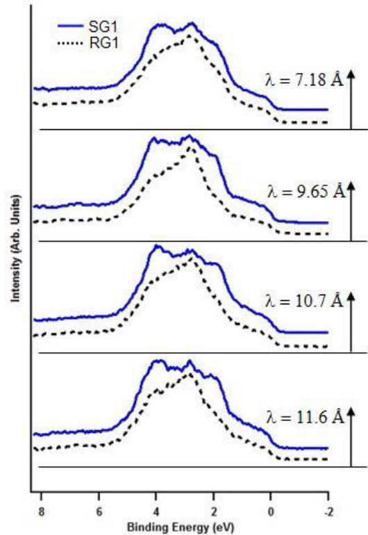
FIGURE 4.25: The VB data from SG1 and RG1 (InPd polycrystal) are displayed such that the top spectra is more surface sensitive whereas the bottom spectra is more bulk-like. The IMFPs displayed next to the graph were approximated using the kinetic energy within the dispersion plane corresponding to the stop voltages, from top to bottom: 245.5 eV, 445.5 eV, 543.5 eV, and 643.5 eV.
