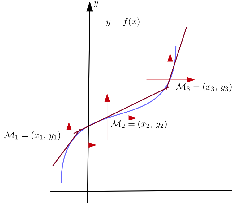
Figure 2.1 – Local approximation
