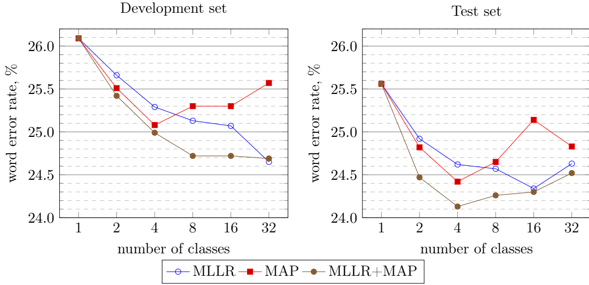
FIGURE 4.1 – Comparing MLLR, MAP and MLLR+MAP for adapting class-based models with KL-based classes. Use 190 hours of training data and 4500 senones
