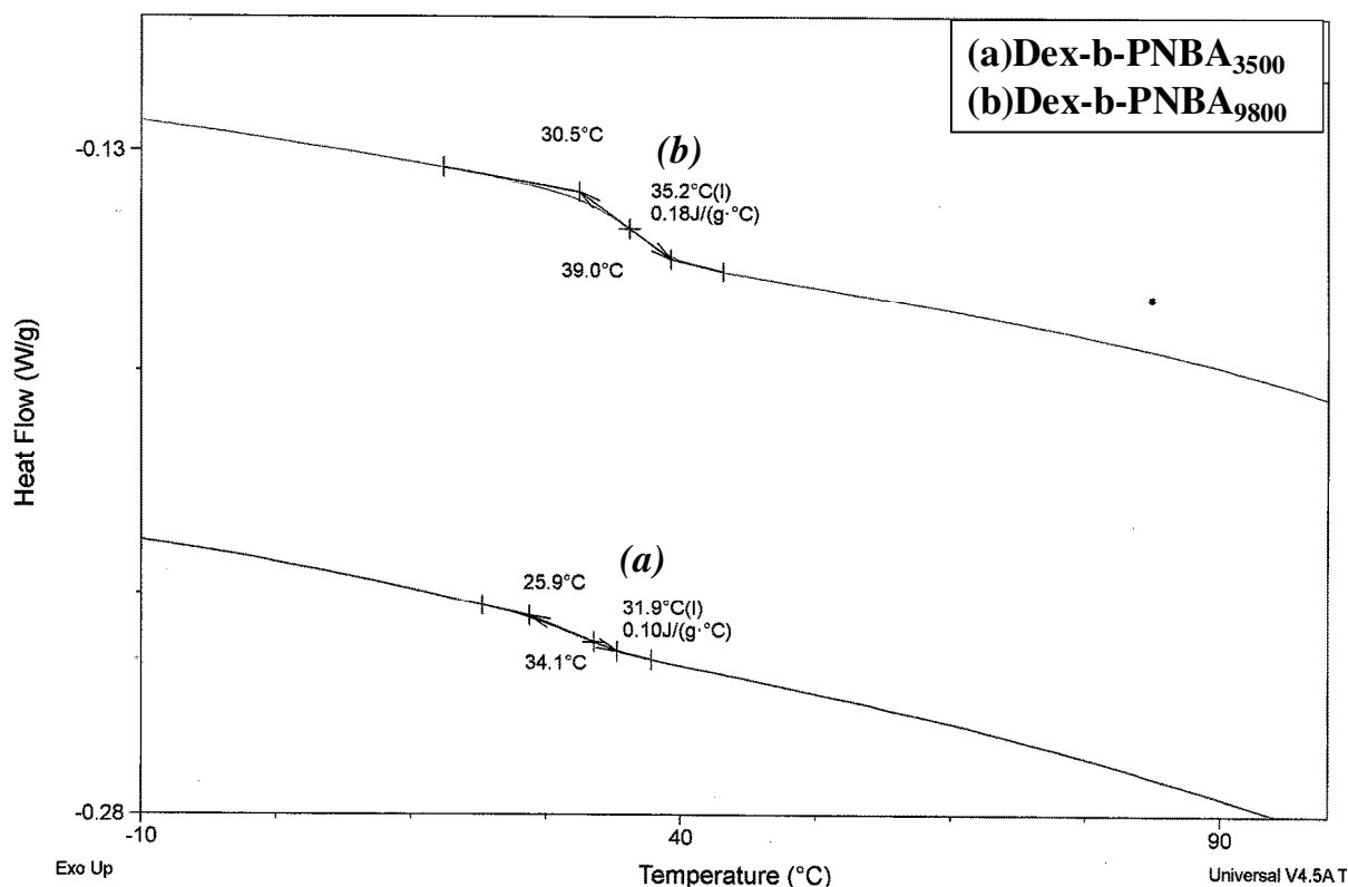
Figure 20. Thermograms MDSC of diblock glycopolymers Dex-b-PNBA 3500 ( F_{\text{PNBA}} = 27\% ) and Dex-b-PNBA 9800 ( F_{\text{PNBA}} = 49\% )
