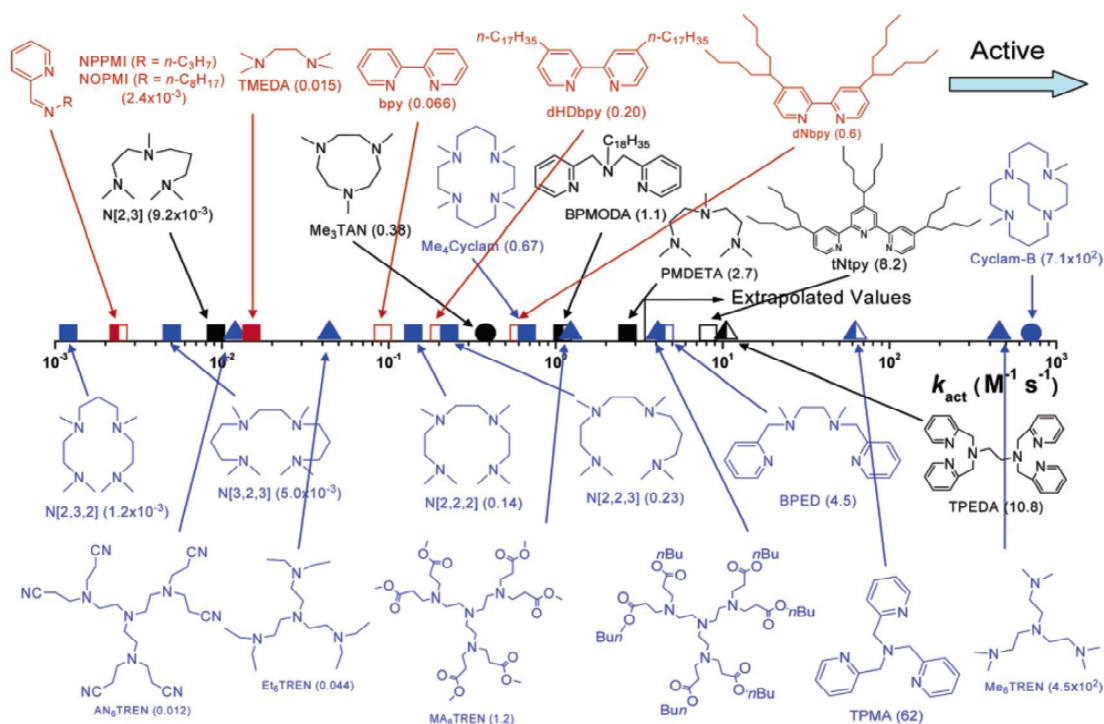
Figure 46. ATRP activation rate constants for various ligands with EtBriB as initiator in the presence of \text{Cu}^{\text{I}}\text{Y} ( \text{Y} = \text{Br} or \text{Cl} ) in MeCN at 35^\circ\text{C} : N2, red; N3, black; N4, blue; amine/imine, solid; pyridine, open. Mixed, left-half solid; linear \square branched \blacktriangle ; cyclic, \bigcirc [143].
