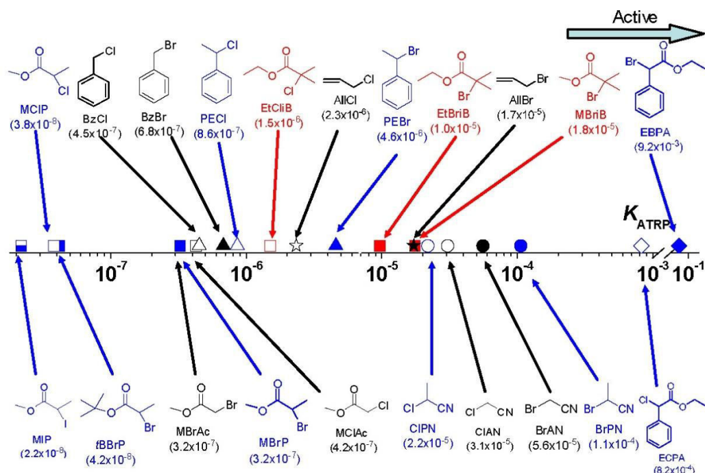
Figure 47. ATRP equilibrium constants for various initiators with \text{Cu}^{\text{I}}\text{X}/\text{TPMA} ( \text{X} = \text{Br} or \text{Cl} ) in \text{MeCN} at 22^\circ\text{C} [144].
