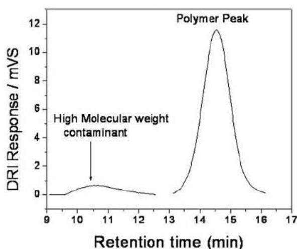
Figure 57. DRI chromatogram of SET-LRP of MA using EtBrIB in DMSO without CuBr 2 [208].
