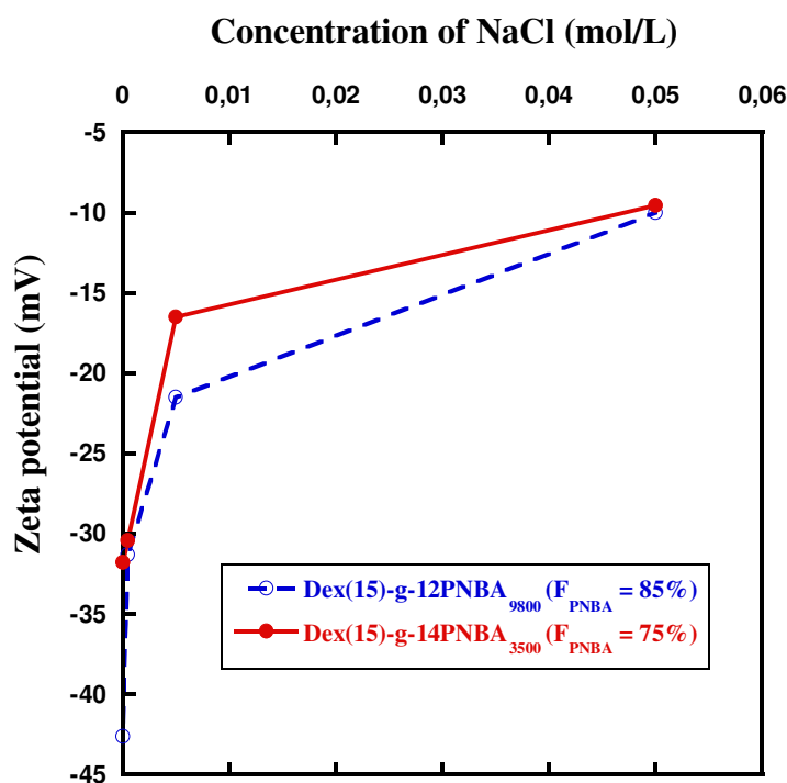
Figure 73. Evolution of zeta potential for nanoparticles made on Dex-g-PNBA ( F_{\text{PNBA}} = 75 and 85\% ) against concentration of NaCl.
