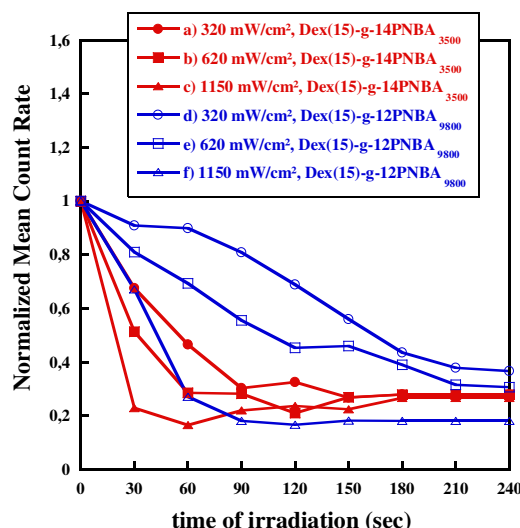
Figure 90. Normalized Mean Count Rate against time of irradiation using different UV-lamp power. Solid symbols Dex(15)-g-14PNBA 3500 ( F_{\text{PNBA}} = 75\% ) and open symbols Dex(15)-g-12PNBA 9800 ( F_{\text{PNBA}} = 85\% )
