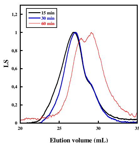
Figure 63. SEC trace (LS detector, eluent THF, 40°C). ATRP in methanol at 40°C, with NBA/ EBiB/ HMTETA/CuBr: 100/ 1/ 1/ 1.
