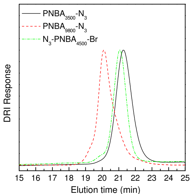
Figure 4. SEC chromatograms in THF of \text{PNBA}_{3500}\text{-N}_3 , \text{PNBA}_{9800}\text{-N}_3 and \text{N}_3\text{-PNBA}_{4500}\text{-Br} (Differential Refractive Index Response).
