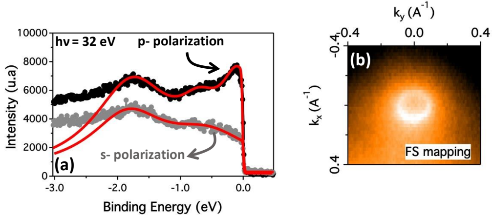
Figure 27: (a) EDCs measured in normal emission for the MgO-covered SGA ( T=4\text{K} and h\nu=32\text{eV} ) with a p-polarized (black circle) and s-polarized (open circle) beam. (b) in-plane cut of the Fermi surface extracted from ARPES measurements.
