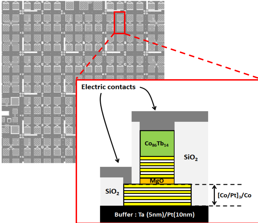
Figure 1: Sketch of the Magnetic Tunnel Junction with the bottom and top [\text{Co/Pt}]_3/\text{Co} electrodes.
