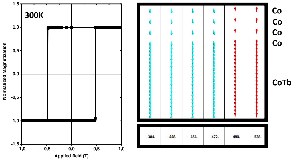
Figure 6: Left: Calculated M(H) loop for the \text{CoTb}/[\text{Co/Pt}]_3/\text{Co} multilayer with 1.42 nm thick Pt layers. Right: magnetic configurations calculated for different applied fields in mT.
