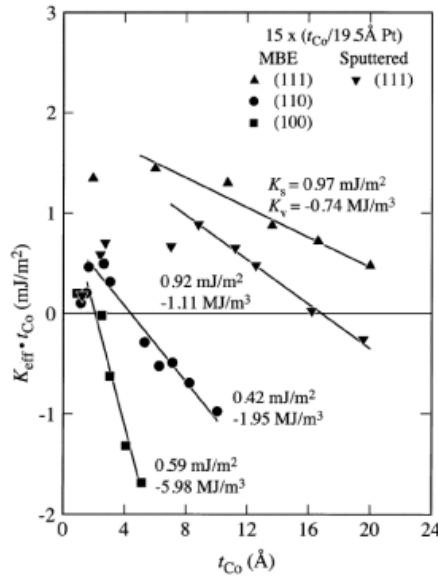
Figure 4: Dependence of the volume ( K_V ) and surface ( K_S ) anisotropy contributions in epitaxial and sputtered [Co/Pt] multilayers for different crystallographic orientations.
