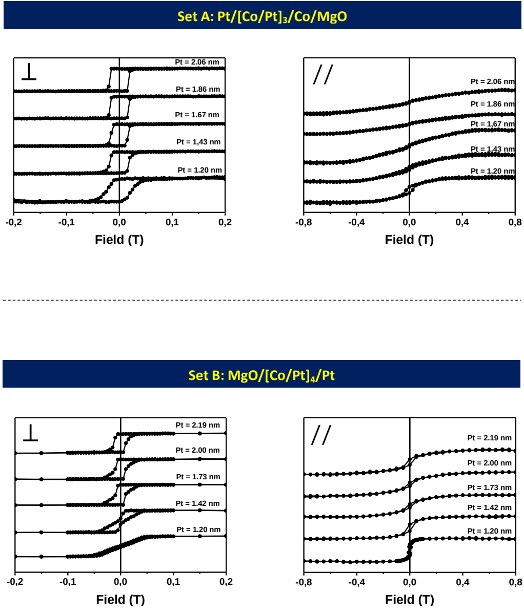
Figure 11: M(H) loops for the out-of-plane (left) and in-plane (right) configurations measured at room temperature for the sets A (top) and B (bottom). The reported Pt thicknesses are the fitted ones.
