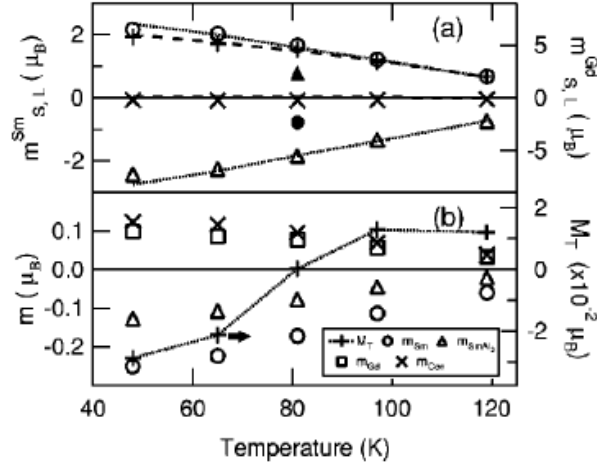
Figure 6: (a) Experimental values of m_S^{\text{Sm}} (○), m_S^{\text{Gd}} (+), m_L^{\text{Sm}} (Δ) and m_L^{\text{Gd}} (x) when the sample was magnetized at 110K (open symbols) and at 43K (filled symbols). The dashed and dotted lines correspond to the theoretical value of the 4f spin and orbital moments of Gd and Sm (respectively). (b) Net magnetization (+) for the Sm (○), Gd (□) and conduction electrons (x) compared to the net magnetization of \text{SmAl}_2 (Δ) (from [12]).
