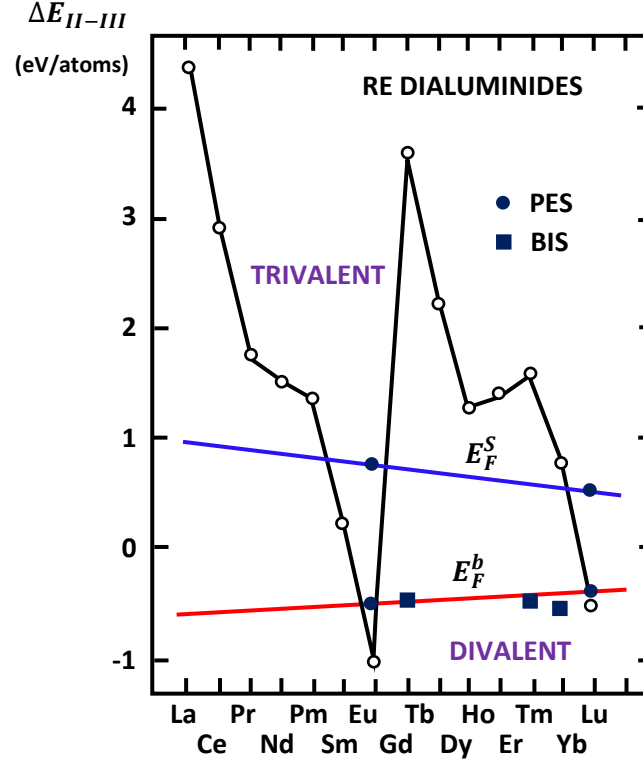
Figure 2: Stability diagram of the divalent and trivalent configurations for the RE dialuminide compounds extracted from PES (blue circles) and BIS (blue squares) experiments. The horizontal lines correspond to the relative position of the Fermi level in the bulk E_F^b (red line) and at the surface (blue line) [14] .
