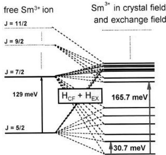
Figure 1: Sketch of the energy levels for free \text{Sm}^{3+} (Left) and for \text{Sm}^{3+} ion in \text{SmCo}_5 (right), where one can see the effects of crystal and exchange fields: lift of degeneracy and mixing of multiplets (from [4] ).
