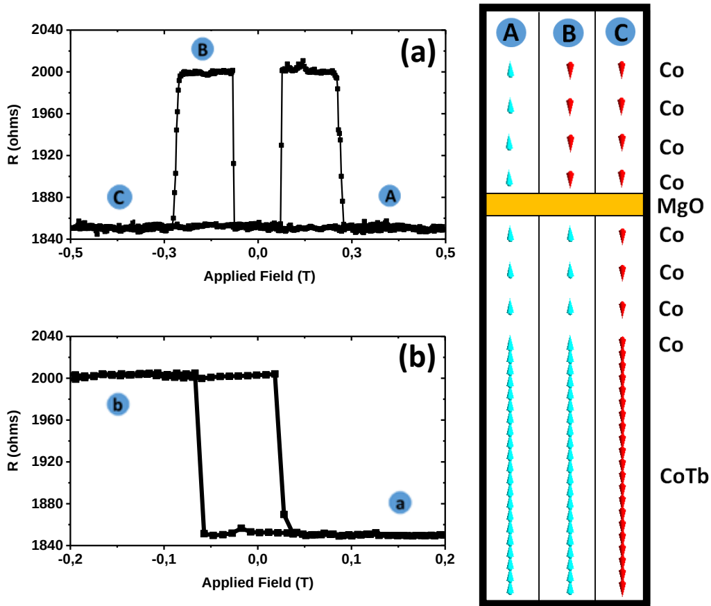
Figure 16: Left: R(H) characteristics measured at room temperature for a reversed field H_{rev} of (a) -0.5 T and (b) -0.2 T. Right: magnetic configurations of the soft and hard electrodes: ④ parallel state, ⑤ reversal of the soft electrode (anti-parallel state), ⑥ back to a parallel state with the reversal of the hard electrode.
