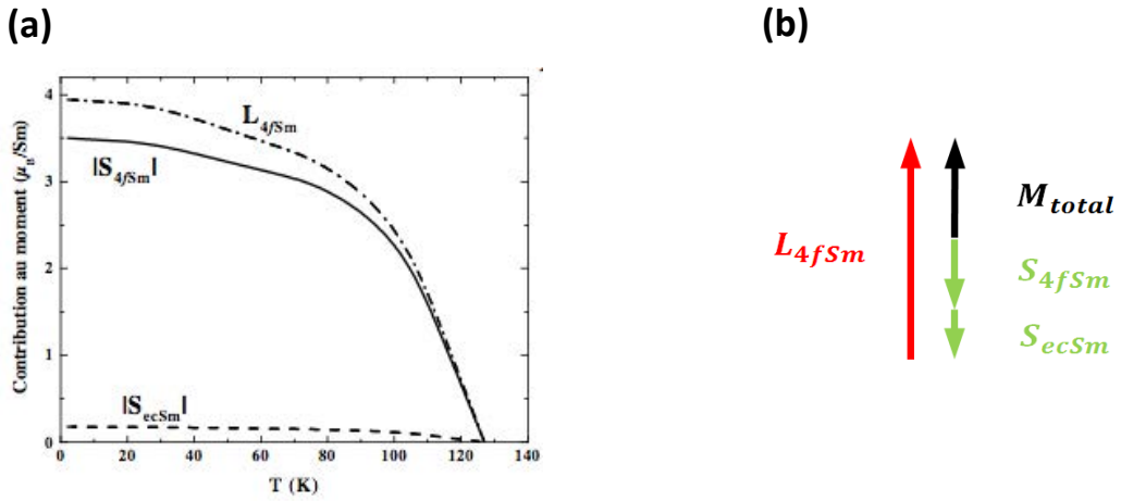
Figure 3: (a) Calculated temperature dependences of the Samarium 4f spin (black lines) and orbital (dash-dot) contributions and of the conduction electrons contribution (dash line) in \text{SmAl}_2 (b) Sketch of the different contributions to the total magnetic moment in \text{SmAl}_2 .
