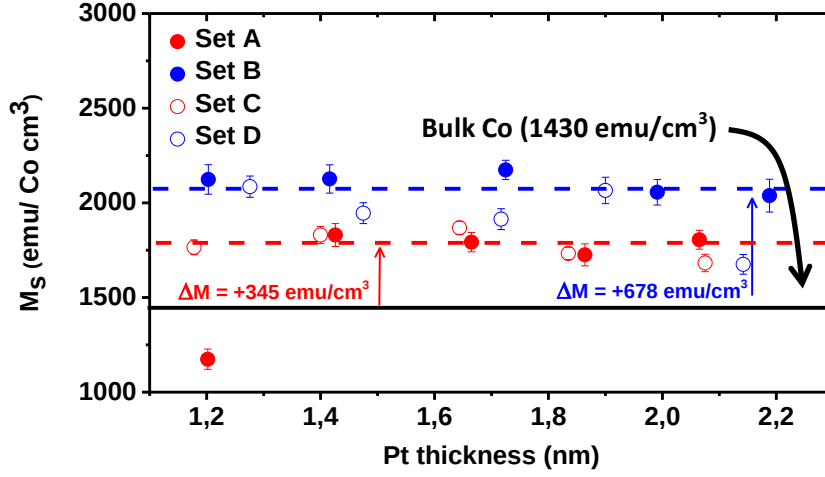
Figure 14: Magnetization versus the Pt thickness for the different sample sets. The black horizontal line corresponds to bulk Co (1430 emu/cm 3 ) and the dash lines are guides for the eyes.
