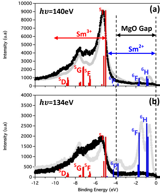
Figure 26: XPS spectra around the Samarium 4f contributions measured in normal emission with a photon energy of 140 eV (a) and 134 eV (b) for the MgO-covered (black symbols) and free (grey symbols) SGA surfaces. The emitted intensity for the free SGA surface has been normalized with respect to the 5 I peak intensity (divided by a factor 5 and 3 for the Sm 3+ and Sm 2+ resonance respectively). The colored bars denote the calculated weights and binding energies for the trivalent (red) and divalent (blue) Sm contributions [25] .
