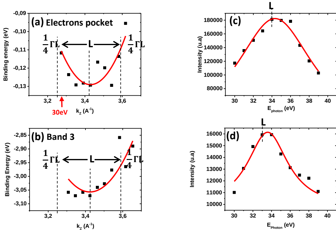
Figure 18: (a-b): Energy dispersion curves along the perpendicular [111] direction for the electrons pocket (top) and the band 3 (bottom) identified in figure 11 (a). The solid red curves are the parabolic fits using E = \hbar^2 k^2 / 2m^* + E_0 . The extracted effective mass m^* and E_0 are given in Table 3. (c-d): Intensity versus the photon energy for the same contributions. The solid red curves are Lorentzian fits.
