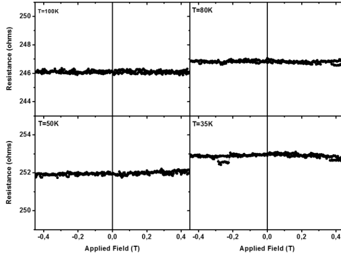
Figure 14: R(H) characteristics measured at 100K, 80K, 50K and 35K for SGA/MgO/ [\text{Co}_{0.58\text{nm}}/\text{Pt}_{1.8\text{nm}}]_4 MTJs ( 10\mu\text{m} \times 10\mu\text{m} )
