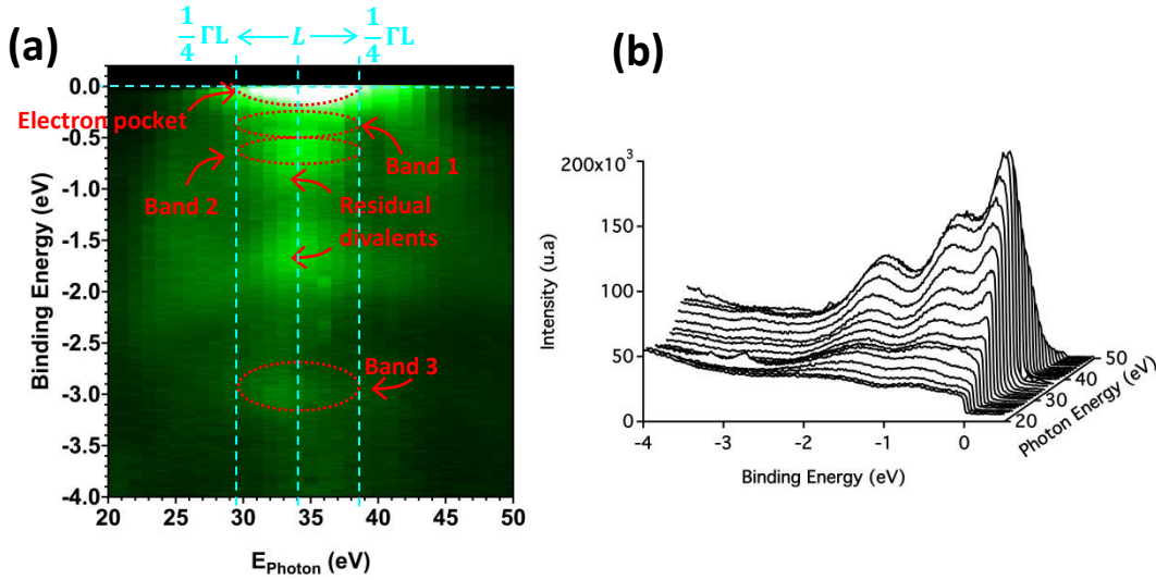
Figure 17: (a) : I(E_B, hv) map and (b) corresponding EDCs, measured in normal emission at 4K and for a p-polarized photon beam.
