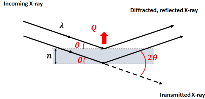
Figure 1: Sketches of the X-ray diffraction principles at large (a) and low (b) angles when incoming X-rays interact with the matter.
