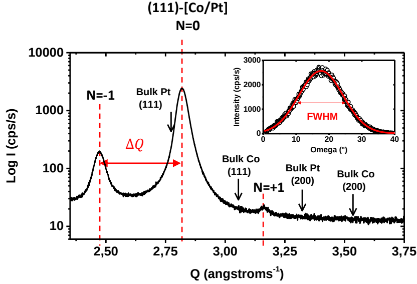
Figure 4: X-ray pattern collected at high angles for the “XRD sample”. The positions of the N = -1, 0 and +1 Bragg peaks for the periodic [\text{Co}_{0.97\text{nm}}/\text{Pt}_{0.5\text{nm}}]_{50} stacking are shown by the red vertical dash lines. Inset is the rocking curve measured across the (111)-[Co/Pt] multilayers Bragg peak (open circles) with a Gaussian adjustment (red line).
