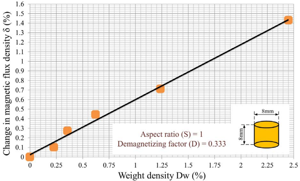
Figure 3.25 Estimating the changes in magnetic flux density with different weight densities.
