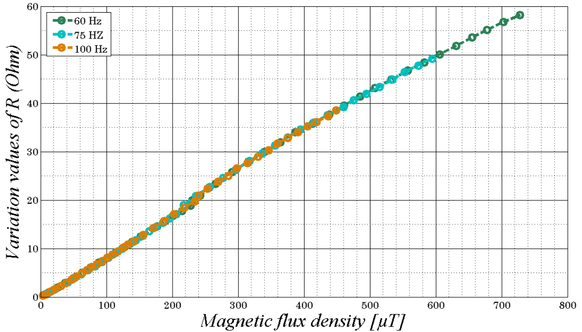
Figure 2.56 The variation ( \Delta R ) of the GMR elements according to the magnetic flux density ( B ) at different frequencies.
