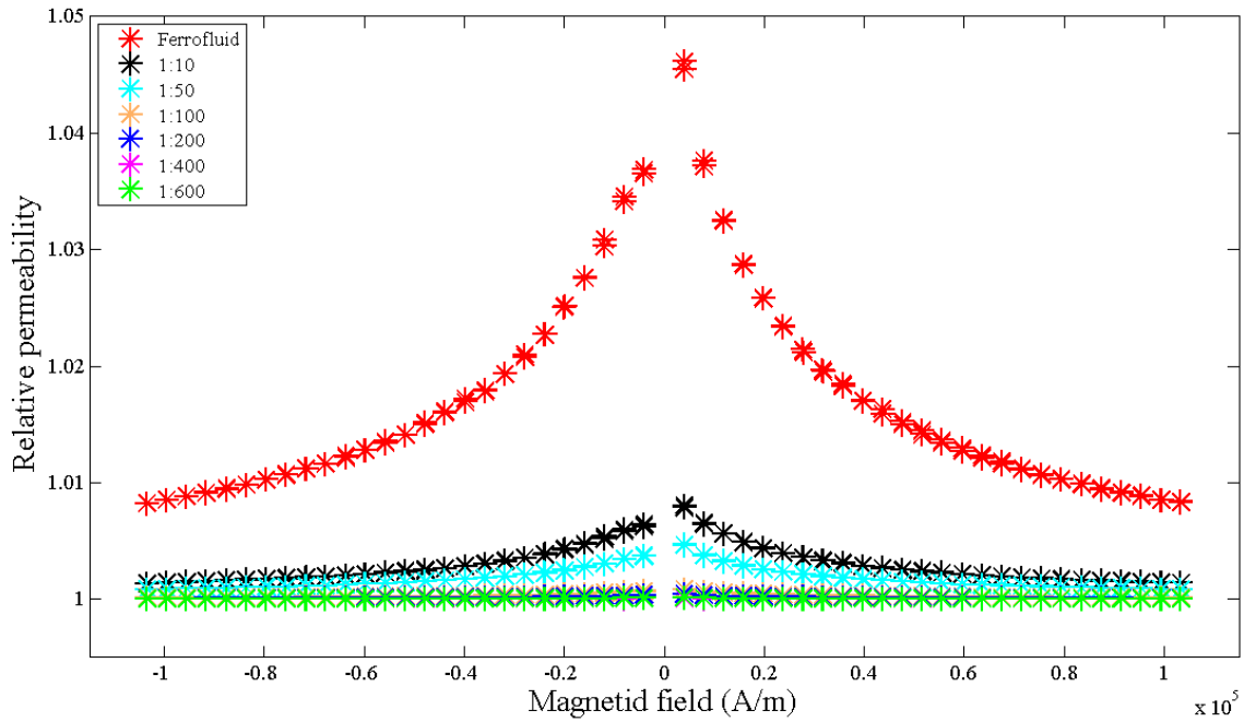
Figure 3.16 Relative permeability ( \mu_r ) as a function of an applied field (A/m).
