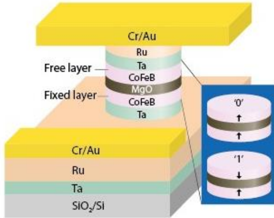
Figure 1.15 Structure representation of a magnetic tunnel junction (ferromagnetic layer fixed (CoFeB) and the other layer free to rotate in to each condition, low resistance ('0') or high resistance ('1'), MgO is a barrier layer [30].
