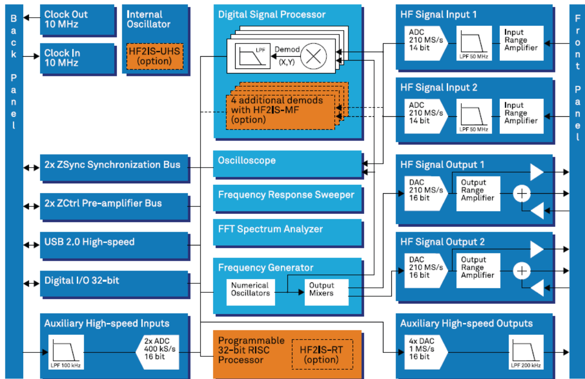
Schematic diagram of internal functioning of the HF2IS [71].
