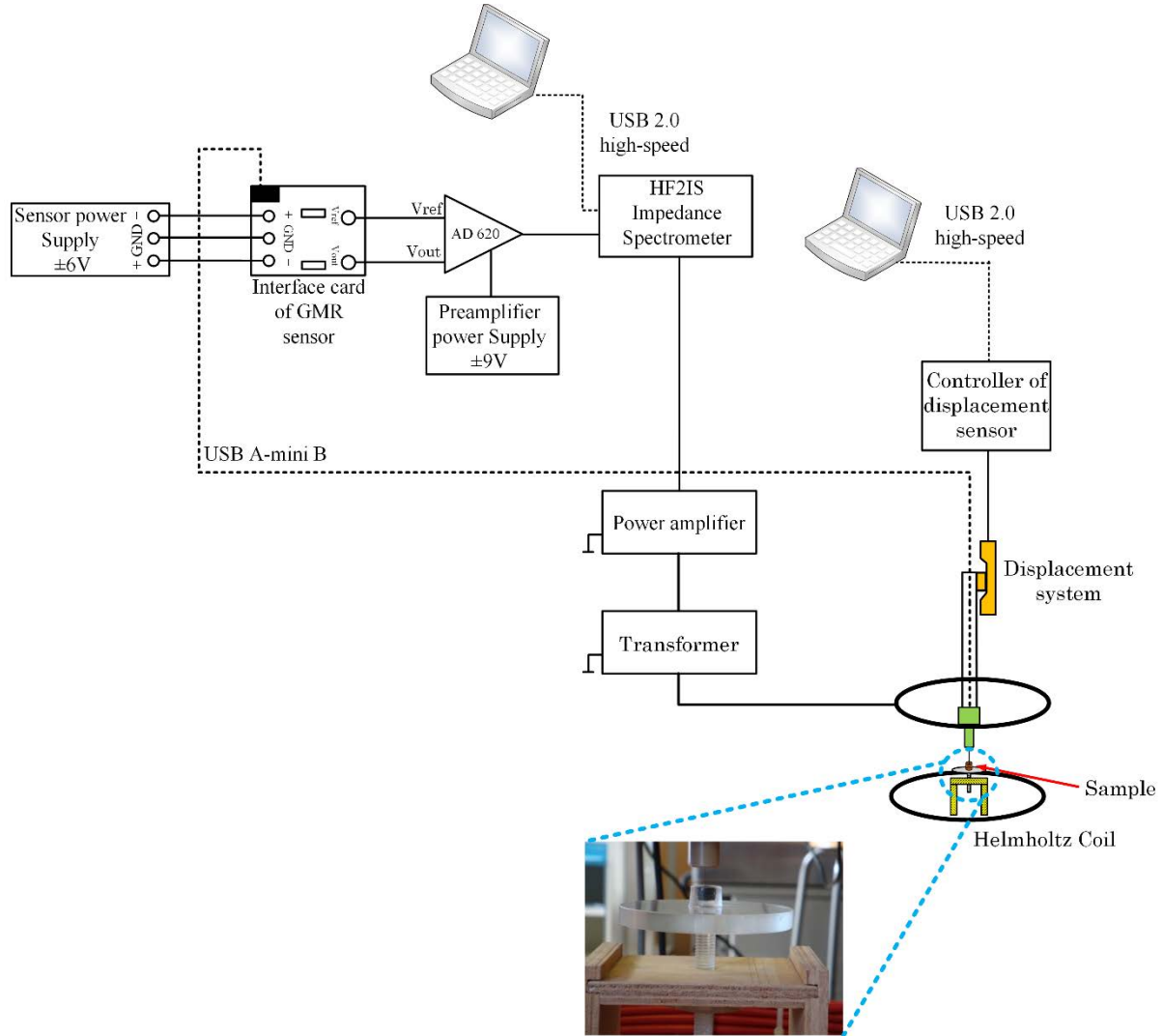
Figure 3.24 Schematic of measurement setup used to characterize the magnetic properties of ferrofluid MAG-D 200 nm.
