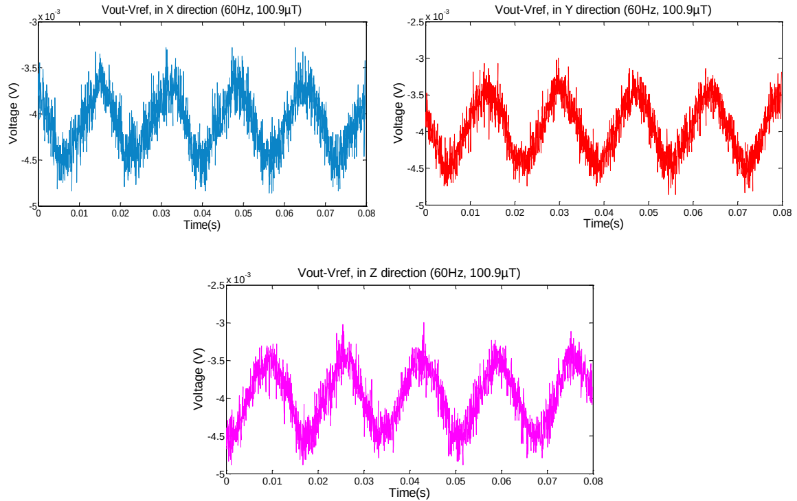
Figure 2.41 Output voltage ( V_{out}-V_{ref} ) signals of the GMR sensor in direction (X, Y, Z) at a frequency 60 Hz with B=100.9\ \mu T .
