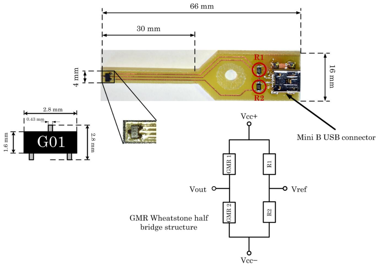
Figure 2.50 The design and components of the GMR sensor III.
