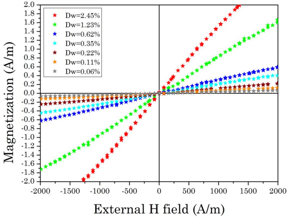
Figure 3.22 The hysteresis curves of fluid MAG-D's concentrations.
