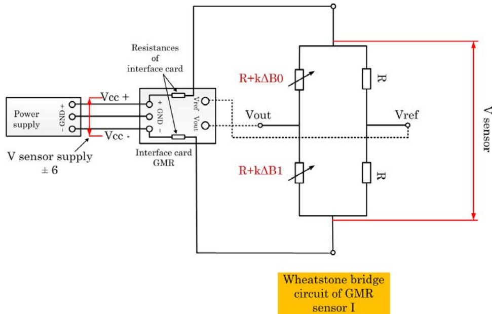
Figure 2.38 Electrical schematic and the Wheatstone bridge circuit of the GMR sensor I.
