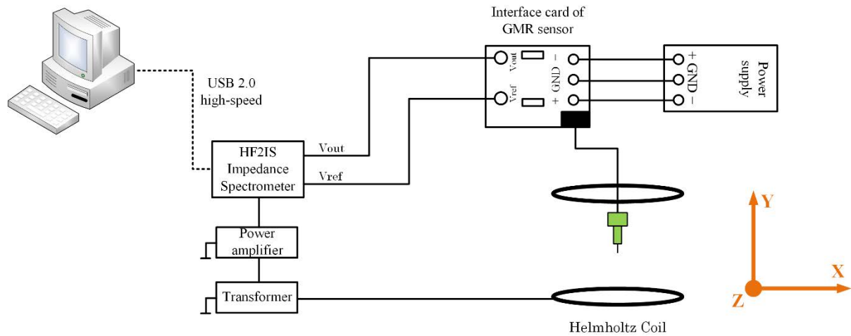
Figure 2.40 Measurement setup to characterize the GMR sensor.
