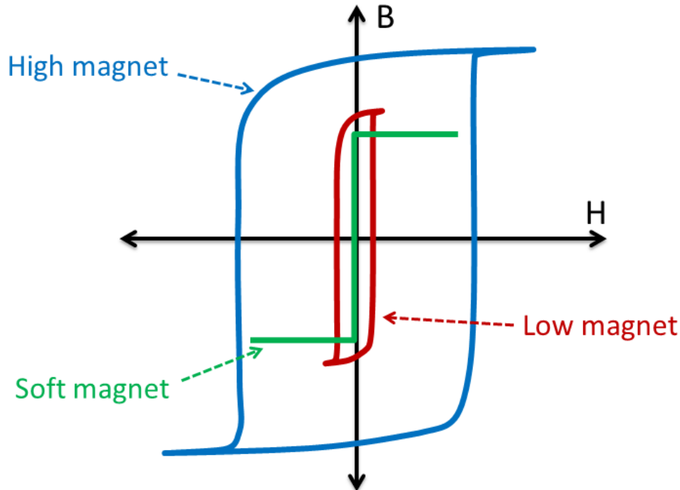
Figure 1.22 Typical Hysteresis curves for hard, low and soft magnetic materials.
