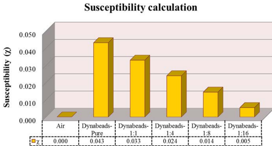
Figure 4.17 Relationship between susceptibility ( \chi ) and different magnetic fluid concentrations.
