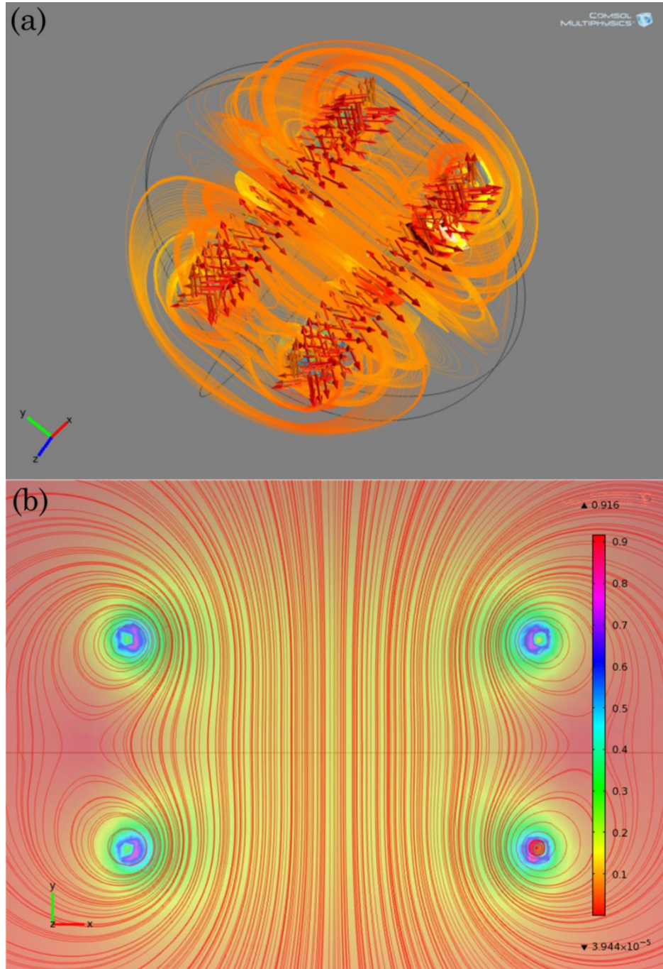
Figure 3.5 Magnetic flux density in total sphere of coils (a), distribution (B) at midpoint of the Helmholtz coil.
