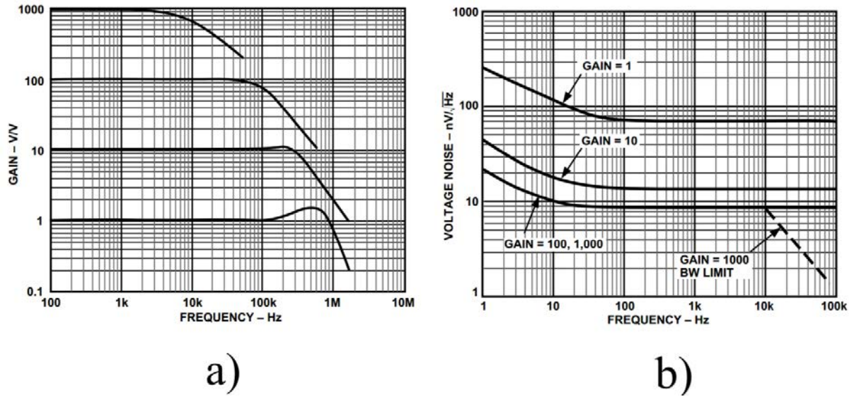
Figure 2.17 Typical characteristics of the Analog Device AD 620: Range of gain as a function of frequency (a); Voltage Noise Spectral Density depending on frequency for Gain = 1–1000 (b) [70].
