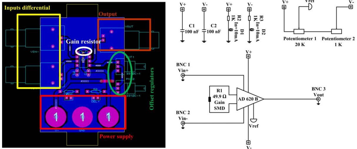
Figure 2.18 Design of preamplifier circuit.
