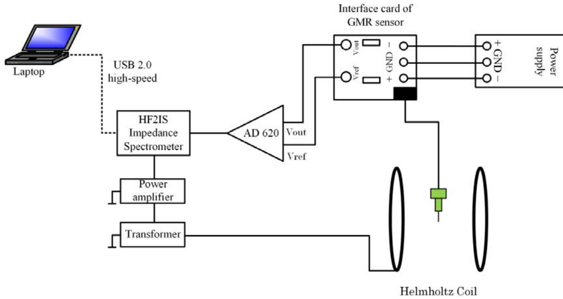
Figure 2.24 Measurement setup of the GMR sensor.
