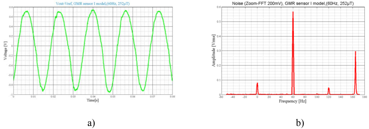
Figure 2.26 The output voltage ( V ) of first model (a) and the FFT detection from ( V_{out}-V_{ref} ) of the GMR sensor at 60 Hz (b).
