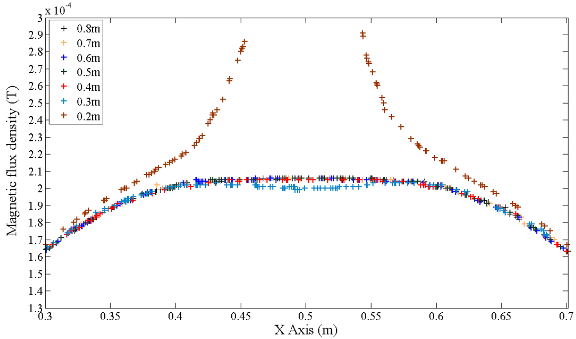
Figure 2.14 Changing the magnetic flux density ( B ) in center of the Helmholtz coil by changing the position of the displacement system along X axis.
