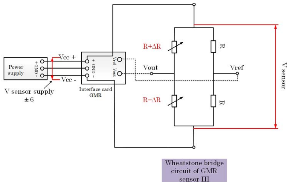
Figure 2.55 Electrical schematic and the Wheatstone bridge circuit of the GMR sensor model III.
