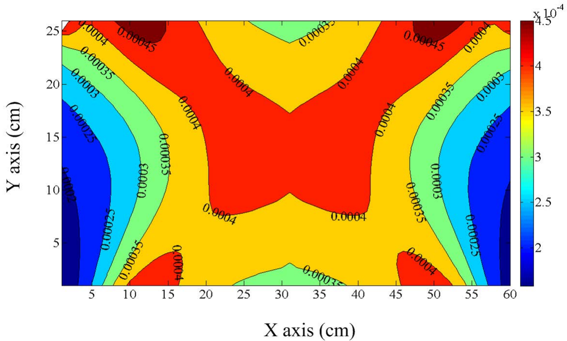
Figure 2.7 Analytical calculation the B distribution along the axes X and Y.
