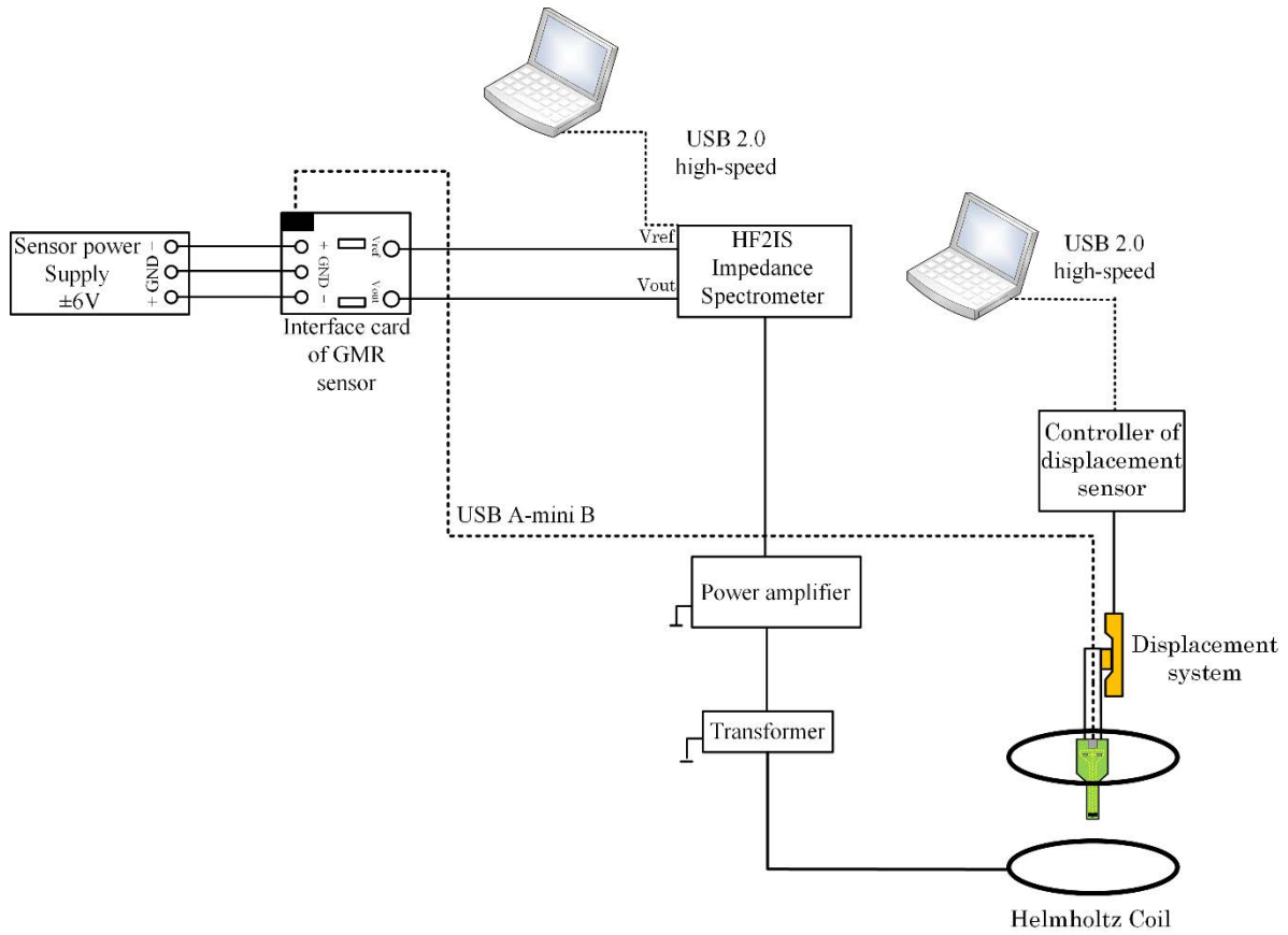
Figure 2.52 Measurement setup for characterize of the GMR sensor type III.
