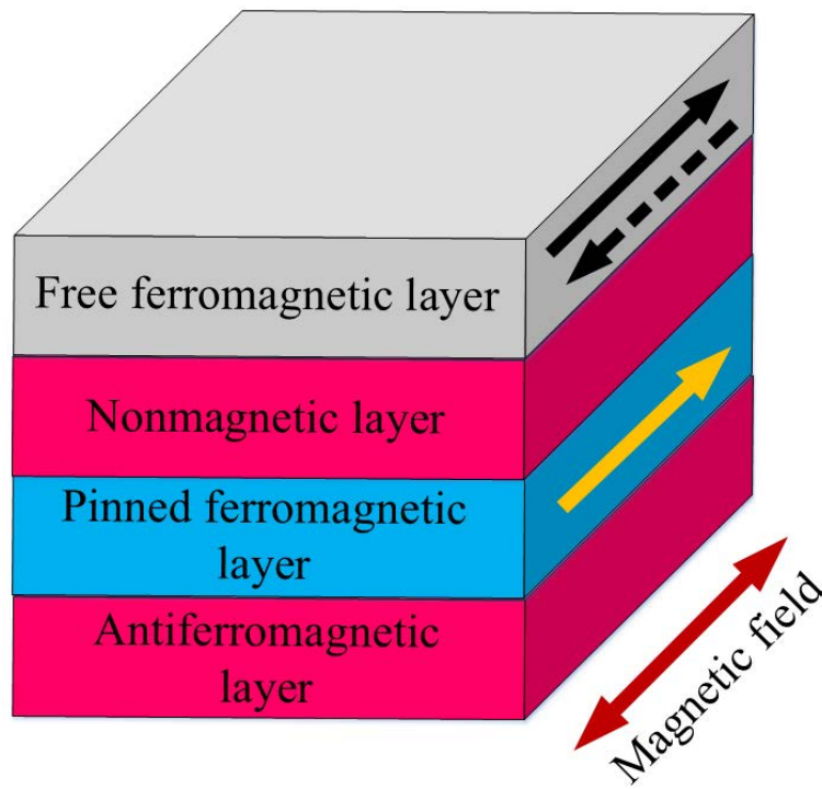
Figure 1.8 The structure of a spin-valve system.
