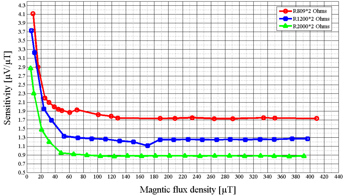
Figure 2.36 The relationship between sensitivity ( \mu\text{V}/\mu\text{T} ) and changes of the magnetic flux density ( \mu\text{T} ) by using several resistances in the interface card of the GMR sensor I.
