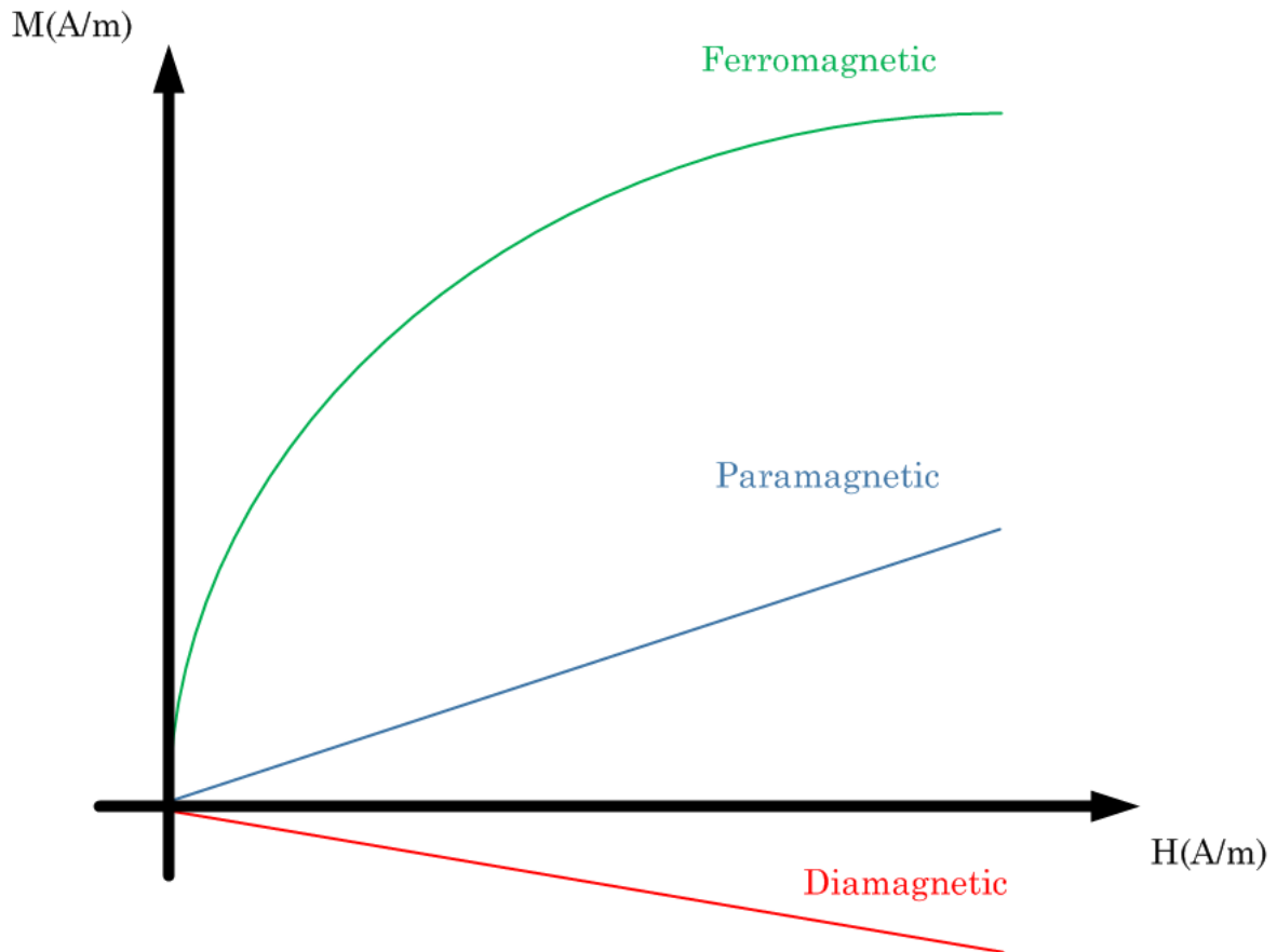
Figure 1.19 Comparison of magnetic behavior of the material.
