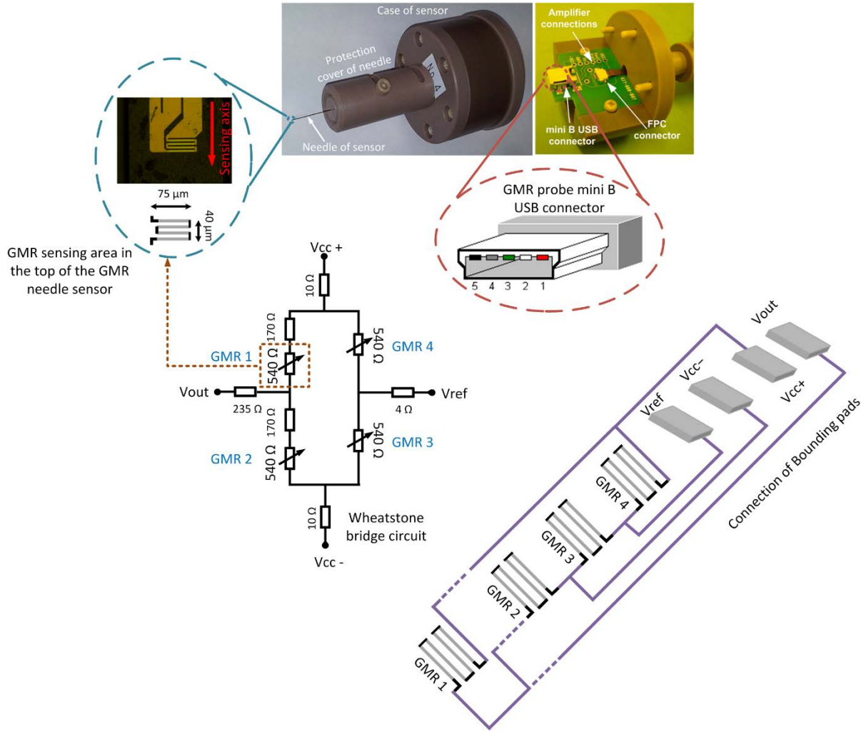
Figure 2.4 The design of the GMR needle probe and its components.
