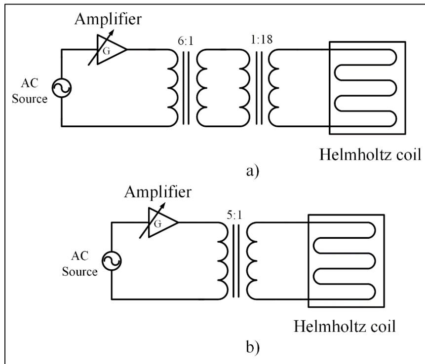
Figure 2.8 The power supplies schematic of the Helmholtz coil: 50/60 Hz (a) and 10/50 kHz (b).
