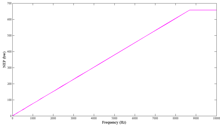
Figure 2.21 Noise equivalent power according to frequency (Hz).
