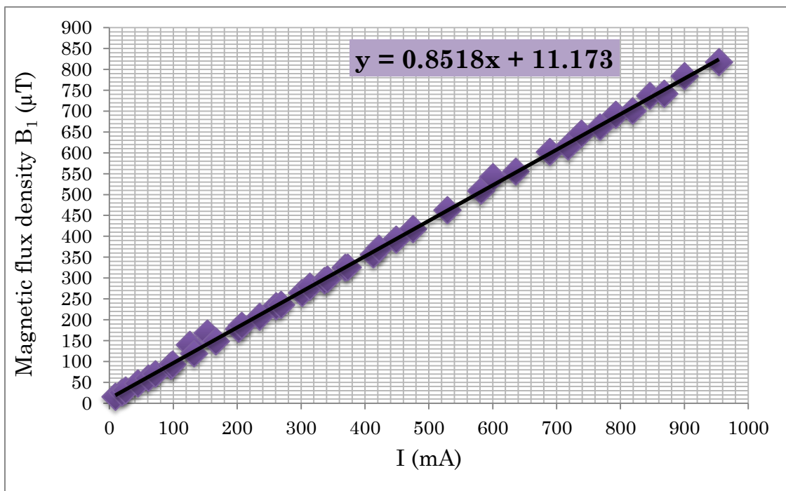
Figure 2.34 Measurement the magnetic flux density B_1 ( \mu\text{T} ) as a function of the input current (mA) applied to 60 Hz.
