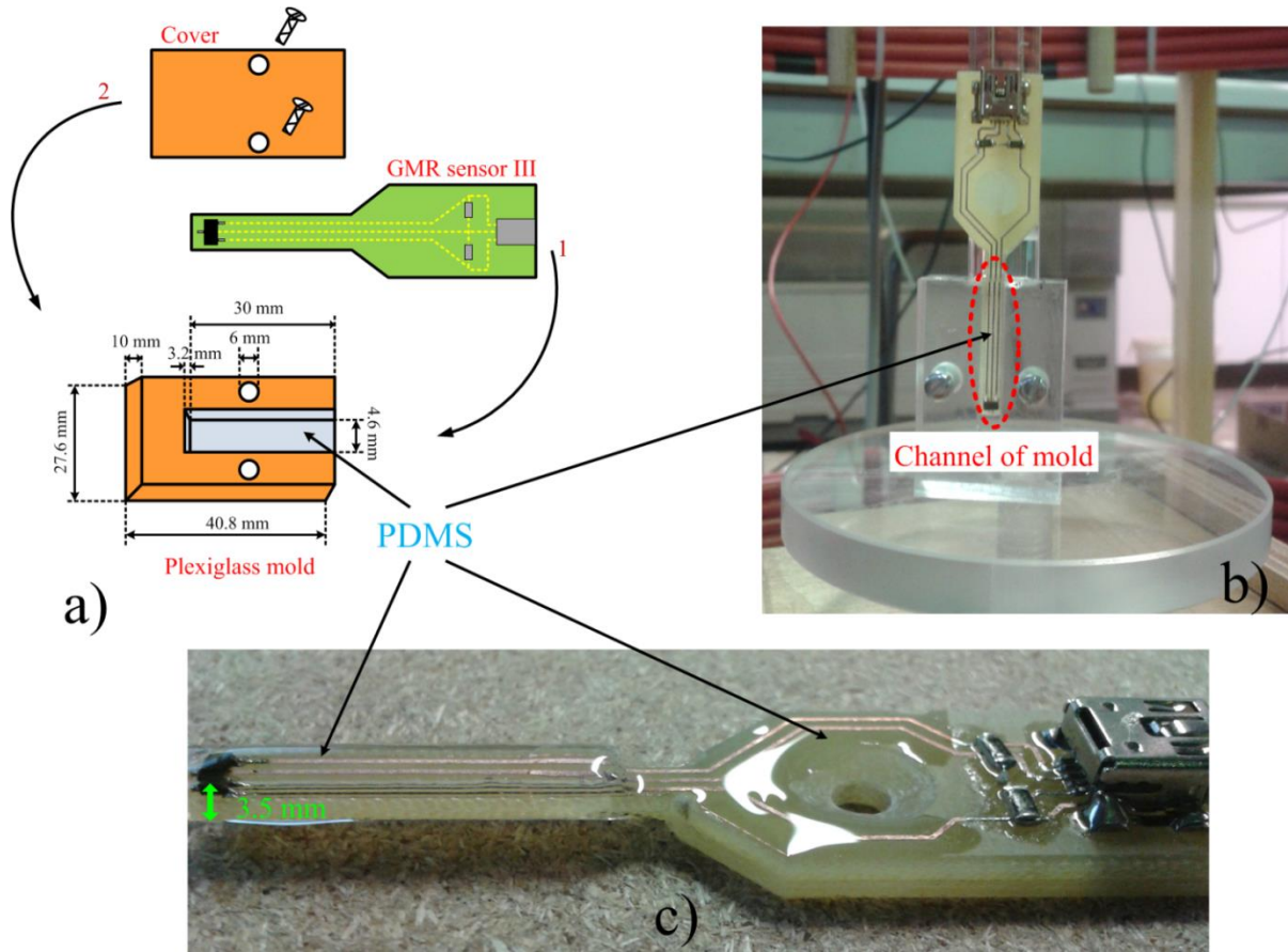
Figure 4.14 The insulation steps of GMR sensor: preparation of plexiglass mold (a), sensor's positing in the channel of mold (b), GMR sensor III with protective PDMS layers (c).
