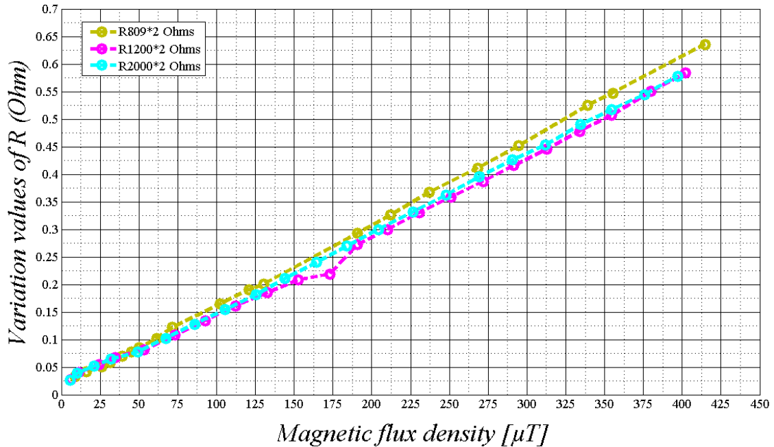
Figure 2.39 The values of \Delta R according to magnetic flux density ( \mu T ).
