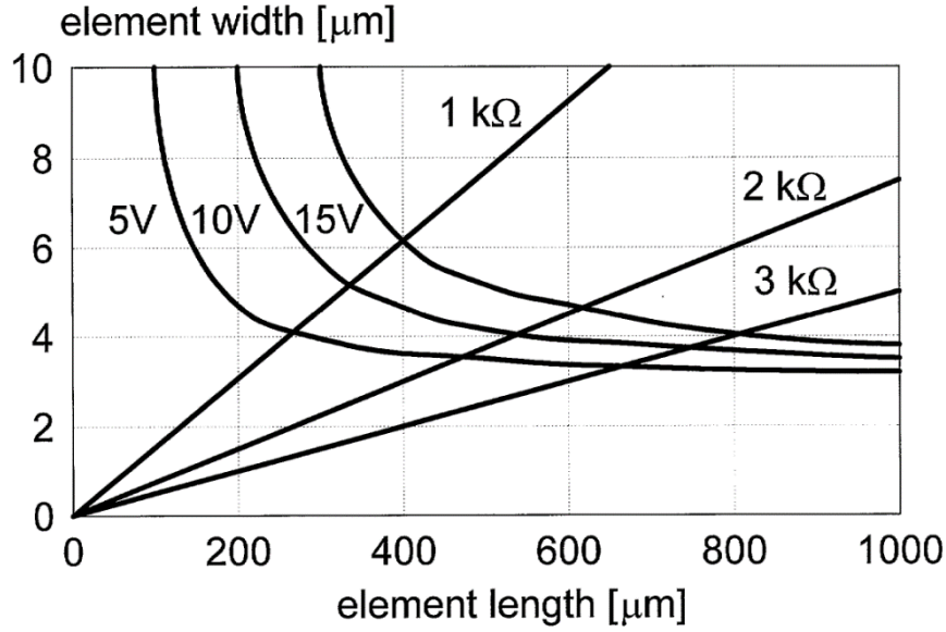
Figure 1.13 Relationship between design parameters of the spin-valve sensor [14, 24].
