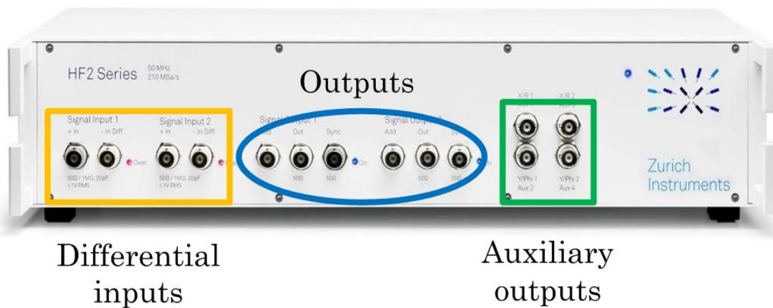
Figure 2.22 The schematic of the HF2IS Impedance Spectrometer.
