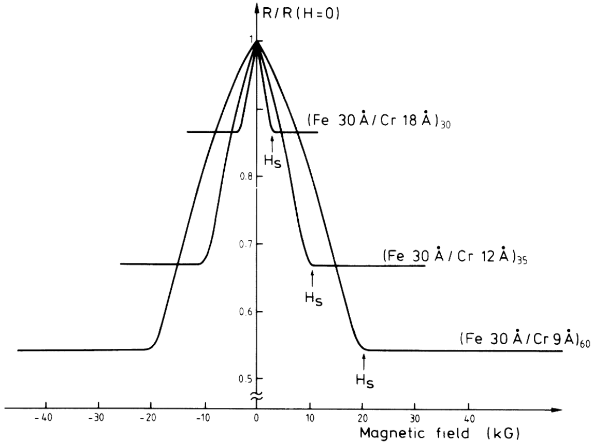
Figure 1.3 Magnetoresistance for several Fe/Cr multilayers at 4.2K [1].
