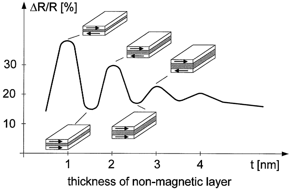
Figure 1.2 Evidence of oscillatory exchange coupling in thin film multilayers [3].
