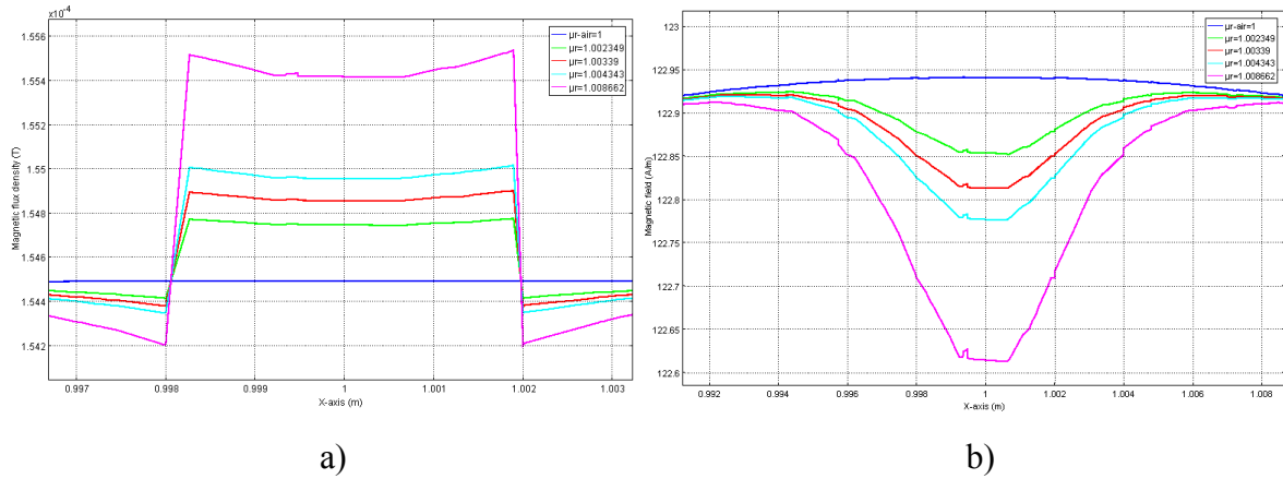
Figure 3.20 Variations of the curve of magnetic flux density (a) and magnetic field (b) in midpoint of the Helmholtz coil by presence the different ferrofluids ( \mu_r up than \mu_r -air).
