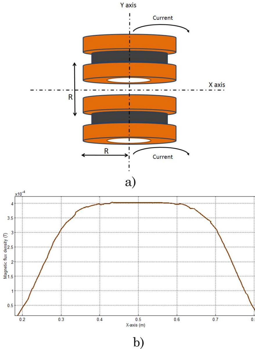
Figure 2.5 The Helmholtz coil structure (a), B (T) along the x-axis (b).
