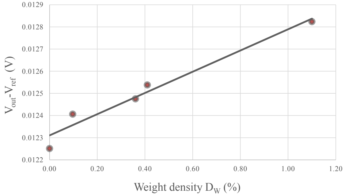
Figure 3.17 The relationship between the output signal from the GMR sensor and the weight density ( D_w %).
