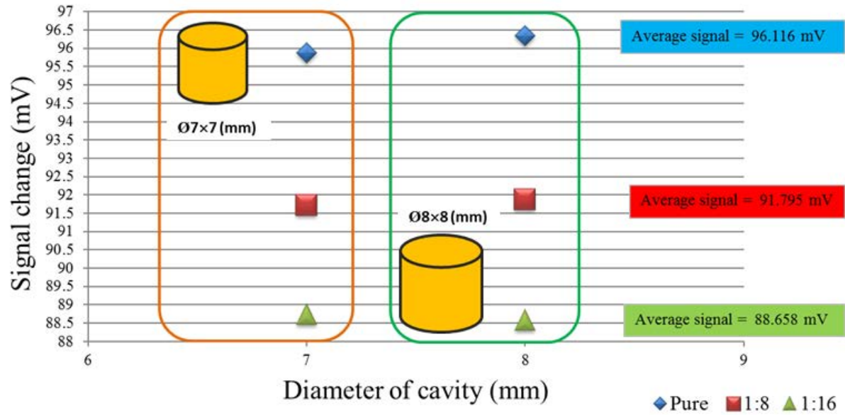
Figure 4.19 Signal changes measured in the cavities with S = 1 , N = 0.333 .
