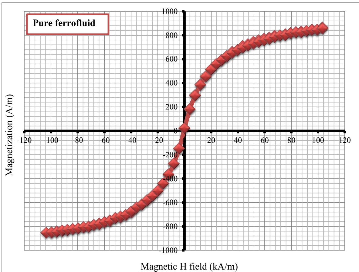
Figure 3.11 Magnetic hysteresis curve of pure ferrofluid.
