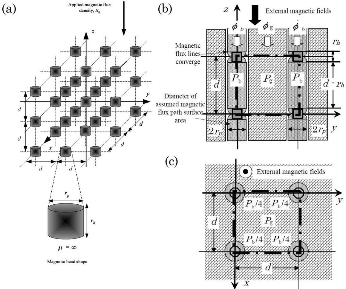
Figure 3.1 The magnetic model of nanoparticles (a), side view of magnetic path of a magnetic fluid in z -direction external magnetic field (b) and top view of magnetic circuit path (c) [75].
