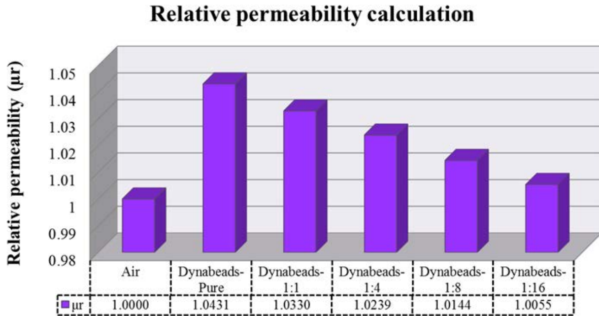
Figure 4.16 Relationship between relative permeability ( \mu_r ) and different magnetic fluid concentrations.
