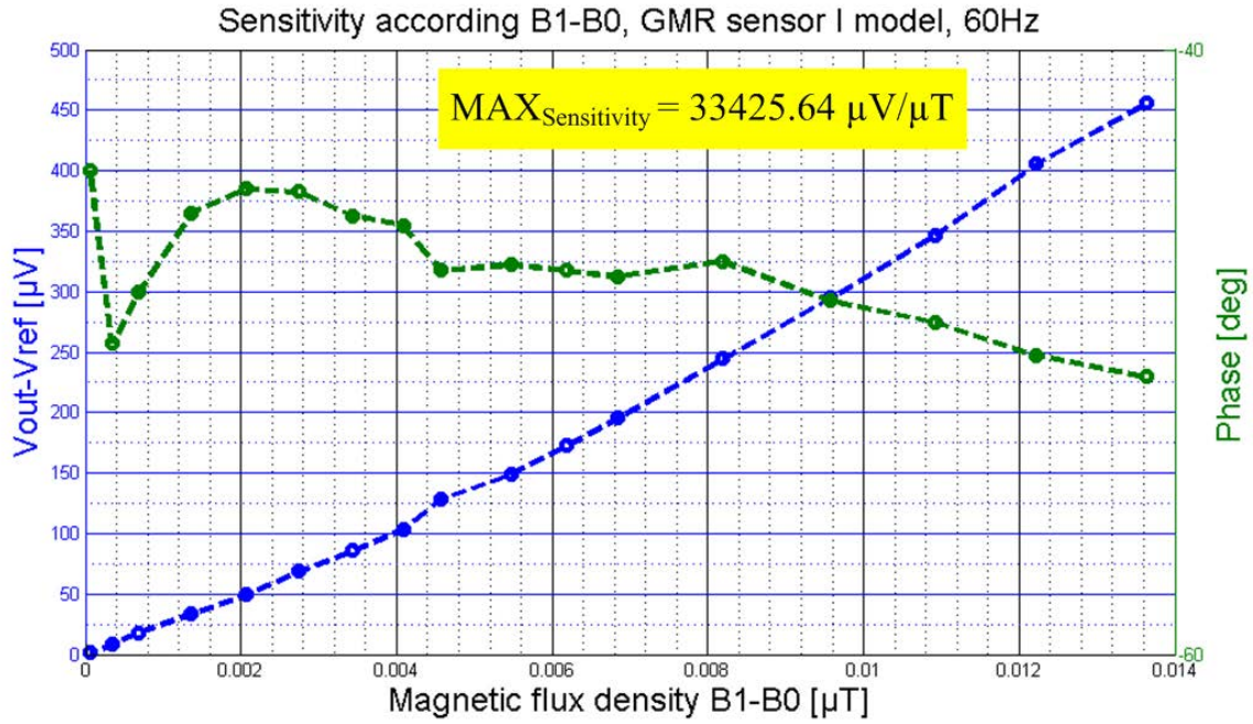
Figure 2.31 The output voltage result by GMR sensor I ( \mu V ) and phase calculation (deg) with two resistors ( 809 \Omega ) as a function of different magnetic flux density ( \mu T ) between two sensing elements GMR.
