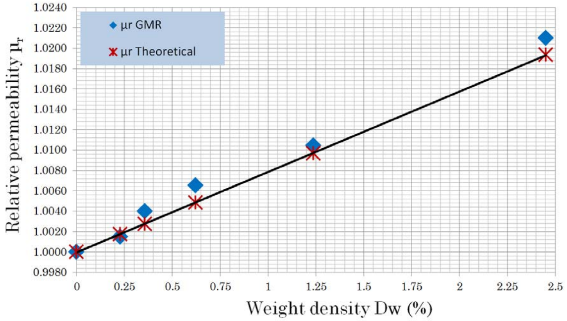
Figure 3.26 Experimental results of the relative permeability ( \mu_r ) as a function of different weight densities D_w (%) and comparison with the theoretical results.
