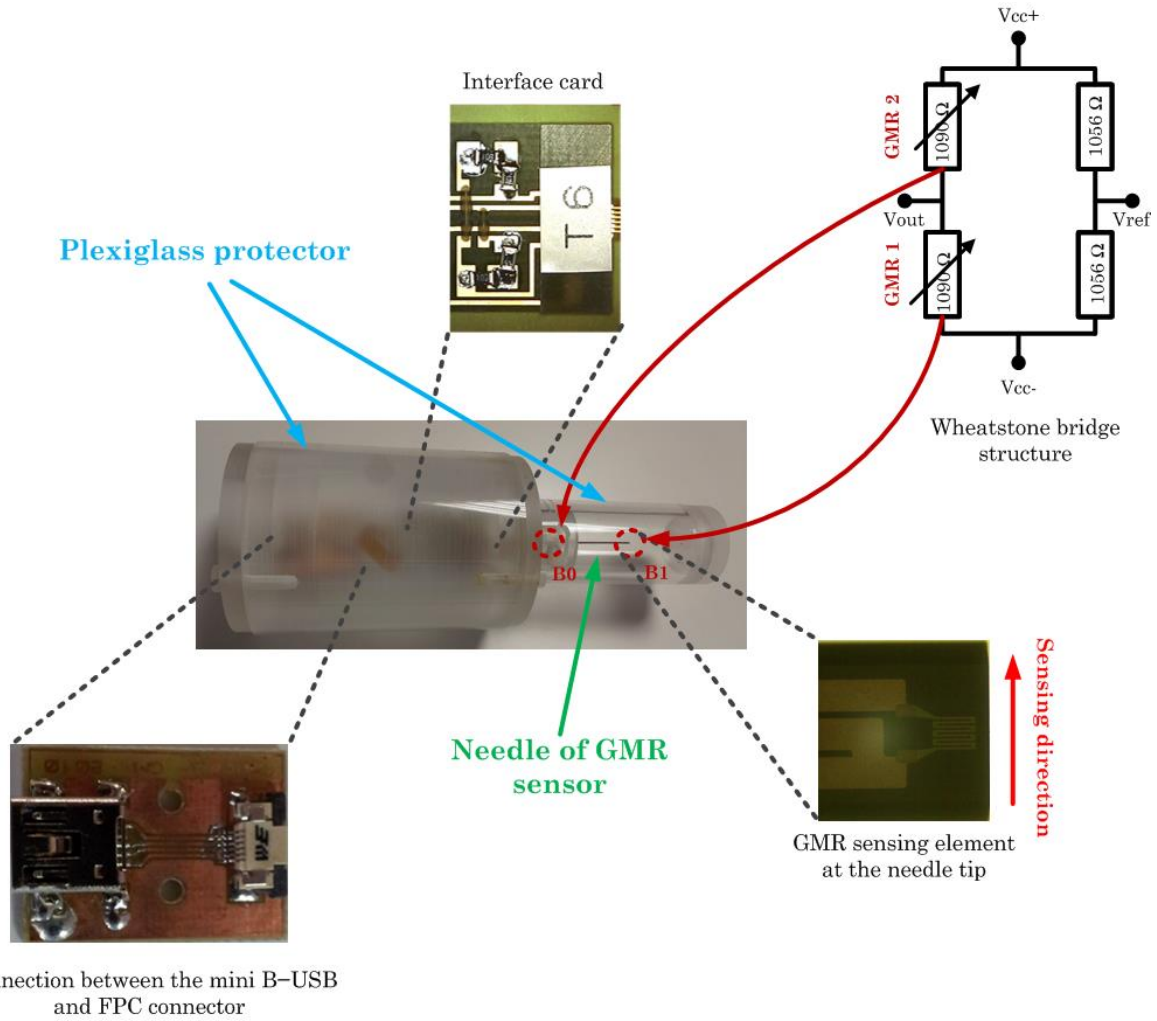
Figure 2.1 Schematic of first model of the GMR sensor.
