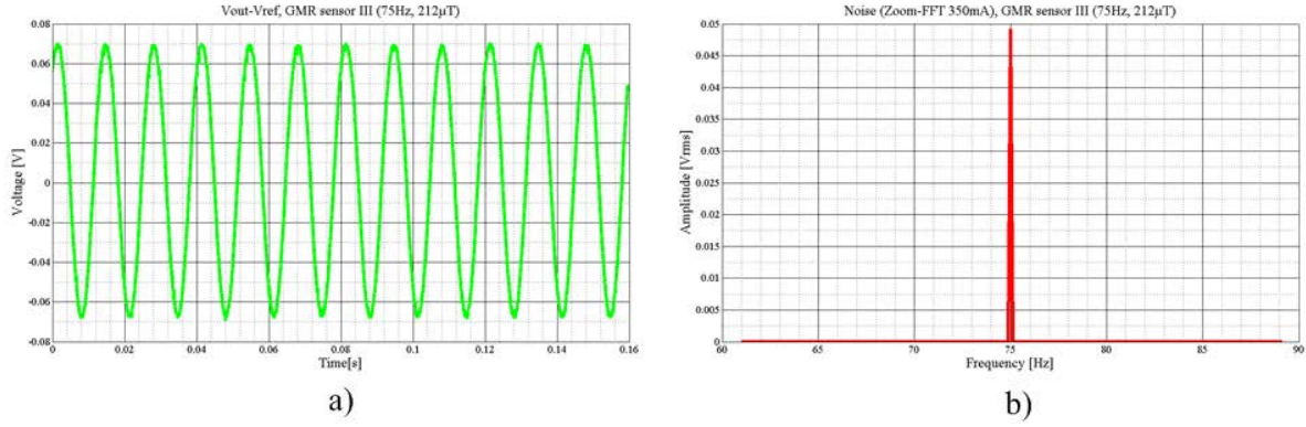
Figure 4.15 The output voltage ( V ) of GMR sensor (a) and the FFT detection from V_{out}-V_{ref} of the GMR sensor for frequency 75 Hz (b).
