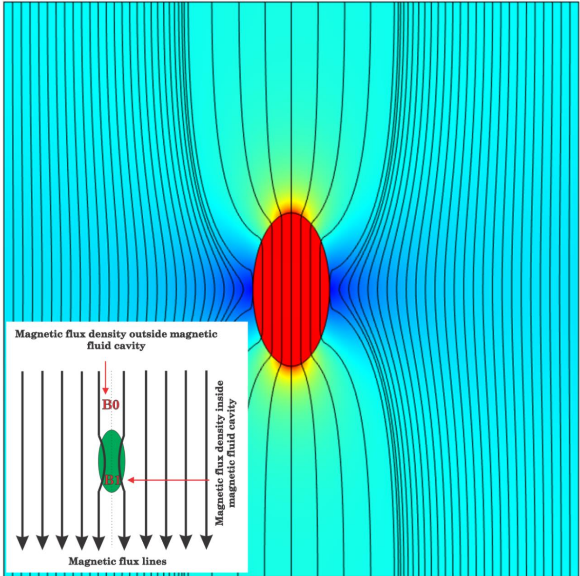
Figure 3.2 Distribution of magnetic flux density inside and outside of an ellipsoidal cavity.
