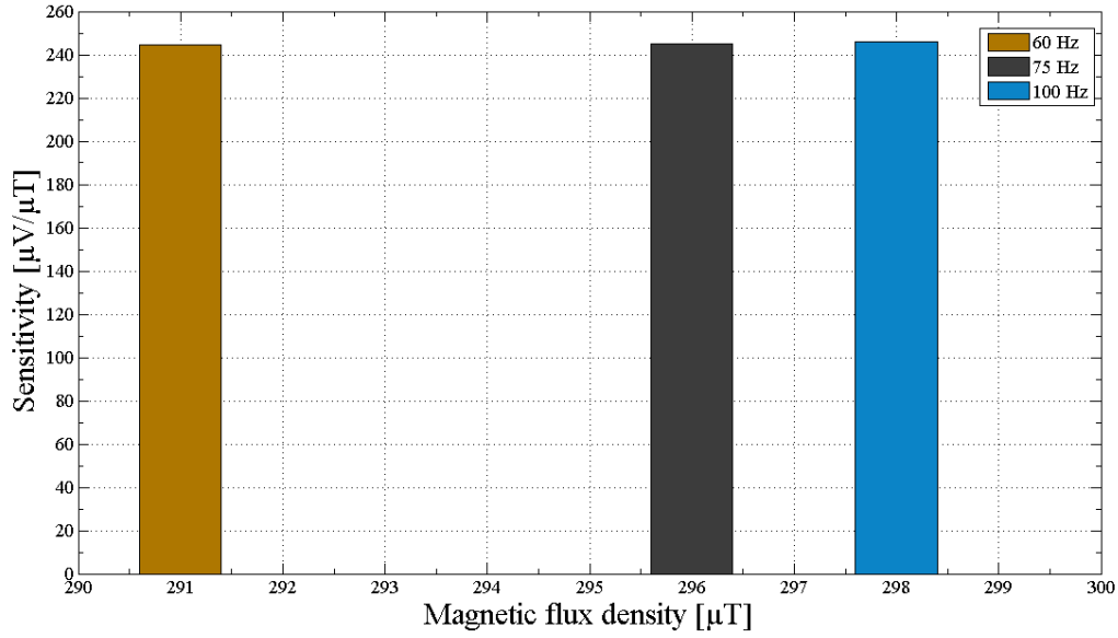
Figure 2.54 High value of sensitivity ( \mu\text{V}/\mu\text{T} ) as a function of B ( \mu\text{T} ) at f=60, 75, 100 Hz.
