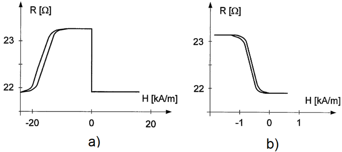
Figure 1.9 Hysteresis loops of the spin valve sensors [14].
