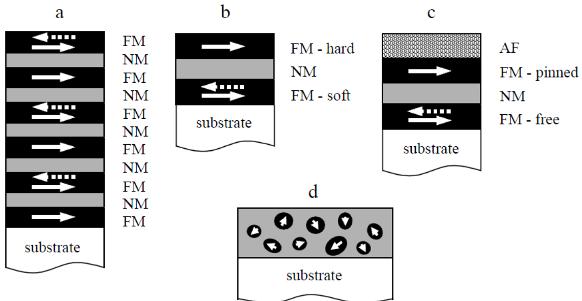
Figure 1.1 Various structures in which GMR can be observed: magnetic multilayer (a), pseudo spin valve as combine hard and soft magnetic (b), spin valve consists of a free layer (soft ferromagnetic layer), a non-magnetic metal spacer layer and pinned layer (ferromagnetic layer) (c), and granular thin film (d) [2].
