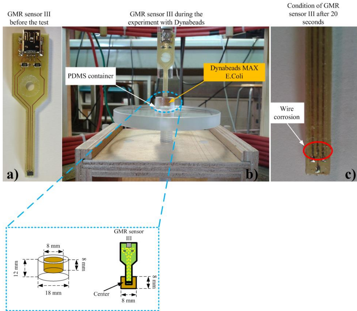
Figure 4.12 The GMR sensor type III status before the test (a), at the time of measuring (b) and after the experiment by Dynabeads (c).
