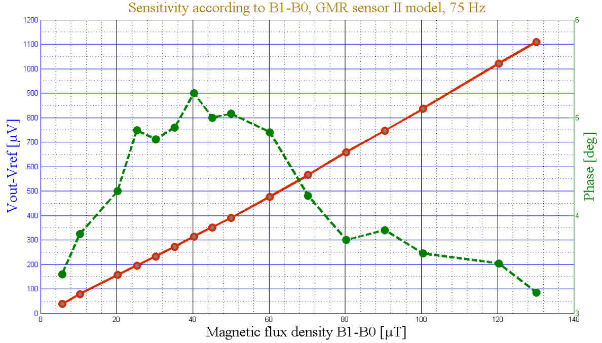
Figure 2.44 The output voltage results obtained by the probe GMR sensor ( \mu V ) and phase calculation (deg) with one resistor ( 2.128 K\Omega ) as a function of the changes in magnetic flux density ( \mu T ).
