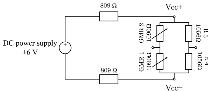
Figure 2.25 Power supply circuit by use two additional resistors.
