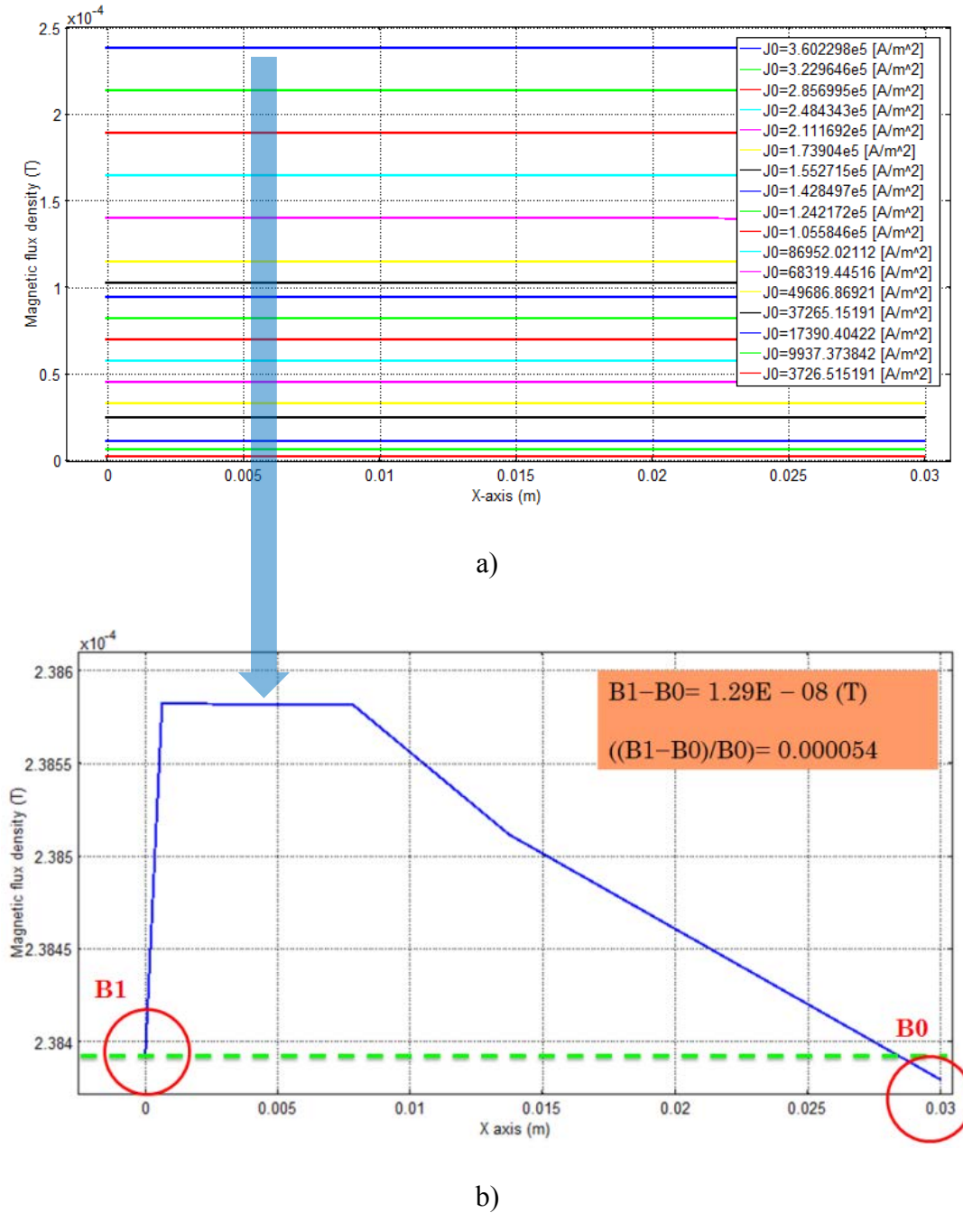
Figure 2.30 Distribution of the magnetic flux density (T) along the needle of sensor (a), zooming on a curve of the figure 2.30 (a) which presents the difference B between two GMR (b).
