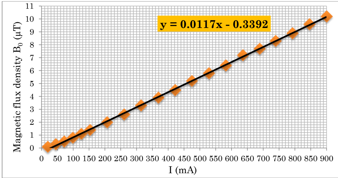
Figure 2.35 Measurement the magnetic flux density B_0 ( \mu\text{T} ) as a function of the input current ( \text{mA} ) applied to 60 Hz.
