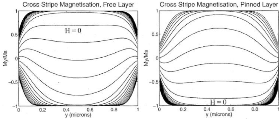
Figure 1.11 Calculations of the magnetization distribution of the spin-valve structure in pinned and free layers by [20].
