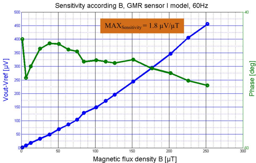
Figure 2.27 The output voltage ( \mu V ) and phase calculation ( deg ) with two resistors ( 809 \Omega ) as a function the total changes magnetic flux density B ( \mu T ).
