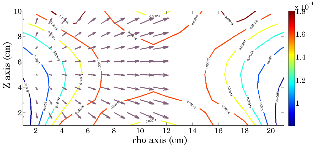
Figure 3.6 Distribution of magnetic flux density ( B ) in a sphere of the Helmholtz coil.
