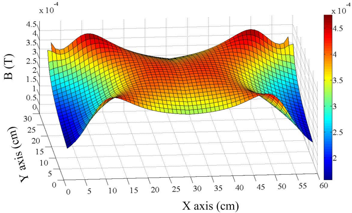
Figure 2.6 Distribution of magnetic flux density in Helmholtz coils.
