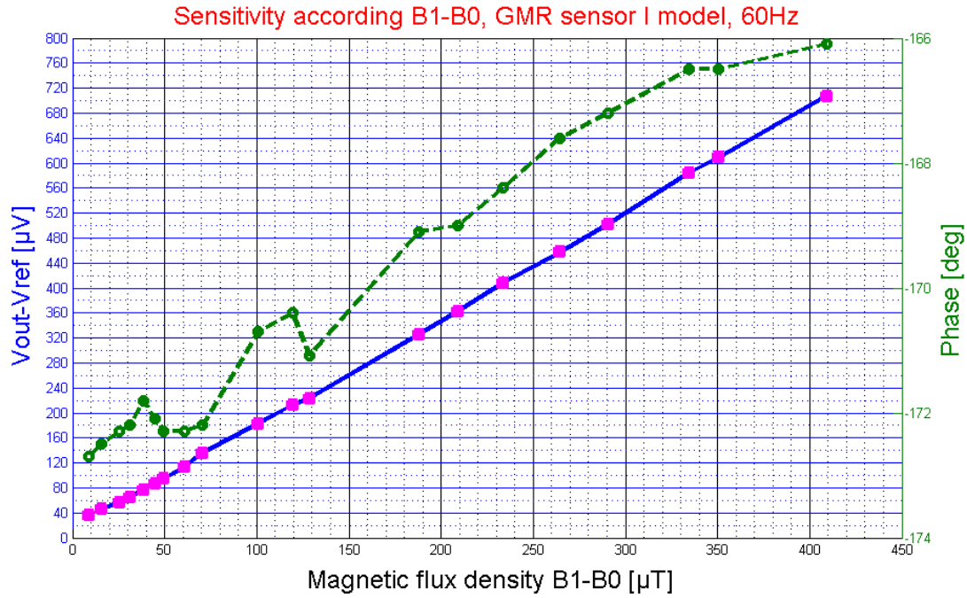
Figure 2.37 Output voltage ( \mu V ) and phase calculation (deg) with two resistors 809 \Omega as a function of the total changes magnetic flux density B_1 - B_0 ( \mu T ).
