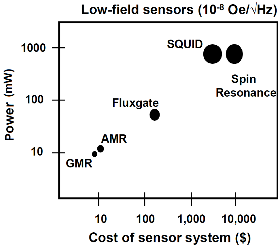
Figure 1.4 Comparison of power, price and size of several low magnetic field sensor technologies [4].
