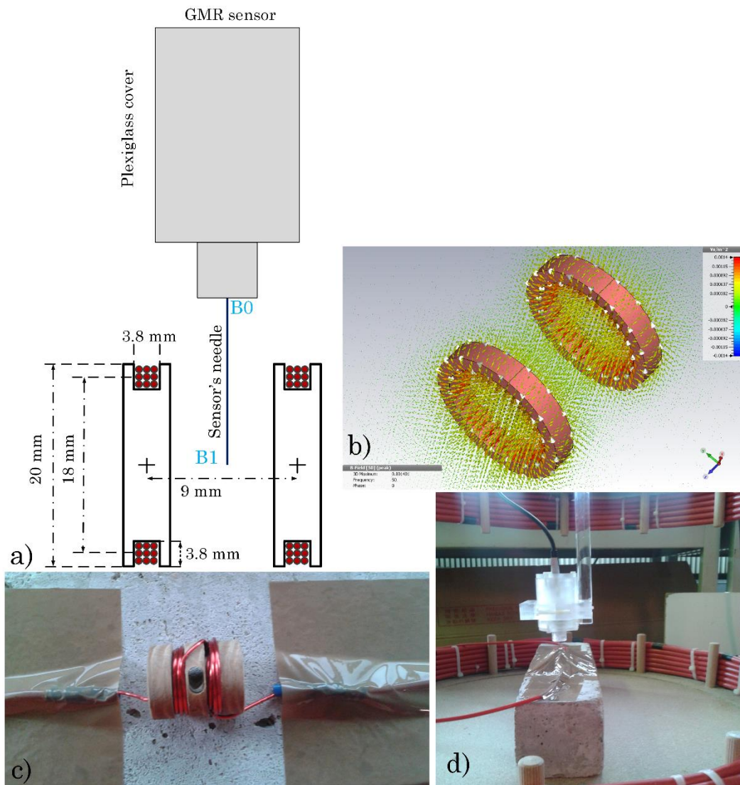
Figure 2.32 Schematic and actual images of small Helmholtz coil (a, c), uniform magnetic flux density simulated with CST (b), placing the sensor at center of coil (d).
