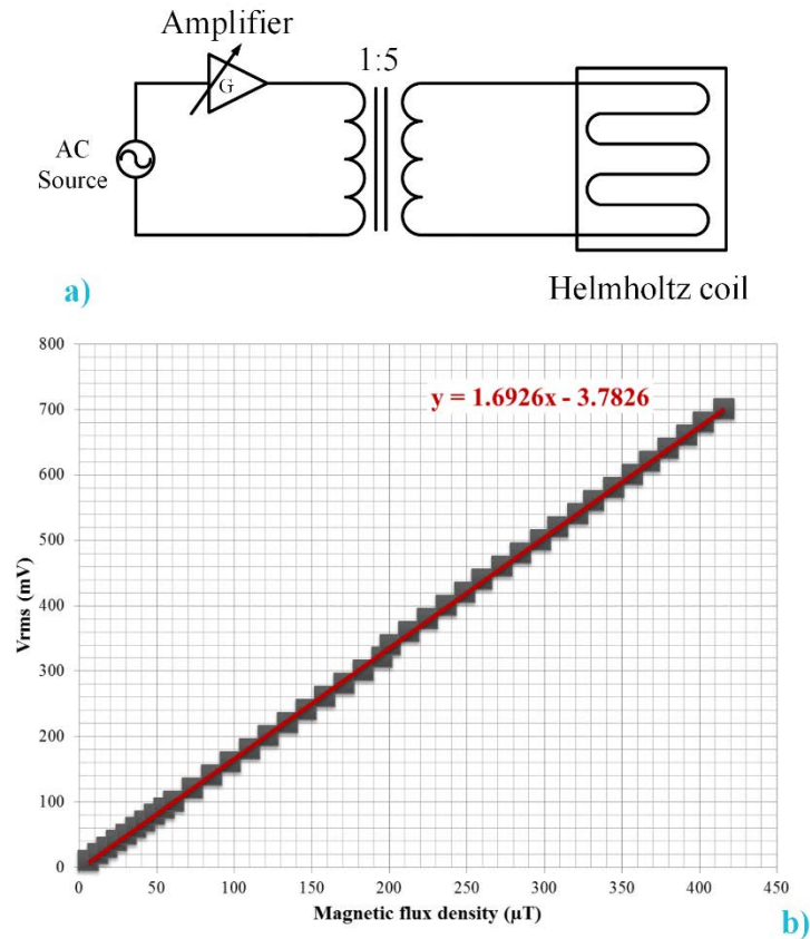
Figure 4.11 Helmholtz coil and its supply for operating in the frequency range 45-1000 Hz (a), measured magnetic flux density ( \mu T ) as a function of signal amplitude ( V_{rms} ) applied at 75 Hz (b).
