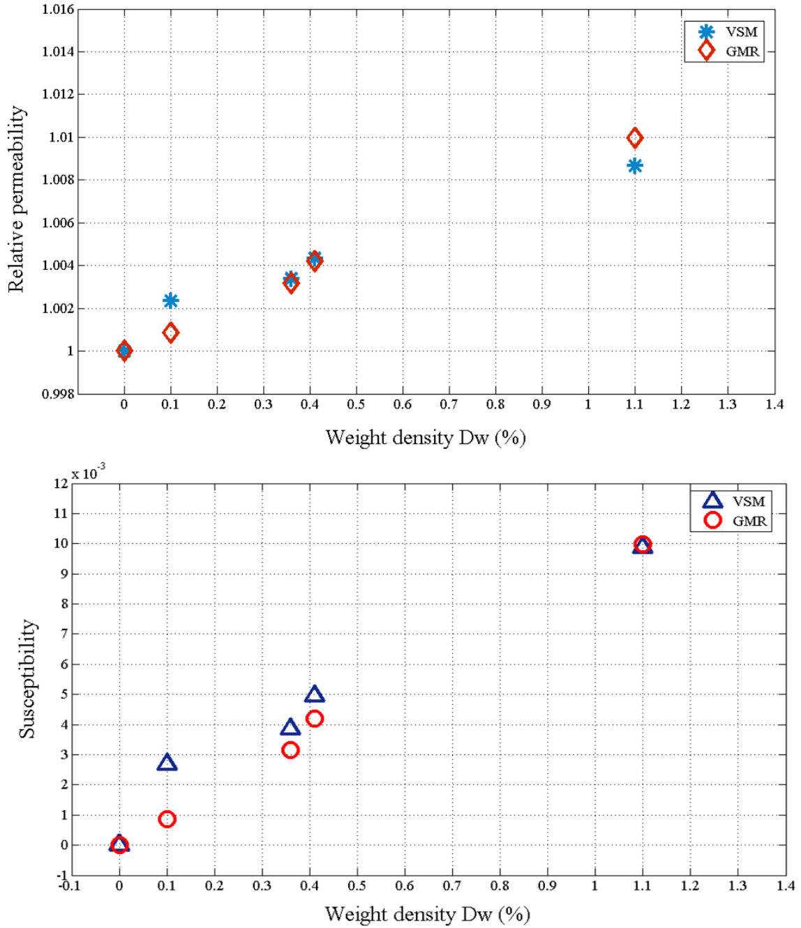
Figure 3.18 The experimental results of relative permeability and susceptibility according to several weight densities (%) of ferrofluid.
