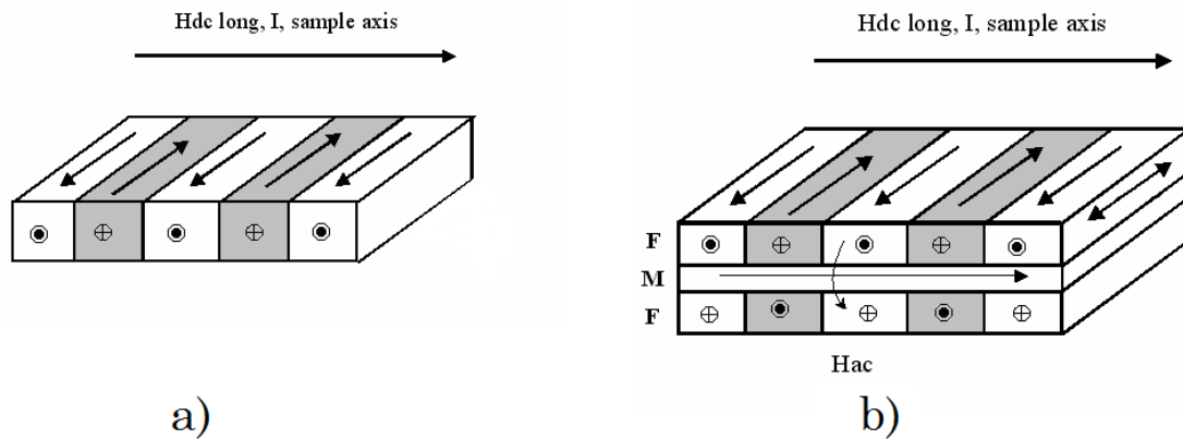
Figure 1.16 The giant magnetoimpedance configuration; in single layered (a) and in multilayered (b) thin films [34].
