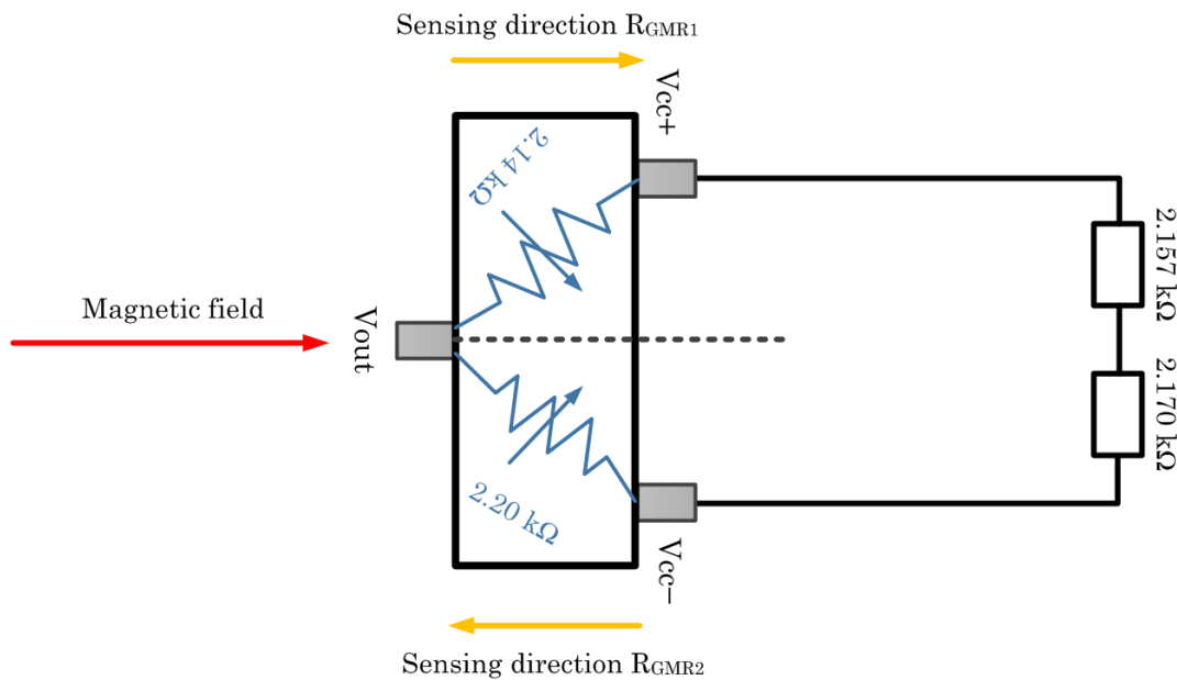
Figure 2.51 The Wheatstone bridge configuration of the GMR sensor type III.
