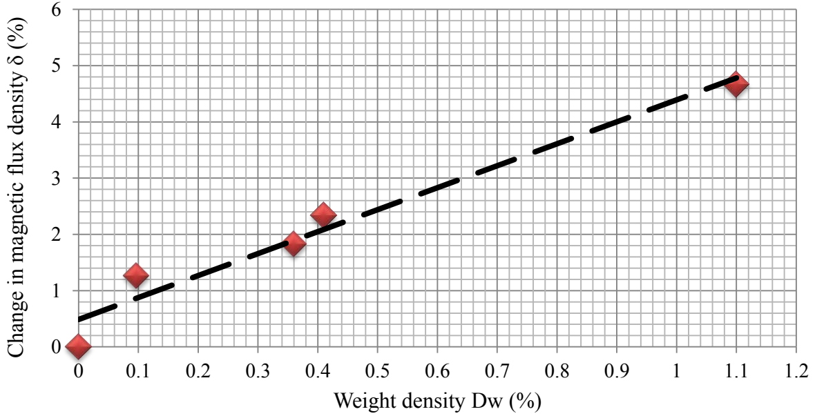
Figure 3.19 The change of magnetic fluid density ( \delta %) with different weight densities ( D_w %).
