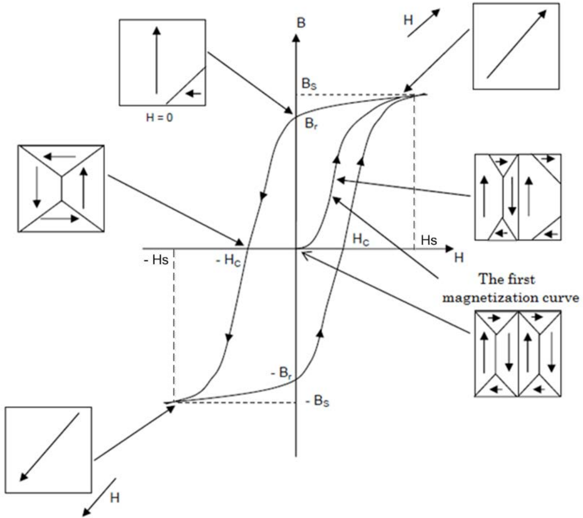
Figure 1.21 The basic magnetization curve and hysteresis loop of a ferromagnetic: B refers to the magnetization of the particle; H is the magnetic field; B_s is saturation magnetization for H > H_s ; H_s is saturation field corresponding to B_s ; B_r is residual magnetization; H_c is coercive force or field necessary for the demagnetization of the particle [43].
