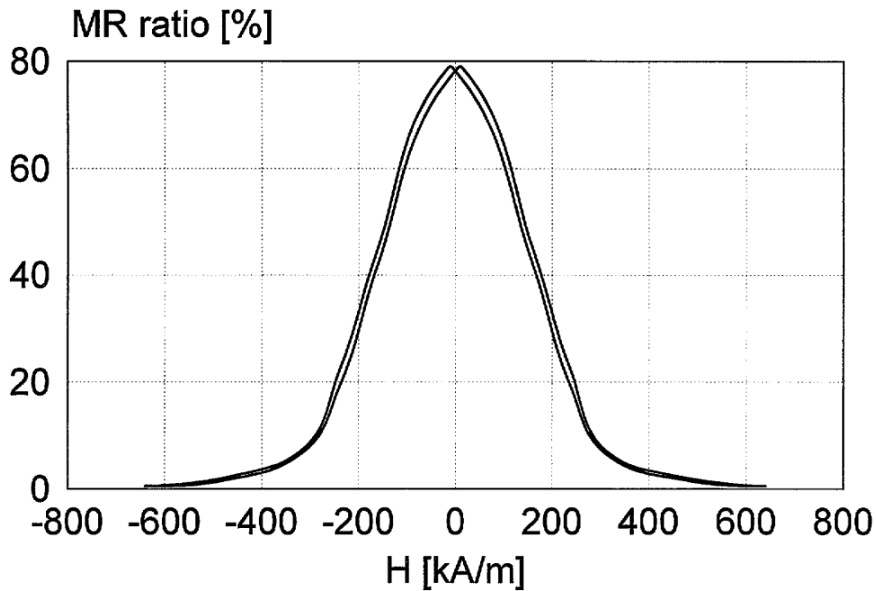
Figure 1.7 Characteristic of the GMR multilayer structure by (Co 1.5 nm/Cu 0.9 nm)×30 multilayer structure depends of magnetic fields [13, 14].
