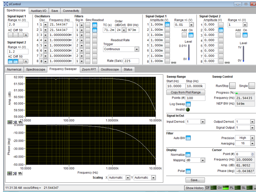
Figure 2.23 Interface program of the HF2IS Impedance Spectrometer.
