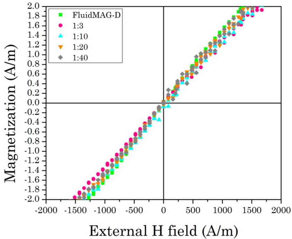
Figure 3.23 Confirmation the results of different concentrations with use the VSM's data.
