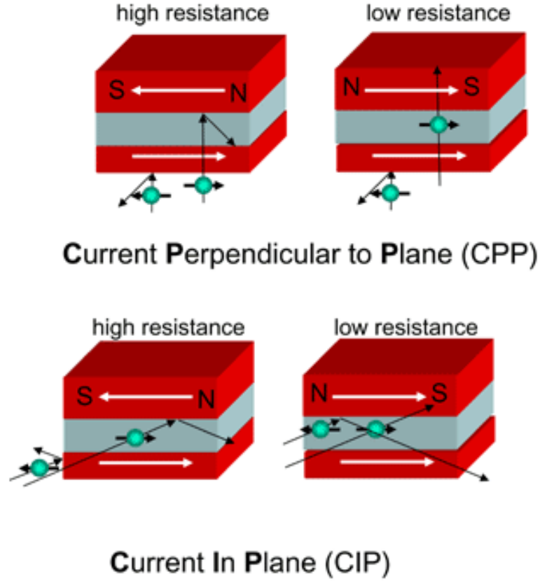
Figure 1.14 Schematic of current perpendicular to plane (CPP) and the current in plane (CIP) geometry [25].
