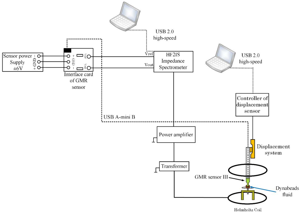
Figure 4.10 Schematic of measurement setup organized to estimate the magnetic properties of Dynabeads.
