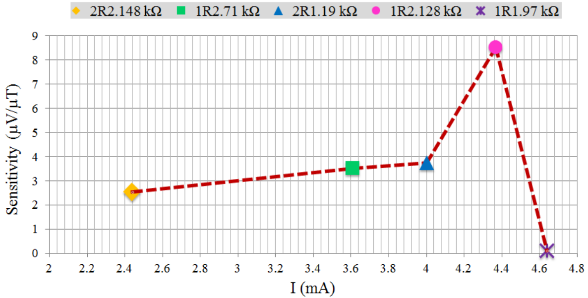
Figure 2.49 The relationship between sensor's sensitivity and its input current according to various resistances in interface supply card of the GMR sensor.
