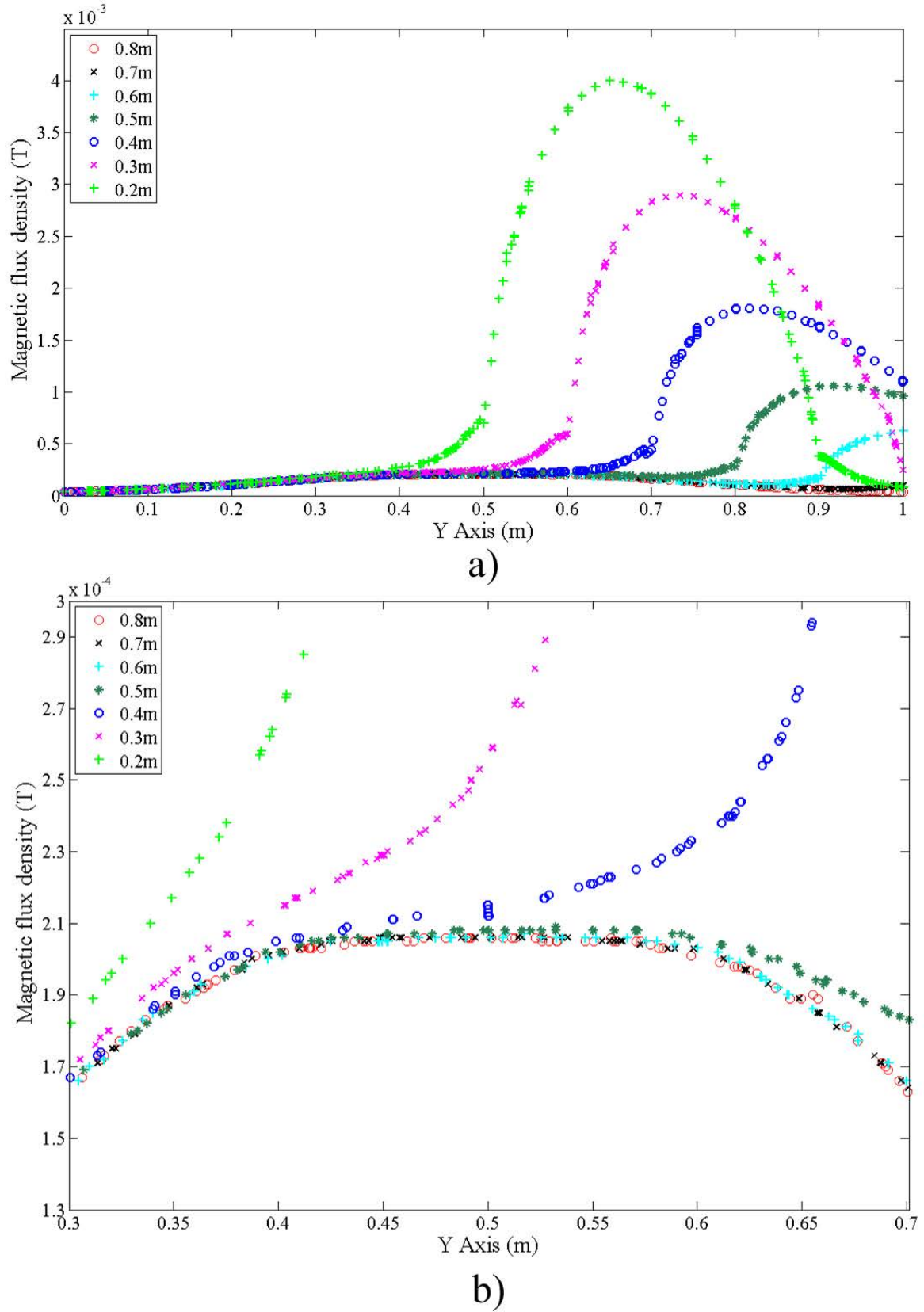
Figure 2.13 Changing the magnetic flux density according to the moving of the displacement system along the Y axis (a), the change of magnetic flux density in midpoint of the Helmholtz coil considering the system of the GMR sensor (b).
