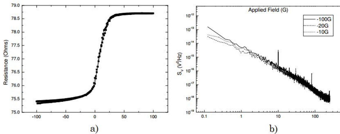
Figure 1.12 GMR characteristics as a function of the magnetic induction (a), 1/f noise in a yoke-type GMR (b) [21].
