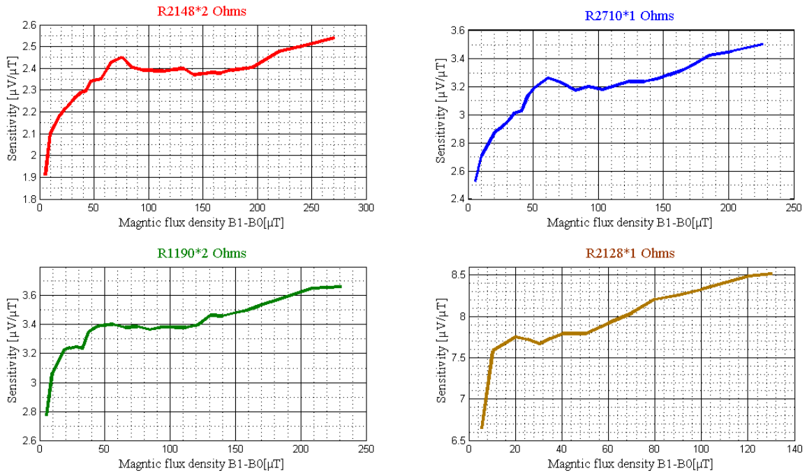
Figure 2.45 The relationship between sensitivity ( \mu V/\mu T ) and the magnetic flux density ( \mu T ) variations for different resistances values in the power supply card of the GMR sensor.
