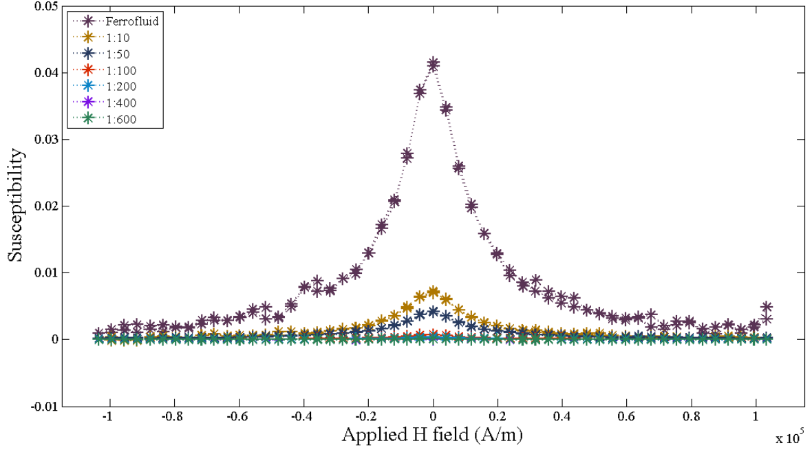
Figure 3.14 Initial magnetic susceptibility \chi_i as a function of an applied field (A/m).
