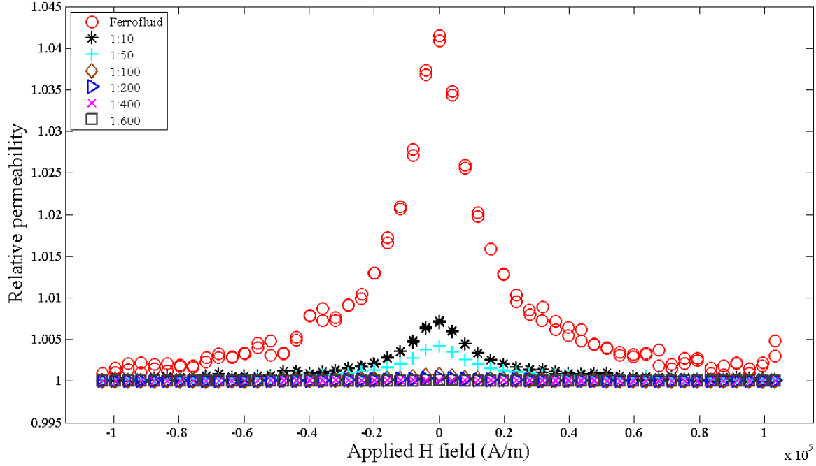
Figure 3.13 Initial relative permeability ( \mu_{ri} ) as a function of an applied field (A/m).
