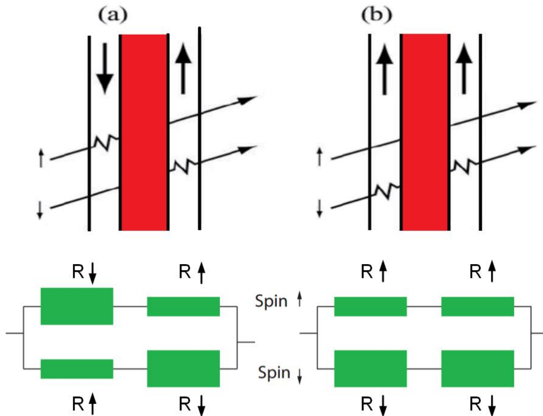
Figure 1.6 Schematic of giant magnetoresistance in a multilayer, two magnetic layers are polarized in the opposite directions (a) or in the same direction (b).
