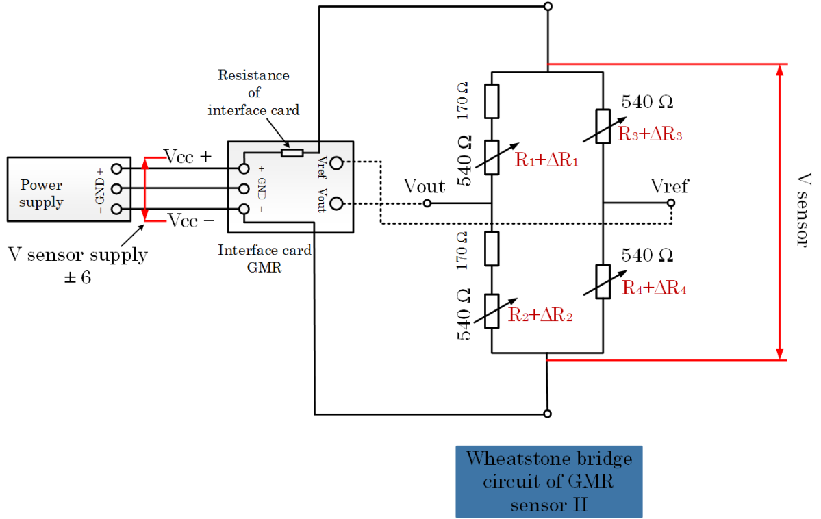
Figure 2.47 Schematic of the GMR II sensor (second model).
