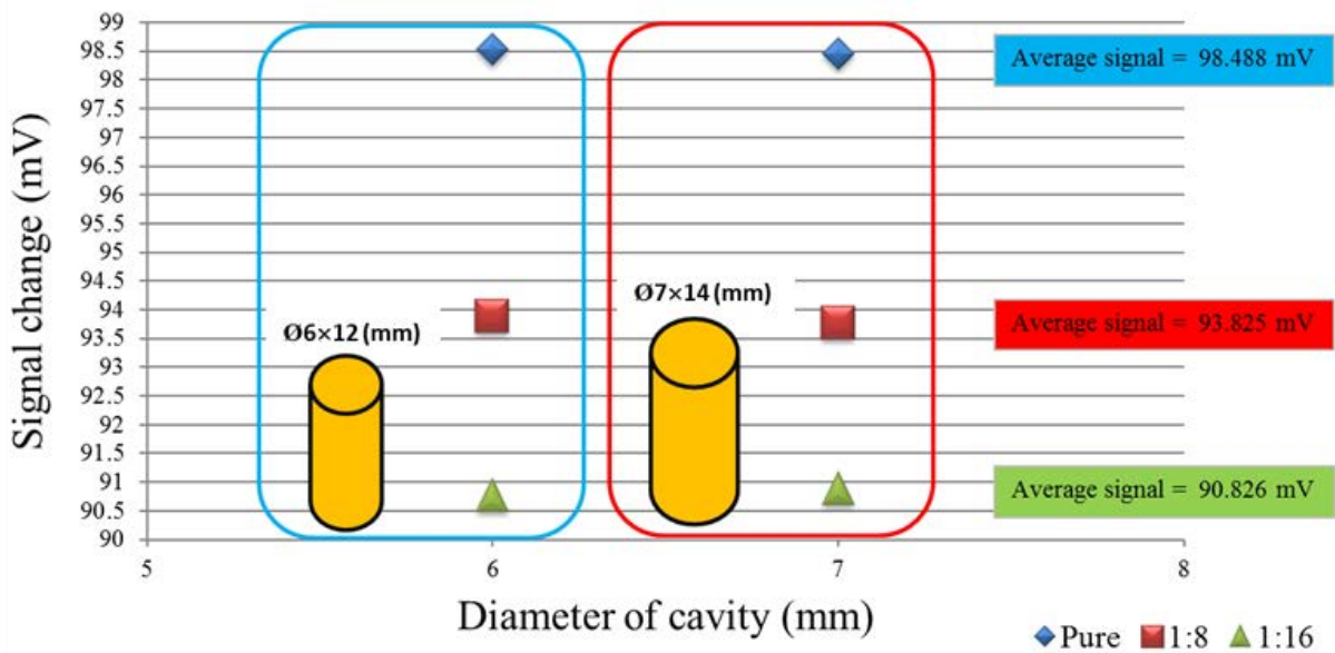
Figure 4.20 Signal changes measured in the cavities with S = 2 , N = 0.172 .
