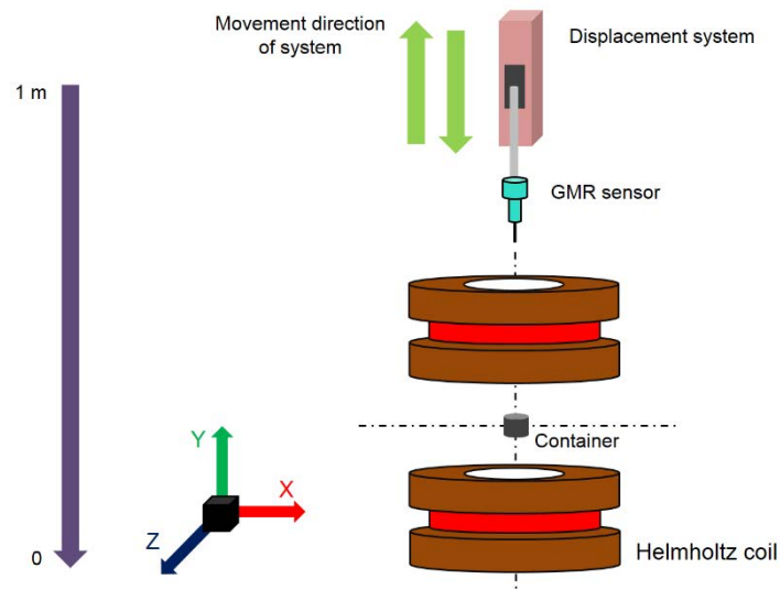
Figure 2.12 Positioning the displacement system of the GMR sensor.
