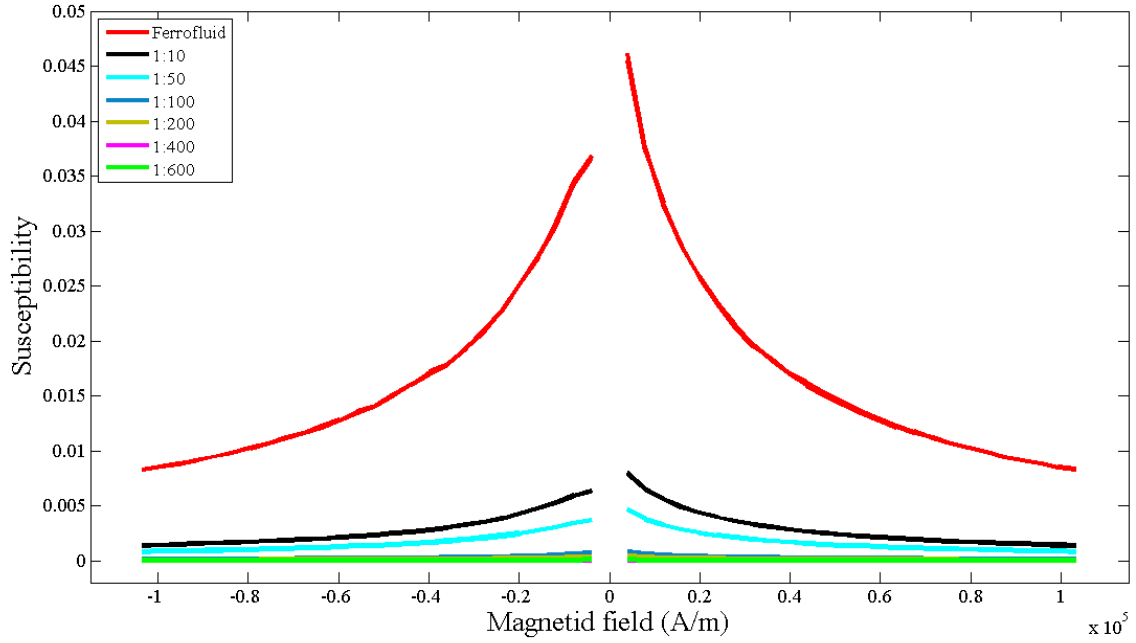
Figure 3.15 Magnetic susceptibility ( \chi ) as a function of an applied field (A/m).
