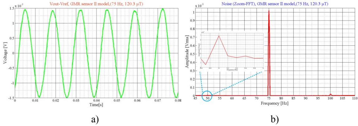
Figure 2.43 The GMR sensor's output voltage ( V ) with 2.128 k \Omega (a) and FFT detection from V_{out}-V_{ref} of the GMR sensor for frequency 75 Hz (b).
