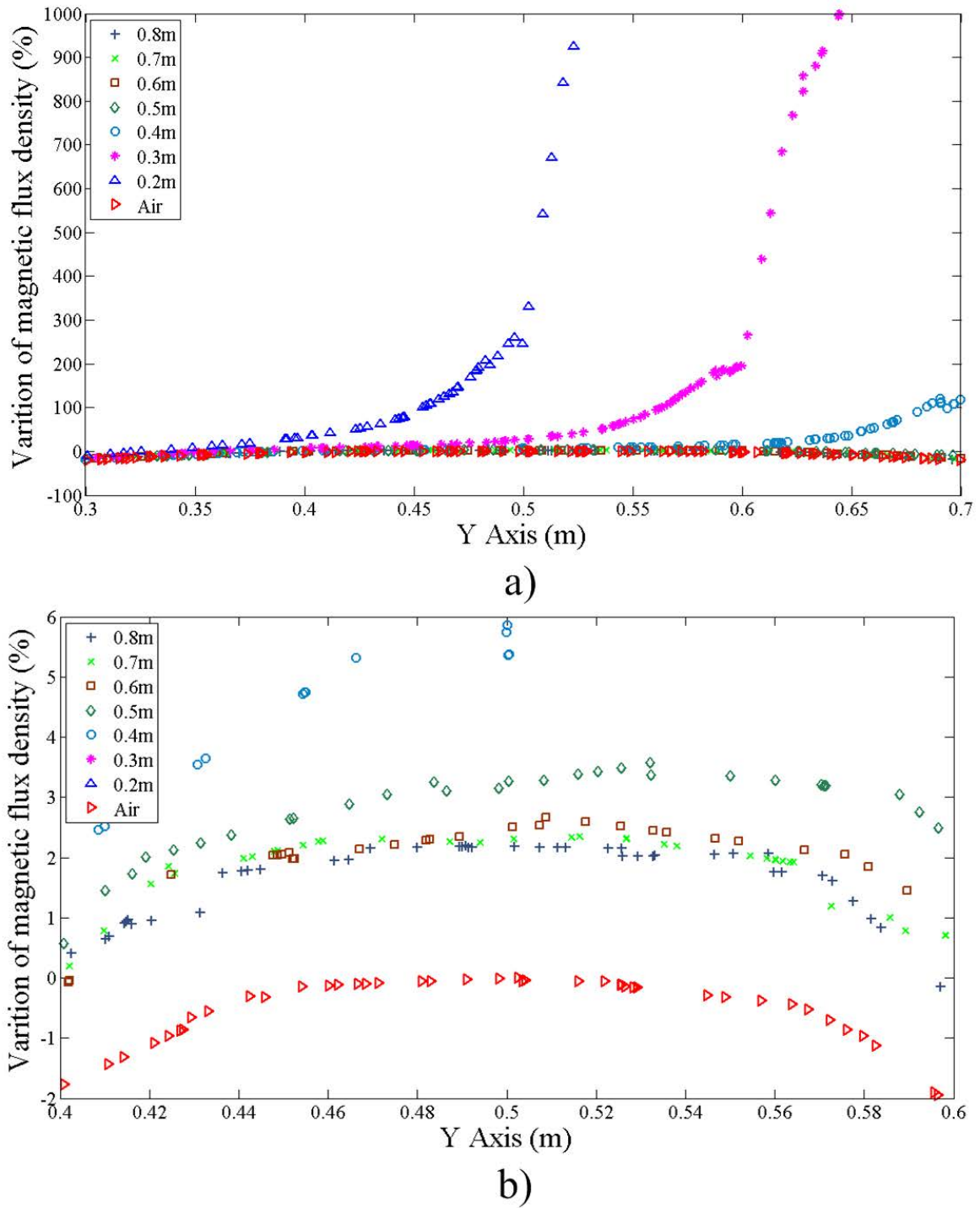
Figure 2.15 Calculation of the percentage error (%) of magnetic flux density variation as function of the system position along the Y axis (a), the variation of (B) % in the center of coil (b).
