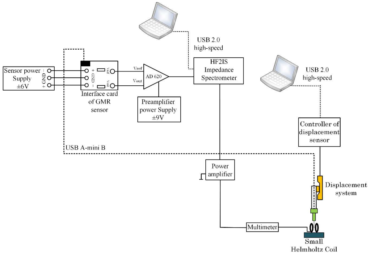
Figure 2.33 Measurement setup for sensor characterization.
