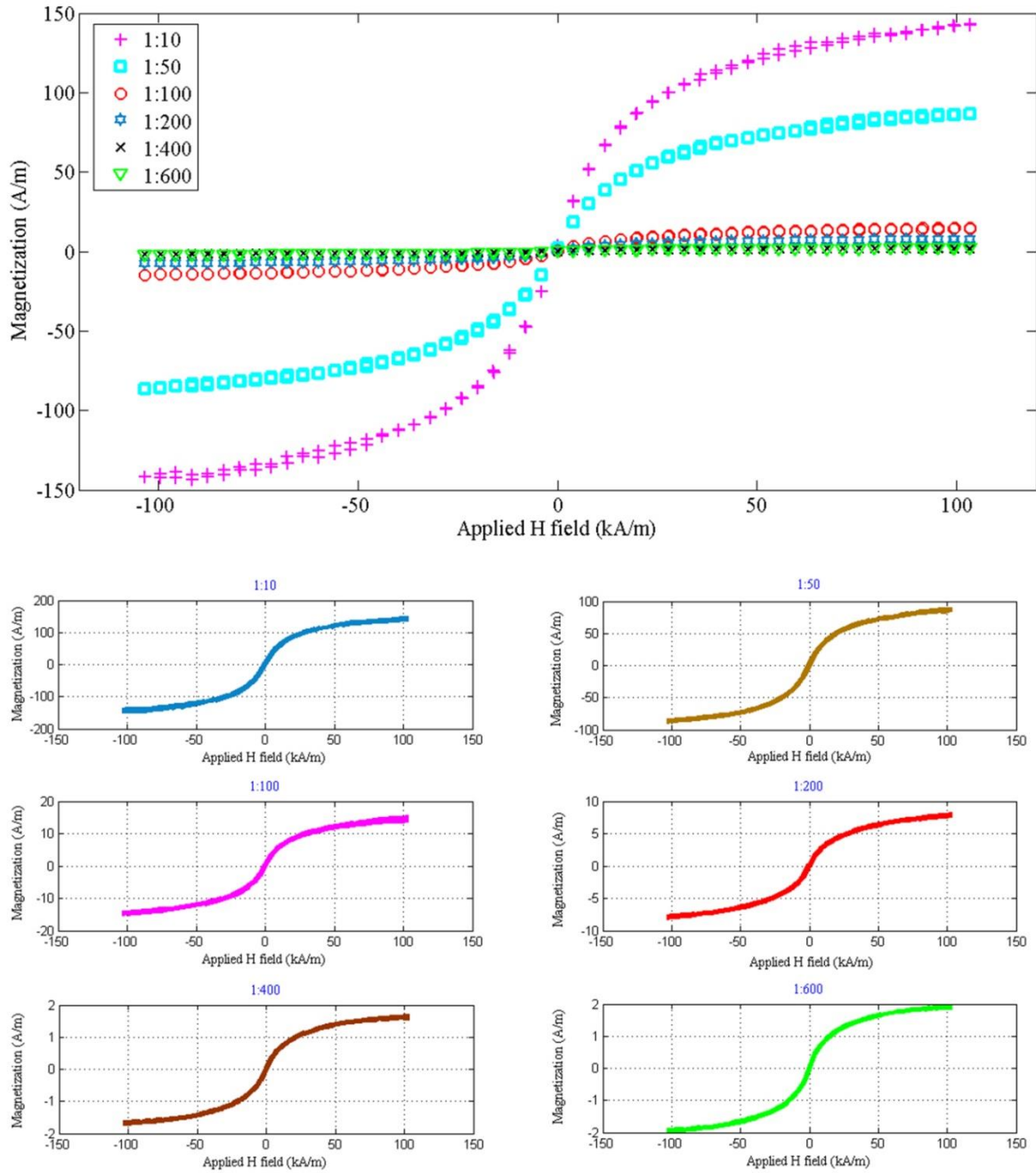
Figure 3.12 Hysteresis curve of fluids obtained from pure ferrofluid.
