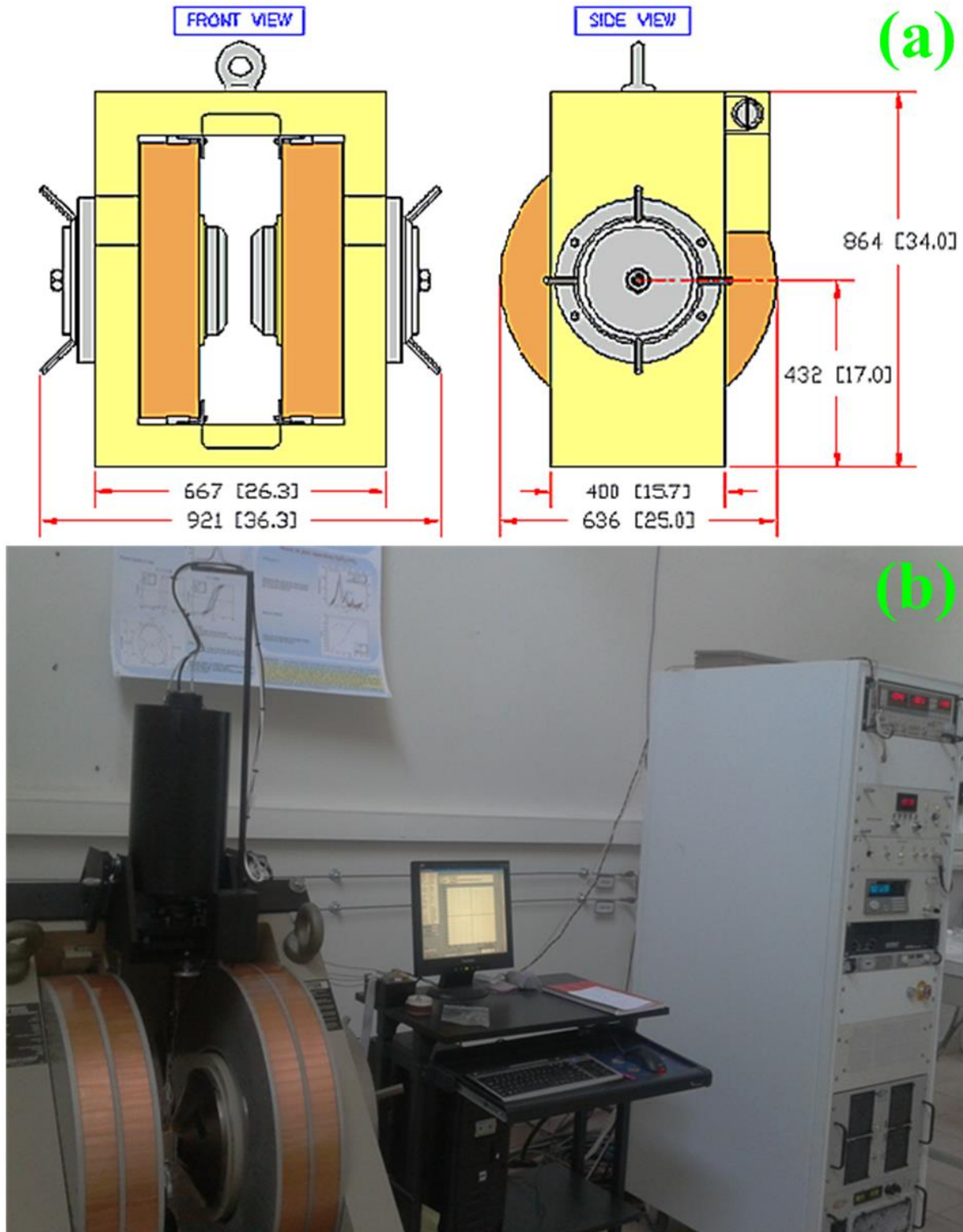
Figure 3.7 Dimensions (a) [84] and real image (b) of the VSM measurement setup.
