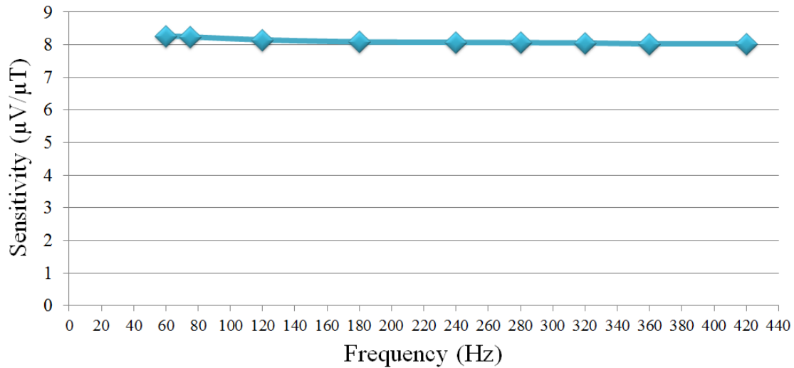
Figure 2.46 Experimental results obtained with GMR sensor to calculate the sensitivity as function of frequency (60 Hz – 420 Hz) with (B_1 - B_0) = 87.6 \mu T .
