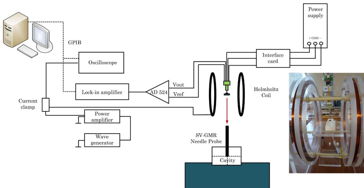
Figure 3.4 Measurement setup.
