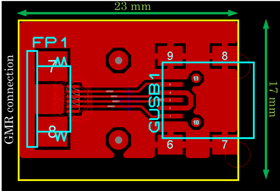
Figure 2.2 Schema of PCB card for connection the mini B-USB and FPC connector.
