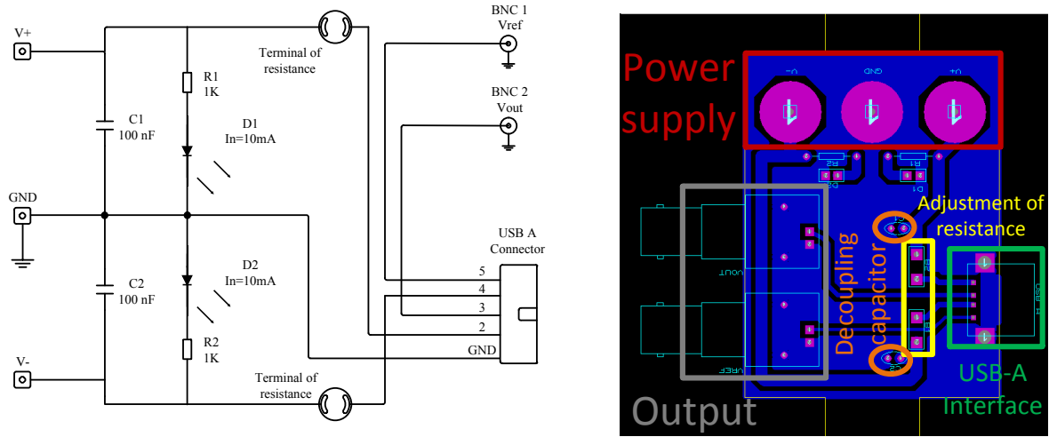
Figure 2.3 The schematic of connection cart between sensor and power supply.
