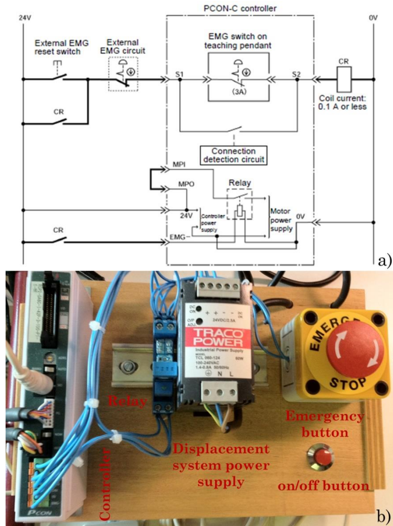
Figure 2.11 Electrical schematic (a) [69], control panel (b) of displacement system.
