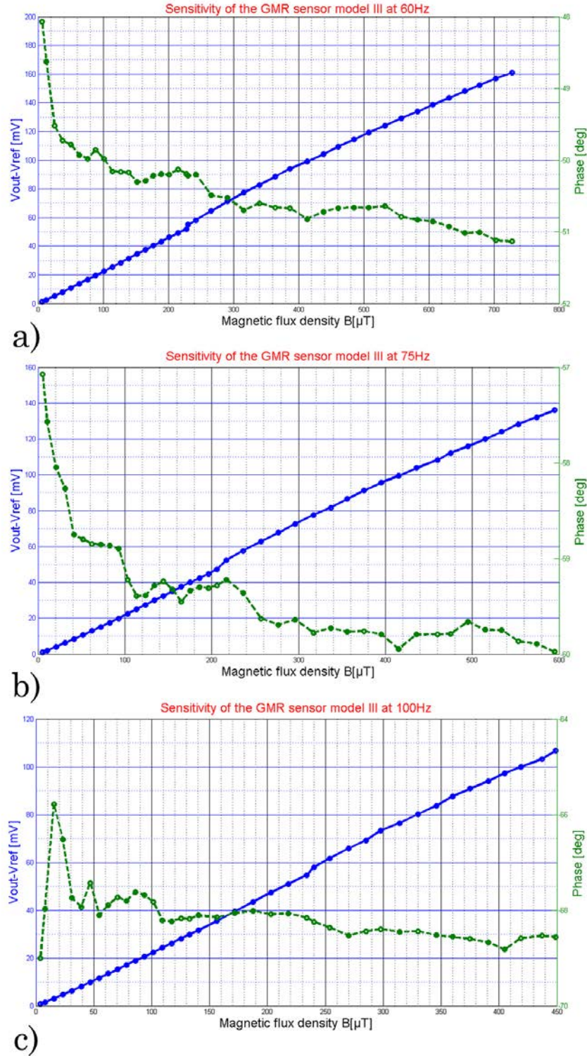
Figure 2.53 Experimental results of sensitivity obtained with the GMR sensor III at different frequencies of 60 (a), 75 (b) and 100 Hz (c).
