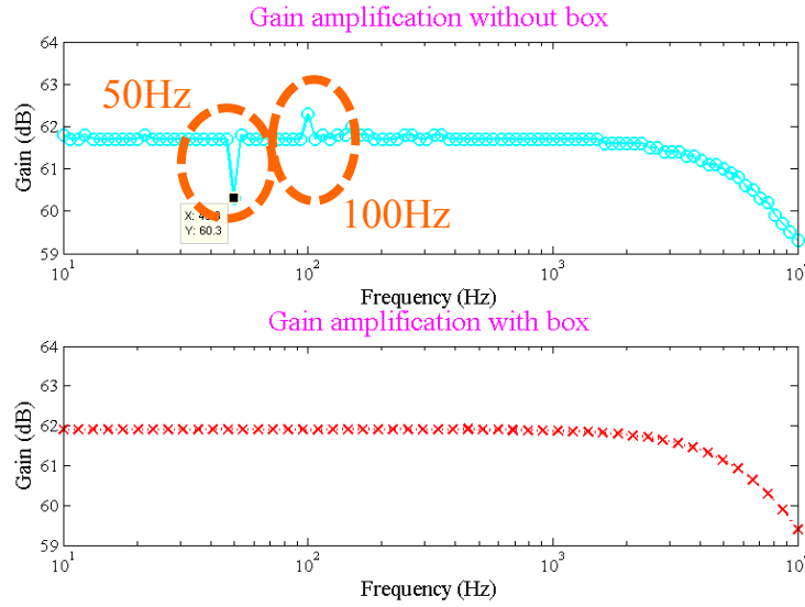
Figure 2.19 The amount of gain as a function of frequency.
