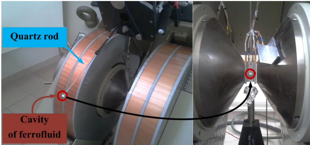
Figure 3.10 The placing of container of ferrofluid in center of the VSM.
