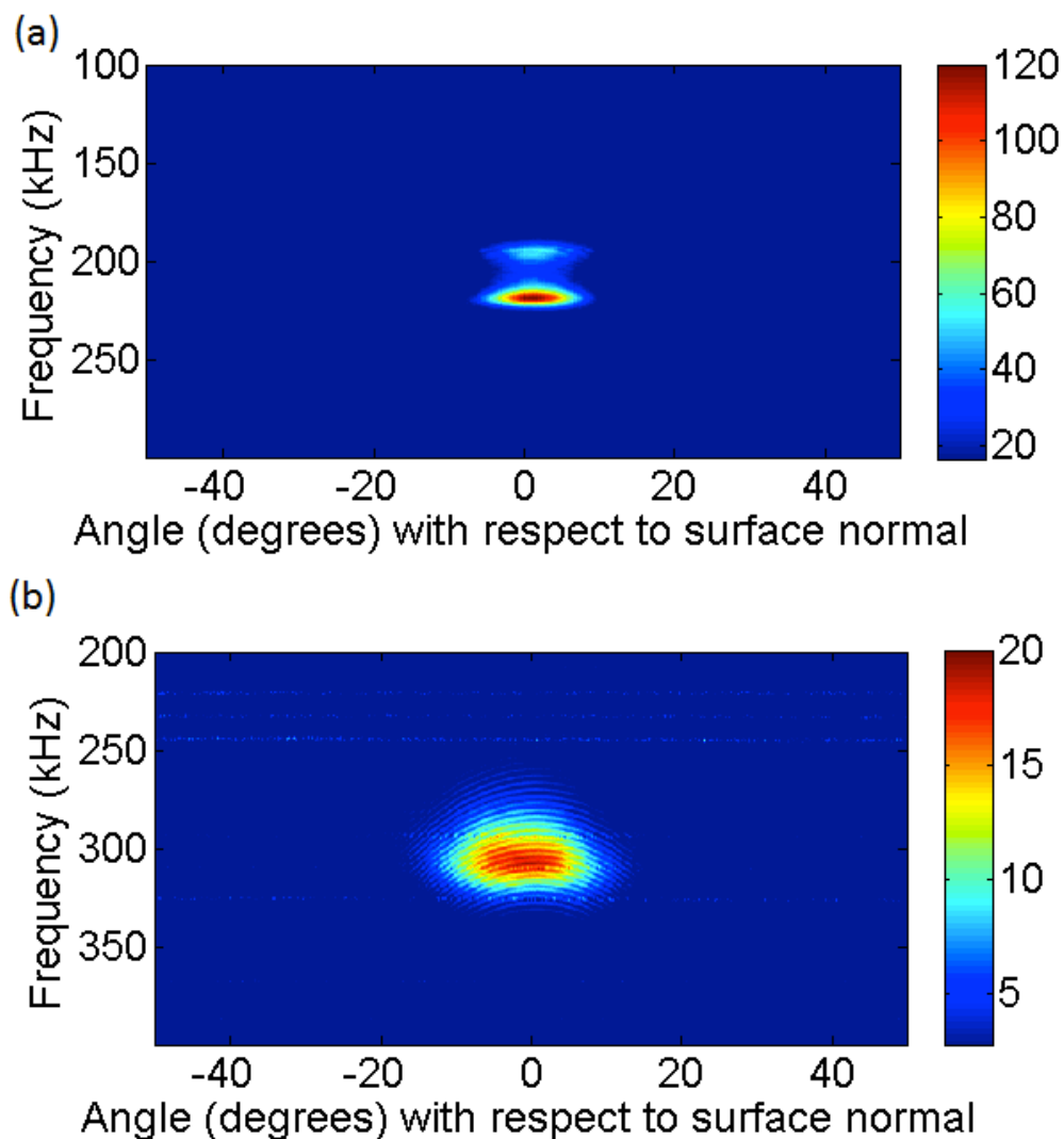
Figure 4-3 Comparison of the angular spectrograms of the polar scans on a flat surface of (a) the 220 kHz transducer and (b) the 310 kHz transducer for the purpose of transducer quality evaluation. The minimum intensity is 1/e^2 of the maximum value.
