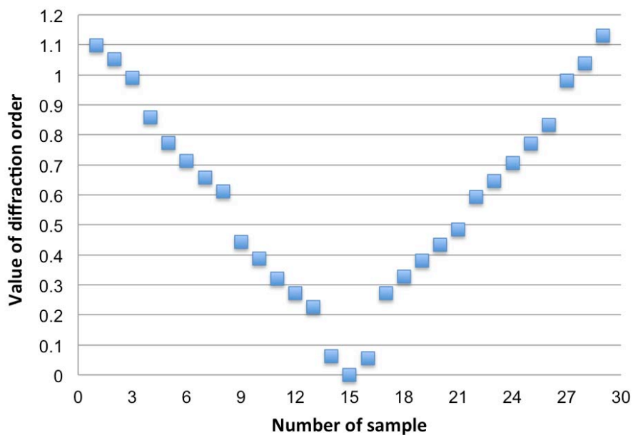
Figure 3-7 Absolute values of all possible diffraction orders from -1 to +1 order of Bragg diffraction. The values are extracted based on experimental data and classical grating equation.
