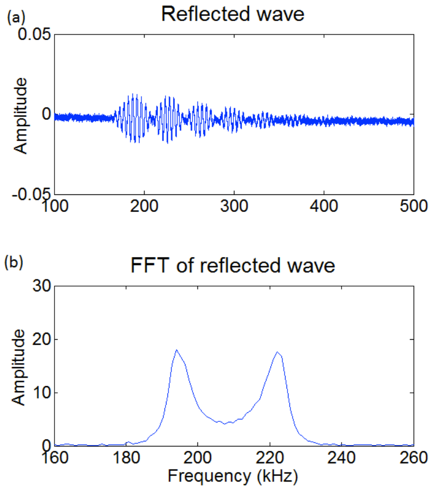
Figure 4-5 (a) Time waveform of a typical reflected wave of the 220 kHz transducer and (b) its frequency spectrum.
