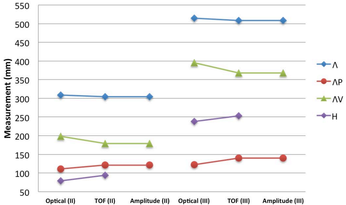
Figure 5-8 Comparison of the average values of the measurements for Sample II and III obtained with optical microscopic technique and the ultrasonic techniques using amplitude and TOF.
