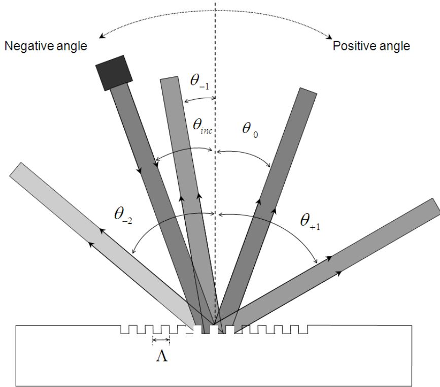
Figure 4-1 Schematic of the diffraction pattern for an acoustic beam incident onto a periodic surface with a periodicity \Lambda . The incident beam, the beam of specular reflection (diffracted beam of zero order), the first positive order diffracted beam, the first and second negative order diffracted beams and their corresponding angles are shown.
