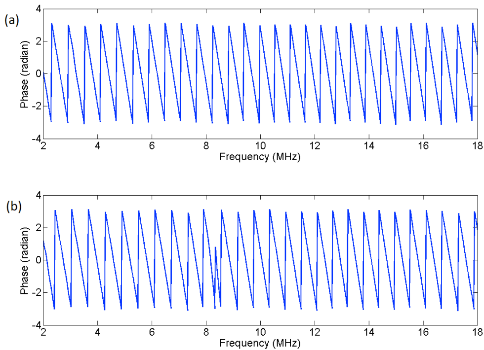
Figure 2-6 Comparison of the phase spectra of the reflection from (a) flat and (b) corrugated water-brass interfaces.
