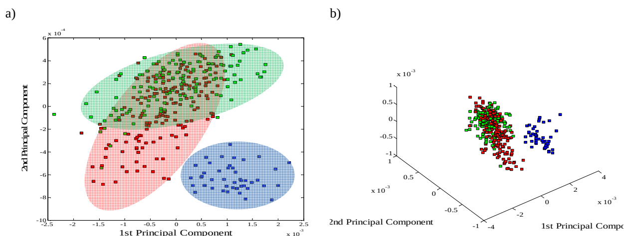
Figure 37 PCA a) score plot on barley spectra in 2D b) score plot in 3D 2009 harvest ■ 2010 harvest ■ 2011 harvest ■. PCA was performed on second derivative spectra in the interval [800-1000] \text{cm}^{-1} . PCA was applied on original data. Two principal components explain 87% of total variance
