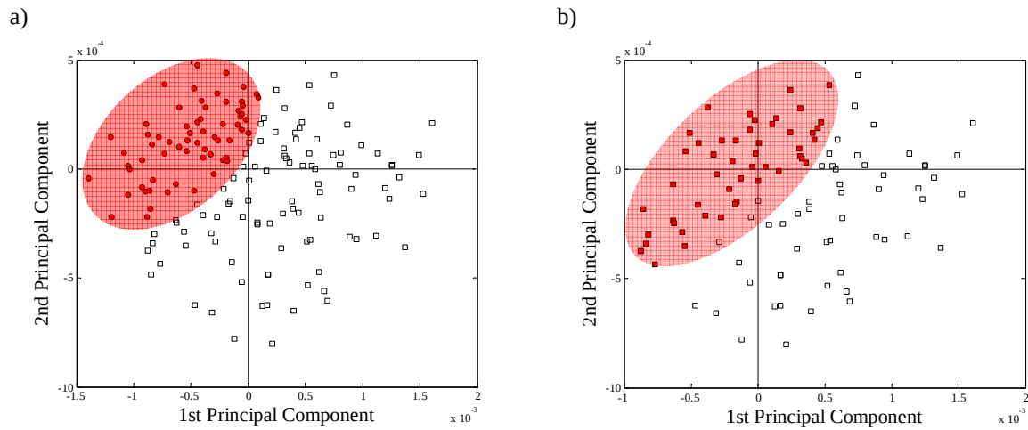
Figure 39 a) PCA score plot on barley 2010 \square winter barley \bullet spring barley. Two principal components explain 89% of the total variance.
