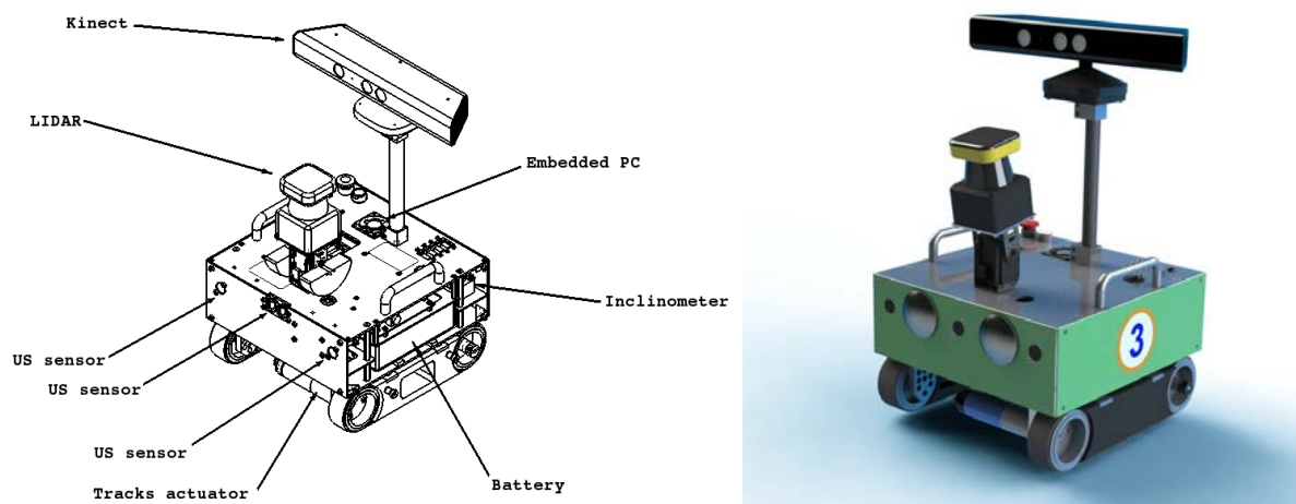
FIGURE 8.1 – Robot MiniRex.
