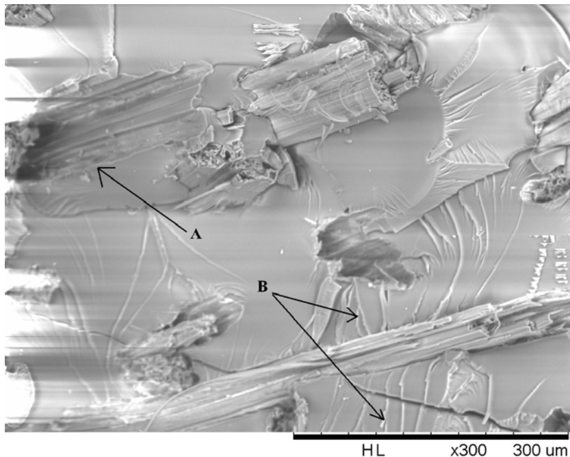
Figure 34: Facies de rupture composite KENAF E
