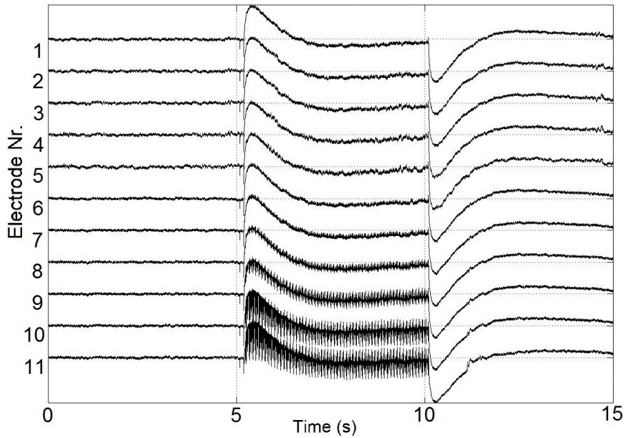
Figure 2.23: Real SEEG stimulation. Measurements of one multi-electrode.
