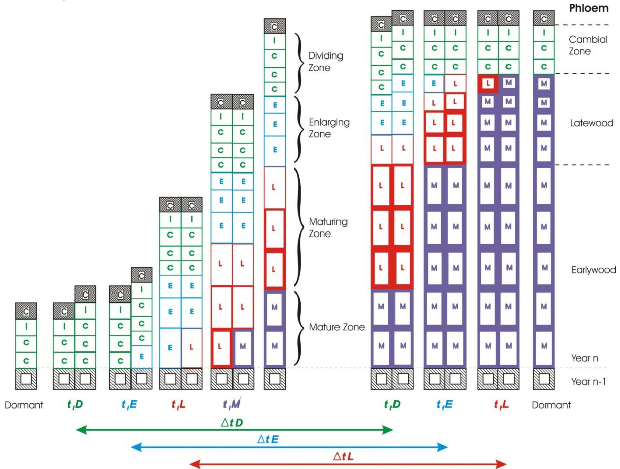
Fig. 1. Illustration of xylem cell development. This drawing illustrates the definitions of critical dates and durations presented in the paper, using two schematic xylem radial files that are developing throughout the growing season. t_{iD} , t_{fD} , t_{iE} , t_{fE} , t_{iL} , t_{fL} , t_{iM} , t_{fM} stands for the beginning of dividing, enlarging, maturing and mature phases respectively; while t_{fD} , t_{fE} and t_{fL} stands for the end of dividing, enlarging, maturing and mature phases respectively; and \Delta t_D , \Delta t_E and \Delta t_L stands for the durations of dividing, enlarging and maturing phases respectively. Cambial cells are noted as C, enlarging cells: E, maturing cells: L and mature cells: M.
