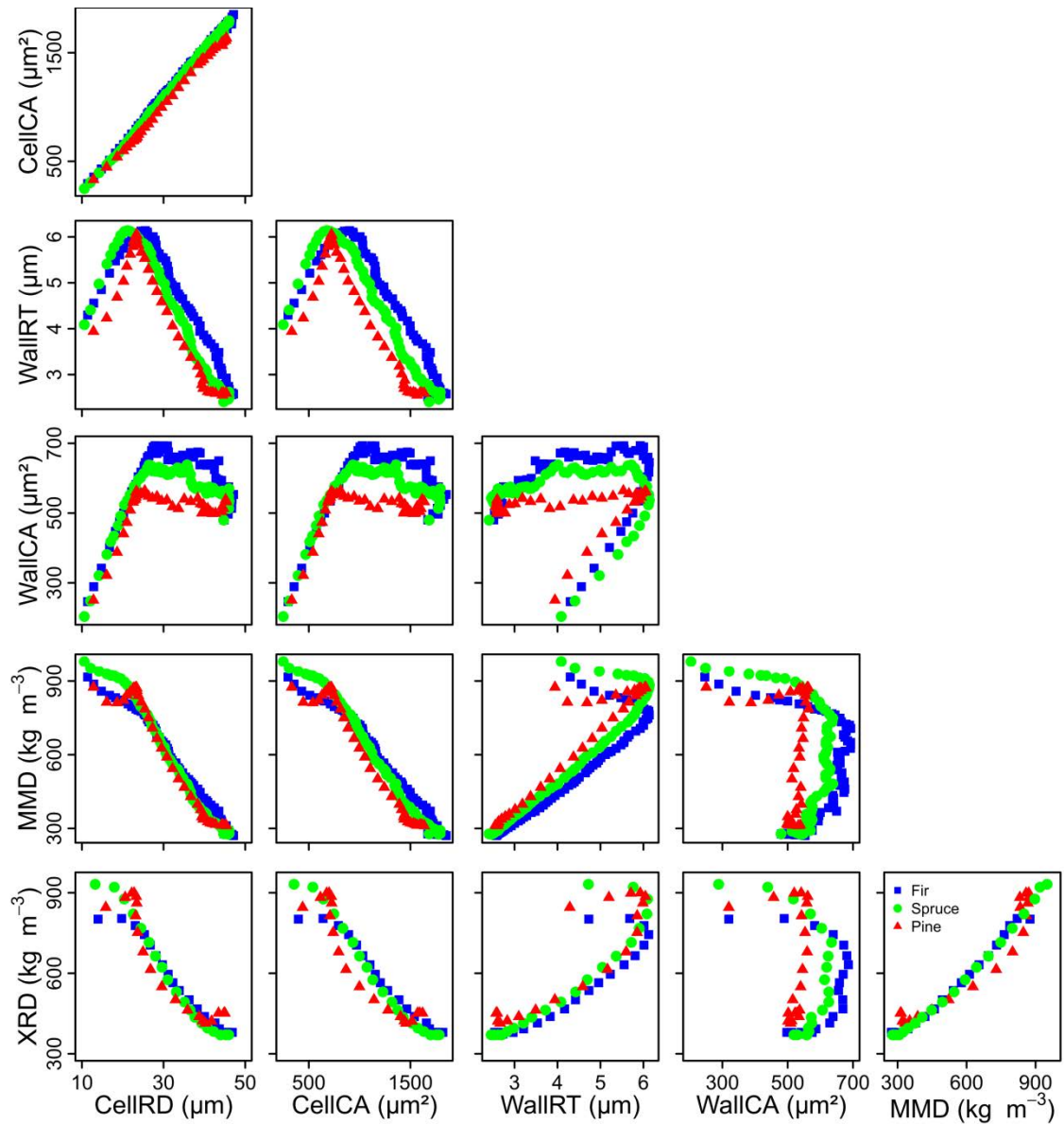
Figure VI.S4: Relationships between the variables of the tree ring structure. Relationships between the tracheid radial diameter (CellIRD), cross-sectional area (CellCA), wall thickness (WallRT), wall cross-sectional area (WallCA), the morphometric density (MMD) and the x-ray measured density (XRD).
