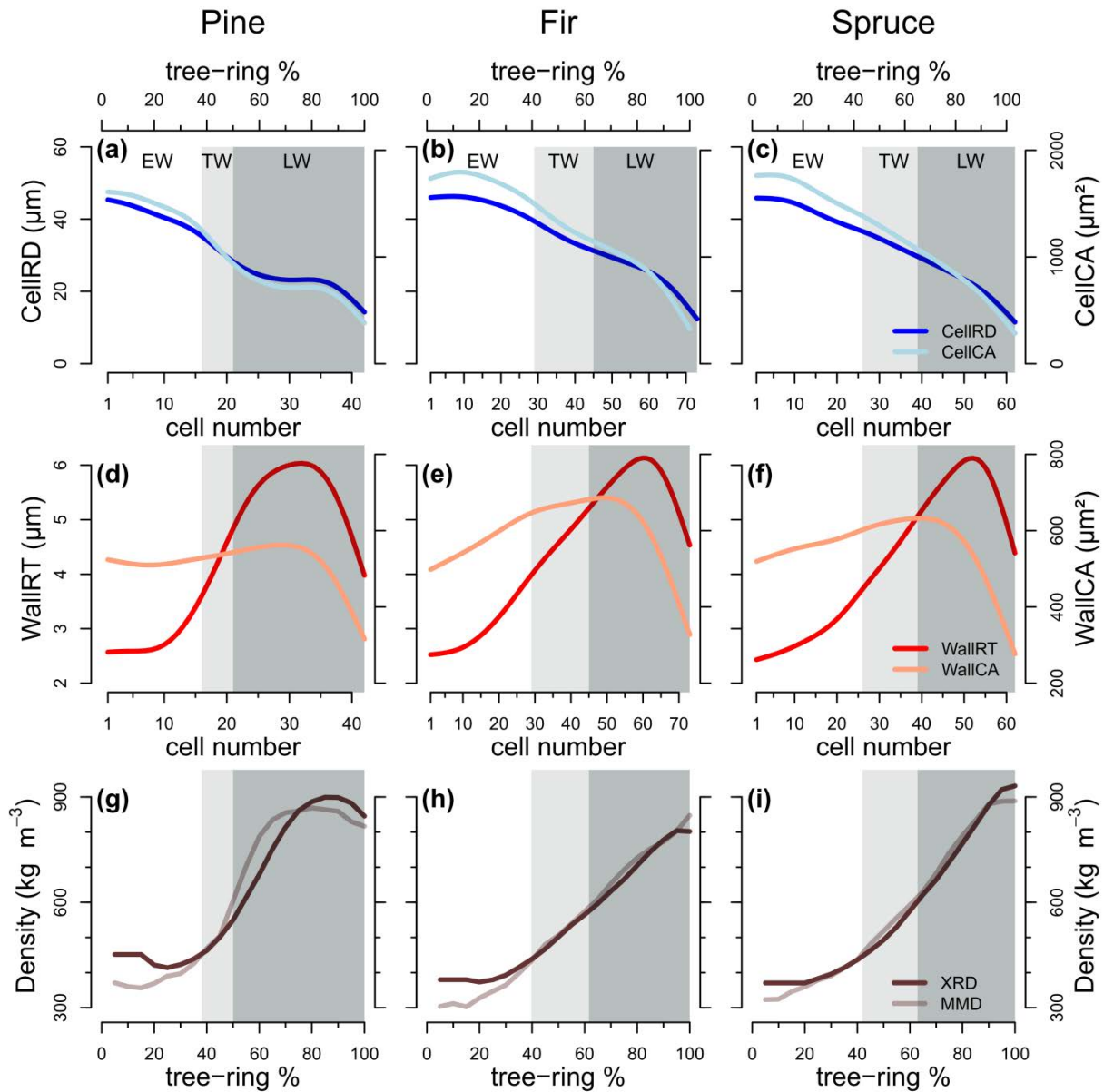
Figure VI.1: Variation in cell (CellCA) and wall (WallCA) cross-sectional area, cell radial diameter (CellIRD), cell wall radial thickness (WallRT), and x-ray measured density (XRD) and morphometric wood density (MMD) along tree rings of three conifer species (Scots pine, silver fir, and Norway spruce). For each species, lines represent the mean values for 15 trees over 3 years (2007–2009). White, light-grey, and dark-grey areas represent earlywood (EW), transition wood (TW), and latewood (LW), respectively.
