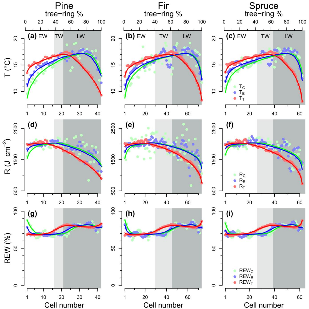
Figure VIII.3: Temperature, global radiation, and relative extractable water when cells were in the cambial ( T_C , R_C , and \text{REW}_C ), enlargement ( T_E , R_E , and \text{REW}_E ) and wall thickening ( T_T , R_T , and \text{REW}_T ) zones. For each species, each point represents a single cell along an average ring (means of 15 trees over three years). Lines represent the global tendencies as revealed by generalized additive models. White, light-grey and dark-grey areas represent earlywood ( E_W ), transition wood ( T_W ), and latewood ( L_W ), respectively.
