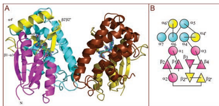
FIGURE 1. Unique dimeric organization of GST5118. A, view of the original dimer of GST5118. The additional secondary structures, highlighted in yellow in the left monomer, include an elongation of the \beta 1 - \alpha 1 loop, a \beta -hairpin motif in the \alpha 2 - \beta 3 loop, and the \alpha -helices \alpha 4' and \alpha 6' . In the left monomer, the N- and C-terminal domains are colored in magenta and cyan, respectively; in the right monomer they are colored in olive and chocolate, respectively. Both monomers have the ability to bind one glutathione molecule, depicted as green sticks, with corresponding 2F_o - F_c electron density (contour level 1.2 \sigma ). B, topology diagrams of GST5118 (circles, helices; triangles, strands). The regular secondary structures of GSTs are colored cyan and magenta, whereas original elements are colored yellow.
