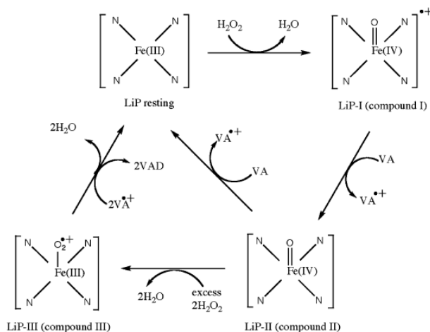
Figure 38 : Cycle catalytique des lignine peroxydases (Wong, 2009).
