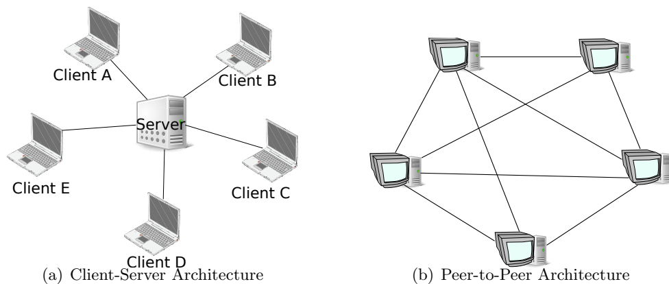
Figure 3.1: Network Architectures
