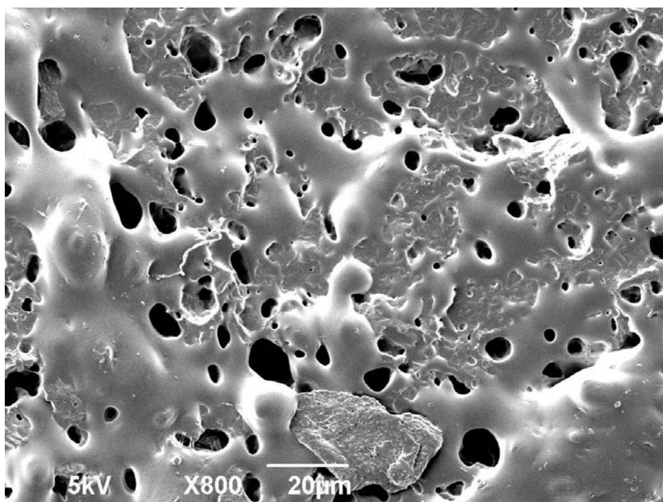
Figure 4.10 SEM images of PBA/PLA (20/80) blend while composite surfactant-0.5gBrij700 with 2g PEGMEM was used in the preparation of PBA latex. dn=1.57 \mu m , dv=5.05 \mu m .
