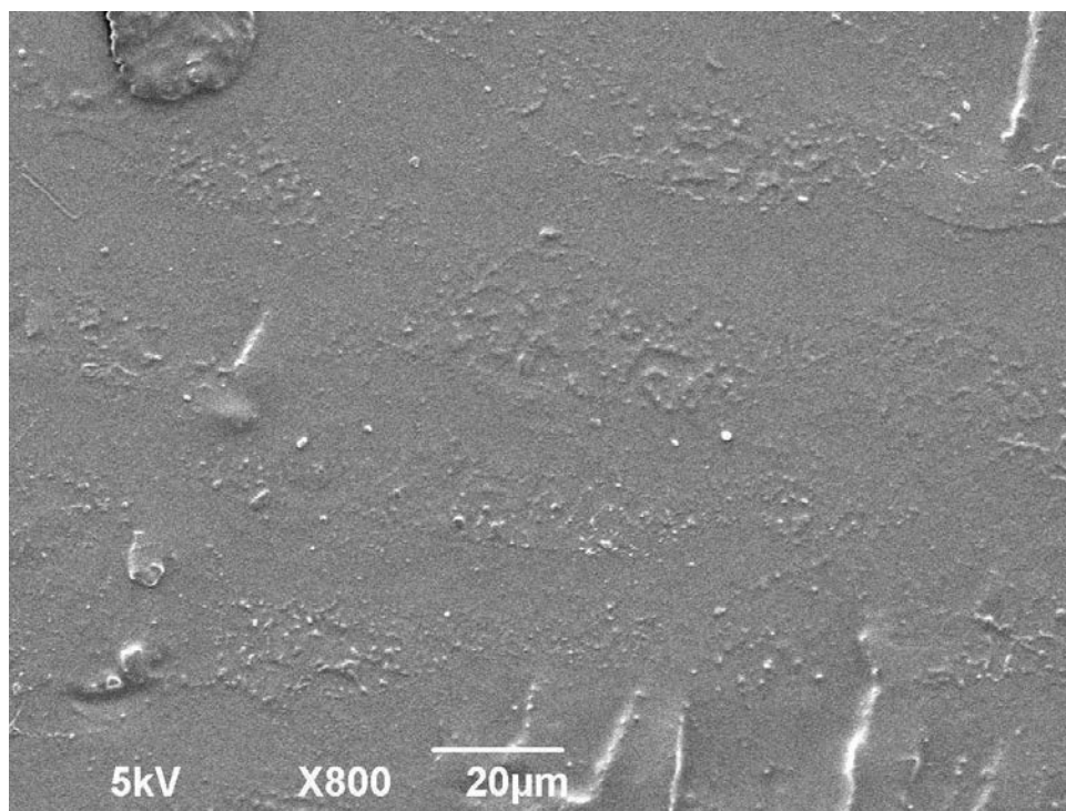
Figure 5.12 SEM fractograph of PLA after impact fracture testing.
