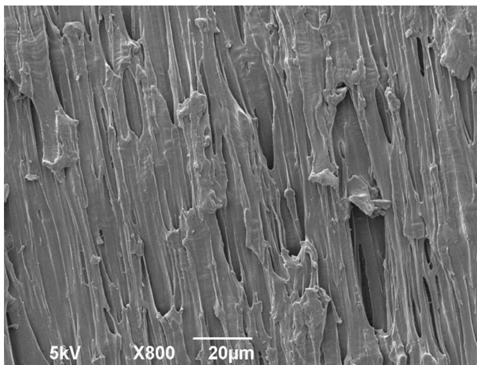
Figure 5.11 SEM fractograph showing fibrous characteristic of specimen PBA/PLA (20/80) after the tensile test. It is the outside surface of the specimen chosen in the necking part and the surface is parallel to the stress direction.
