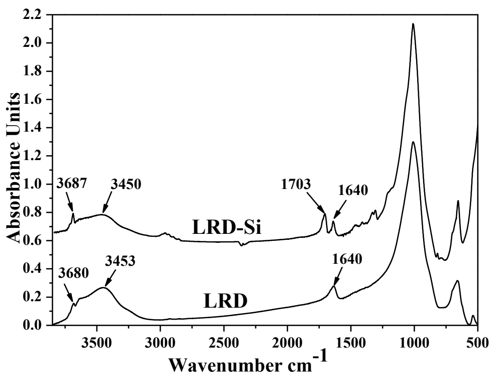
Figure 3.15 FTIR spectra of the bar LRD and MPTMS grafted LRD (LRD-Si).
