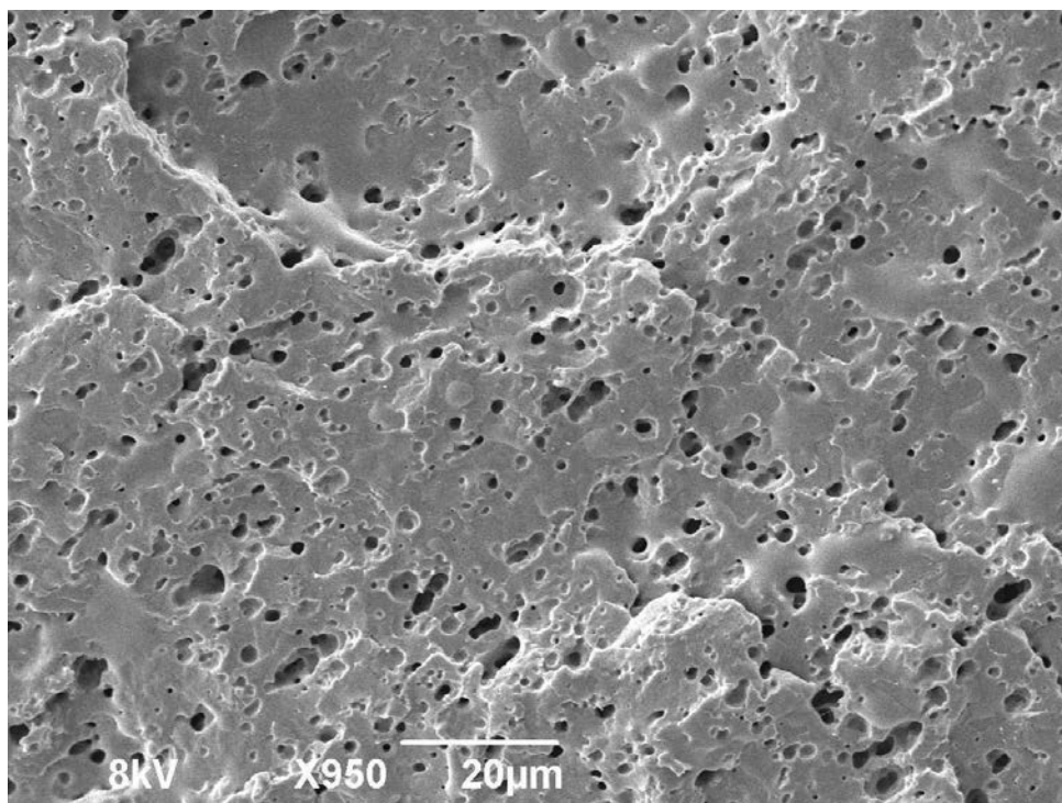
Figure 4.6 SEM images of PBA/PLA (20/80) blend. dn=1.12\ \mu\text{m} , dv=1.78\ \mu\text{m} .
