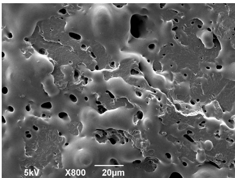
Figure 4.11 SEM images of PBA/PLA (20/80) blend while composite surfactant-1 gBrij700 with 2g PEGMEM was used in the preparation of PBA latex. dn=1.63 \mu m , dv=3.89 \mu m .
