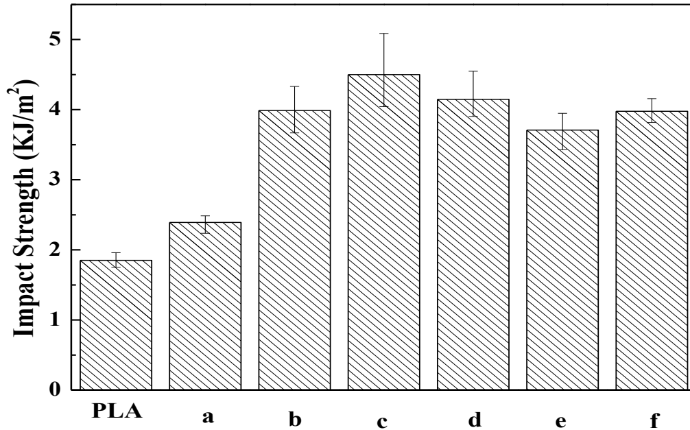
Figure 5.8 Impact strength of pure PLA, PBA/PLA blends: (a) PBA/PLA (20/80) blend, (b) PBA-2%LRD-Si/PLA (20/80) blend, (c) PBA-5%LRD-Si/PLA (20/80) blend, (d) PBA-5%LRD/PLA (20/80) blend, (e) LRD/PLA/PBA (1/79/20) blend, and (f) PBA-3%LRD-Si-3G/PLA (20/80) blend.
