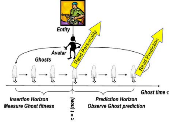
Figure 2.7 – In the polyagent approach each avatar generates a stream of ghosts that sample the personality space of its entity. They evolve against the entity’s recent observed behavior, and the fittest ghosts run into the future to generate predictions. Taken from (Parunak and Brueckner, 2006a)
