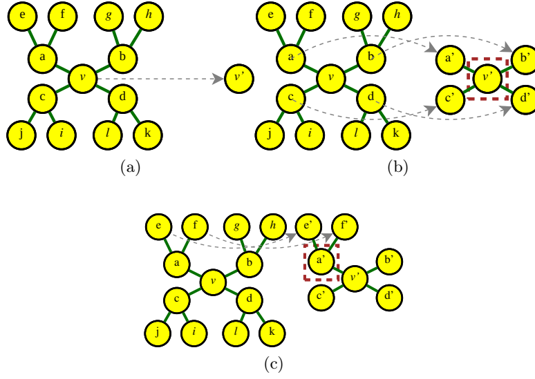
Figure 4.5 – (a) We first select a random node v from the original graph and add it to our model. (b) We add all the neighbors of v in the model. (c) We randomly select a neighbor ( a' ) of v in the original graph and add all of its neighbors to the model.
