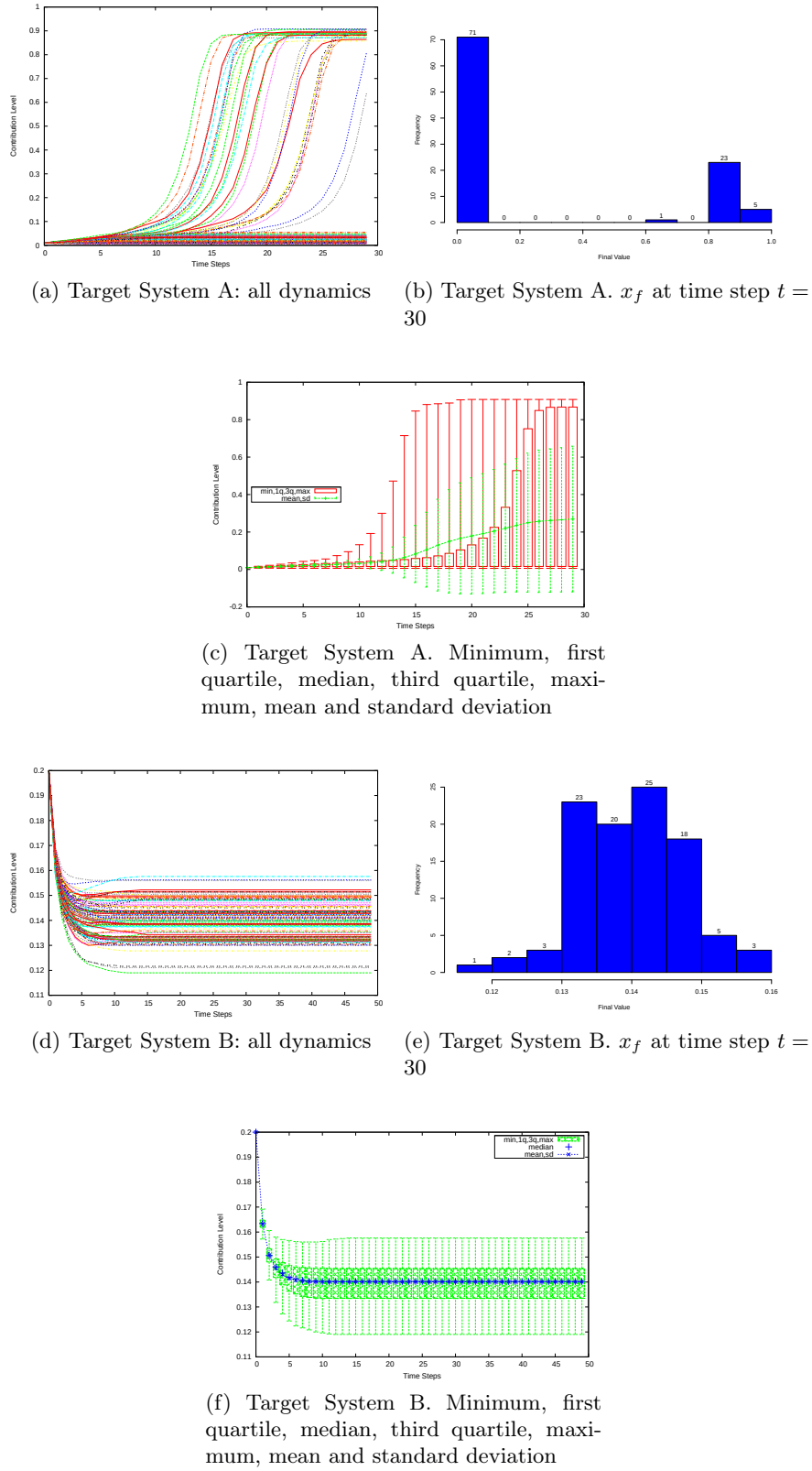
Figure 5.1 – Nominal behavior of target systems A (a, b, c) and B (d, e, f). For each time step, the contribution level of the target system.
