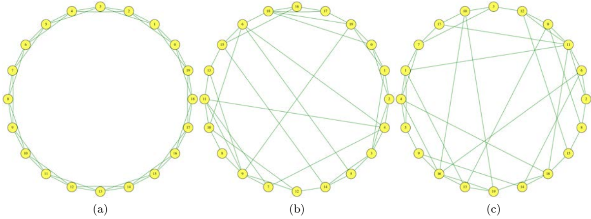
Figure 4.1 – Example graphs generated with the algorithm of (Watts and Strogatz, 1998) with N = 20 initial nodes and k = 4 neighbors per node. (a) p = 0 (circular lattice), (b) p = 0.25 (small-world graph), (c) p = 1 (random graph)
