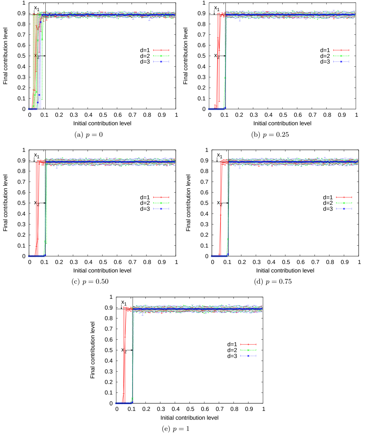
Figure 4.3 – Summary of results of preliminary study on the target. Each figure shows the global dynamics of the network in terms of the “contribution level”. Each image depicts the average contribution level found after 200 time steps and after conducting 1000 repetitions.
