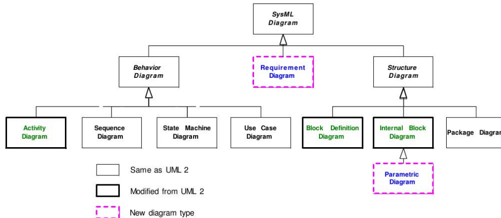
Figure 3.2 – SysML Diagram Taxonomy, taken from (SysML Specification, 2012). The generalization and specification notation of UML is used.
