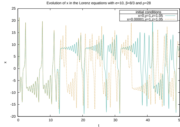
Figure 1.1 – The evolution of x in the Lorenz equations, with initial conditions differing only in the x variable by 1 \times 10^{-05} .
