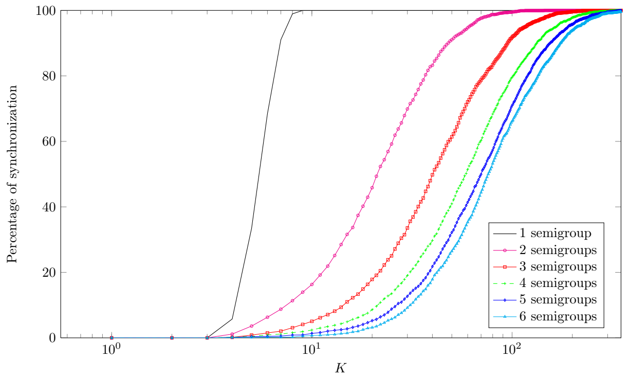
Figure 3.3: Percentage of the number of times the system \mathcal{E}\text{--}\mathcal{D} has synchronized with respect to the delay of synchronization for different number of nilpotent semigroups.
