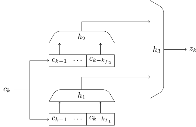
Figure 2.10: Parallel composition
