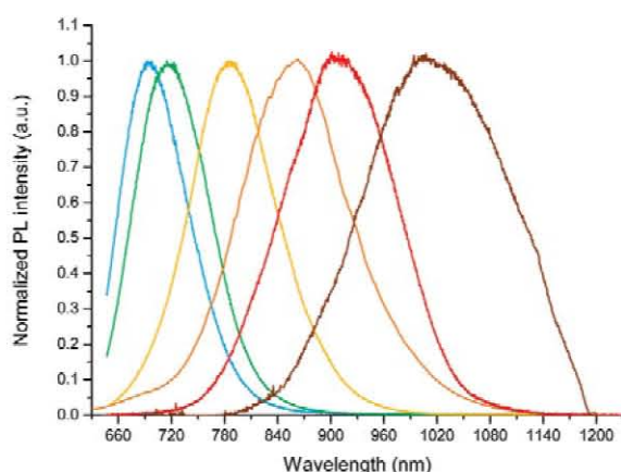
Figure 8. PL spectra of Cu–In–Se/ZnS QDs corresponding to core samples synthesized at, from left to right, T_f = 140, 160, 200, 220, and 250 °C with fast heating and 250 °C with intermediate heating. The emission maxima range from 700 nm to \sim 1030 nm.
