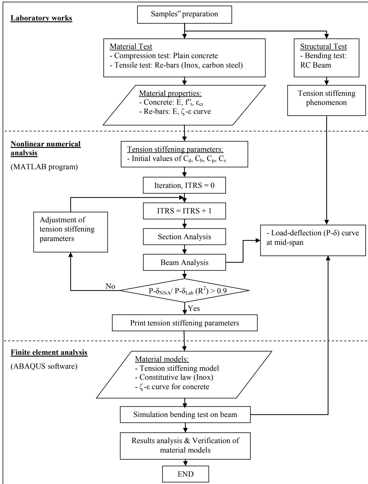
Fig. 3.13. Process to develop the interaction model for inoxydable steel in composite concrete
