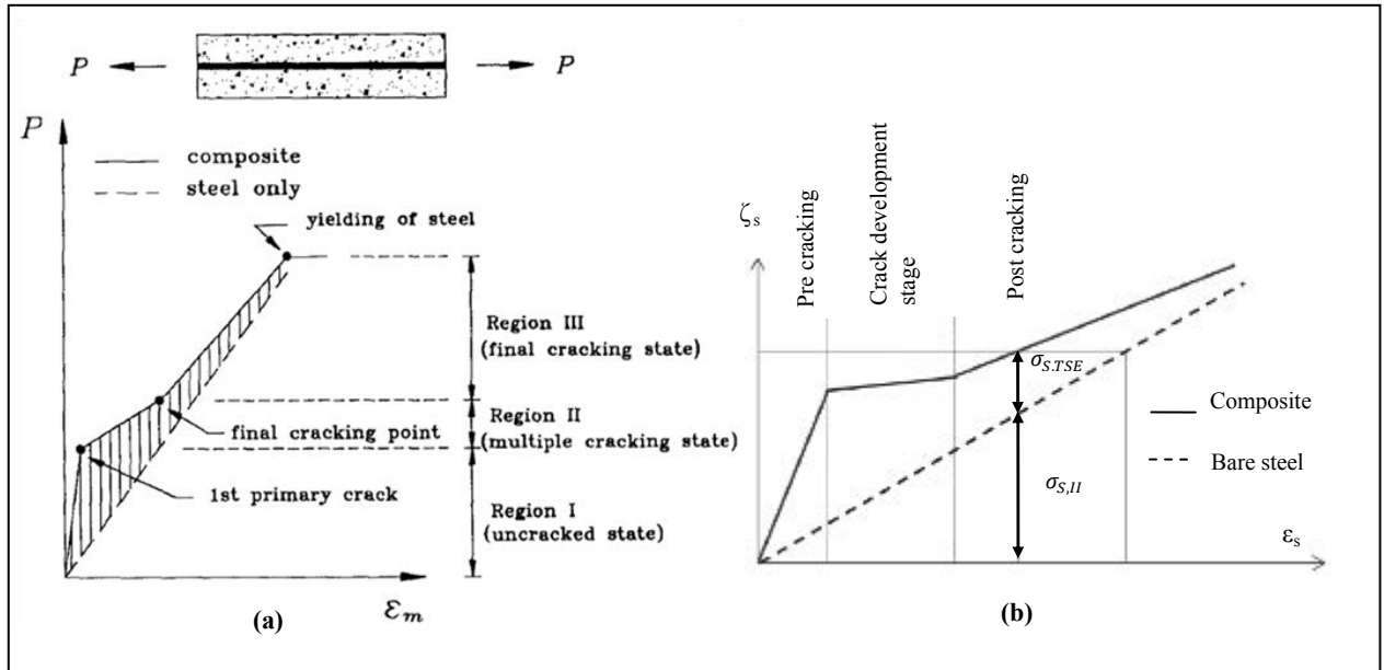
Fig. 2. 5 Phenomenon to account for tension stiffening effect in RC sample under uniaxial tension (a) load-average strain curve [27], (b) stress-strain relationship for a composite and embedded reinforcing bar [8], [9].
