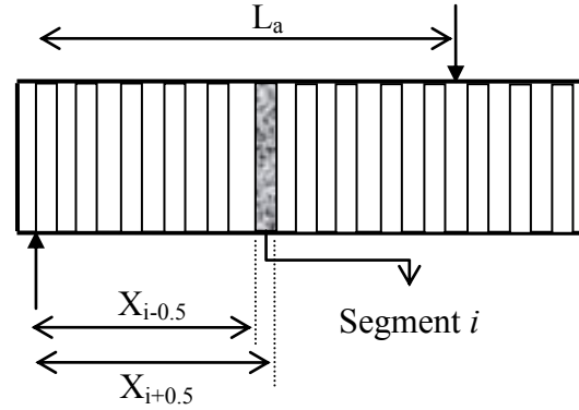
Fig. 3.34. Vertical segment of the beam analysis
