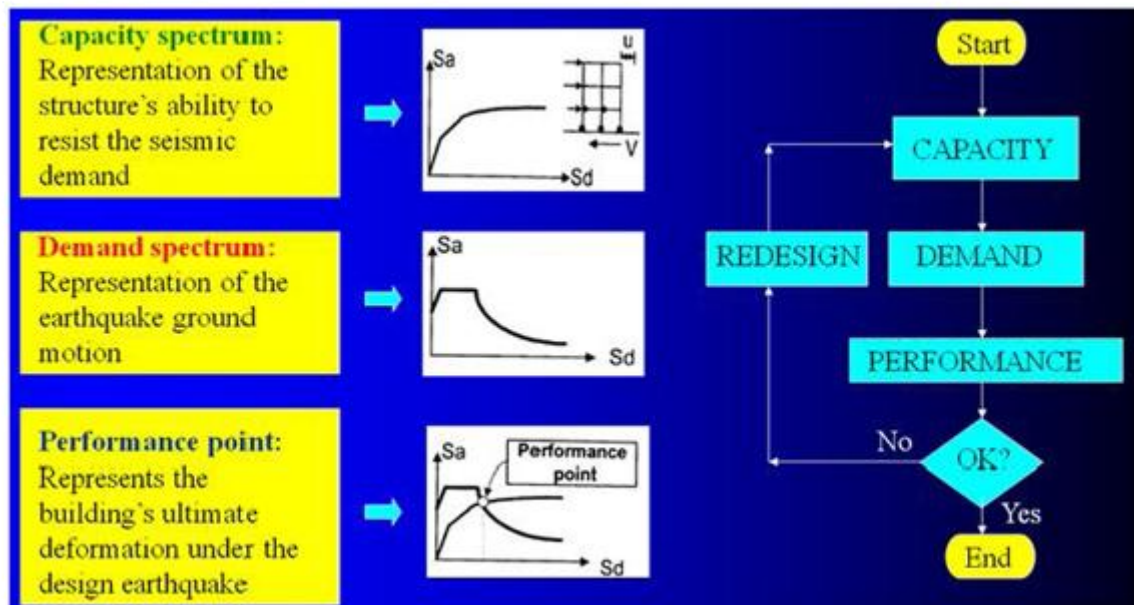
Fig. 2. 14 Simple Push-over method of evaluation [33]
