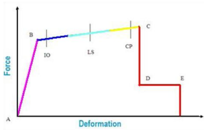
Fig. 2. 13 The force deformation criteria for hinges [34]
