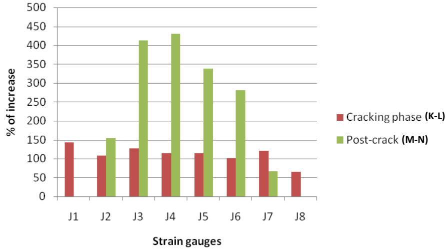
Fig. 3.25. Stress increase recorded in strain gauges
