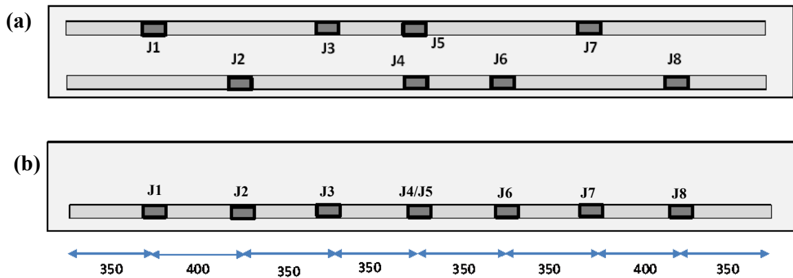
Fig. 3.21. Beam reinforced with AC; detailing position for each strain gauges along the rebar: (a) Position on both re-bars as per plan view, (b) Side view of the RC beam showing the continuous position of the gauges
