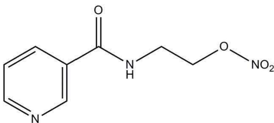
Nicorandil
