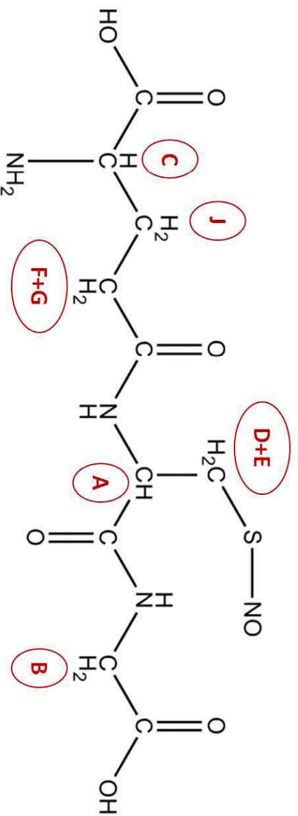
Figure 26 : Spectre 1 H RMN du GSNO
