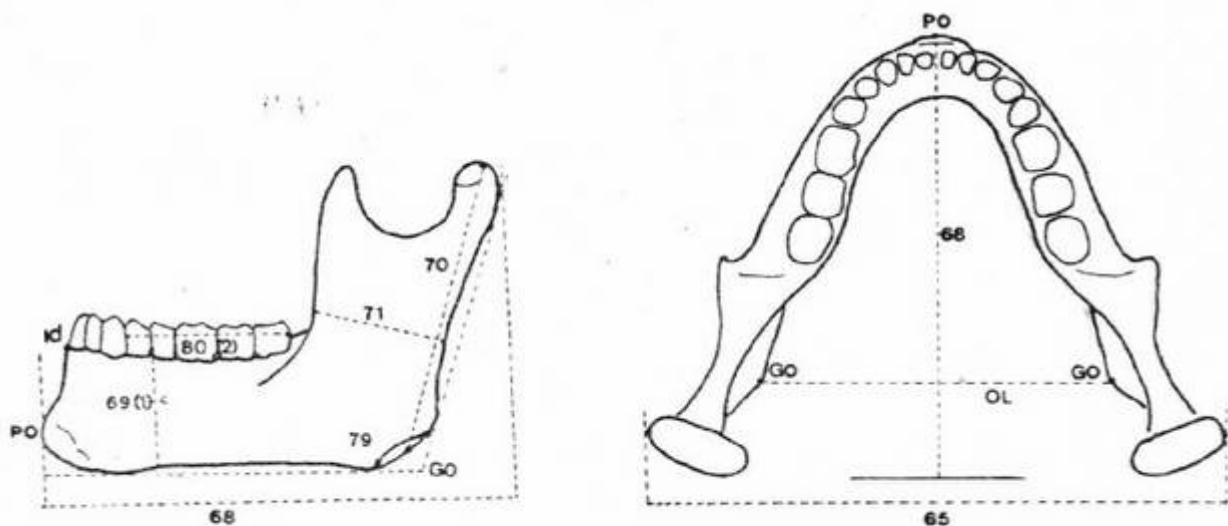
Figure 42 : Mandibule
