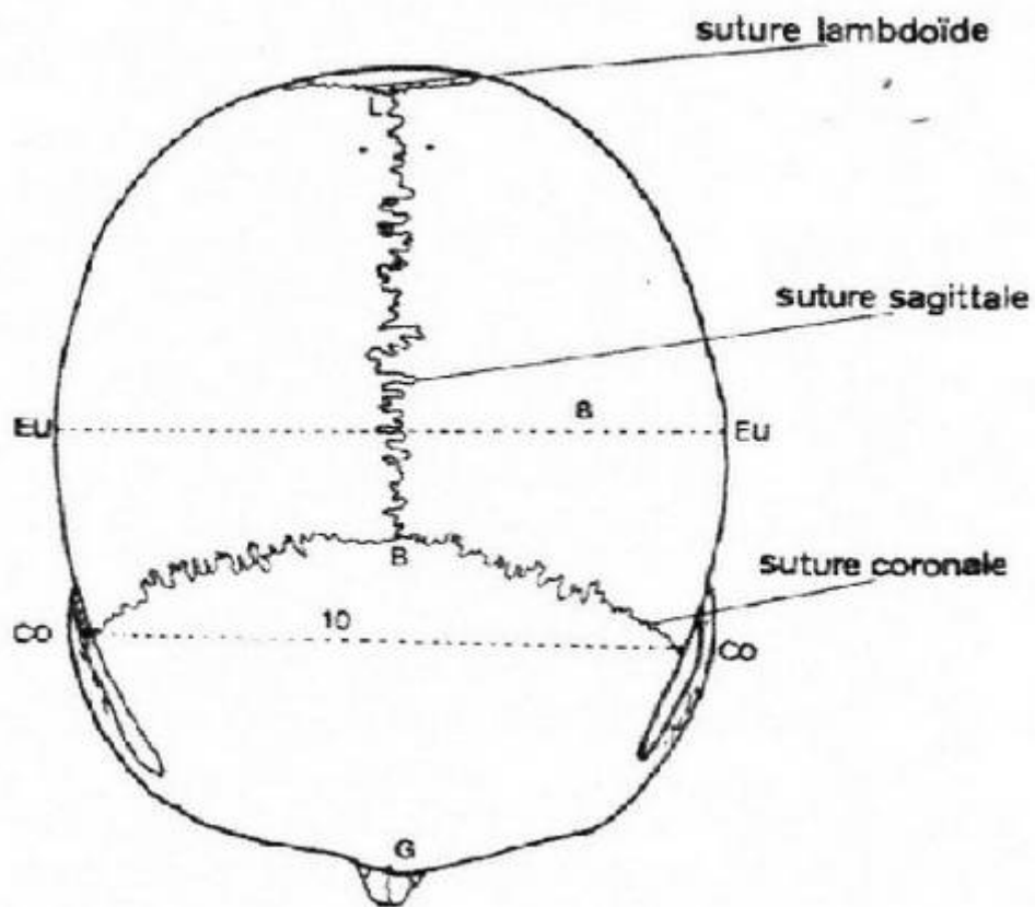
Figure 38 : Norma verticalis
