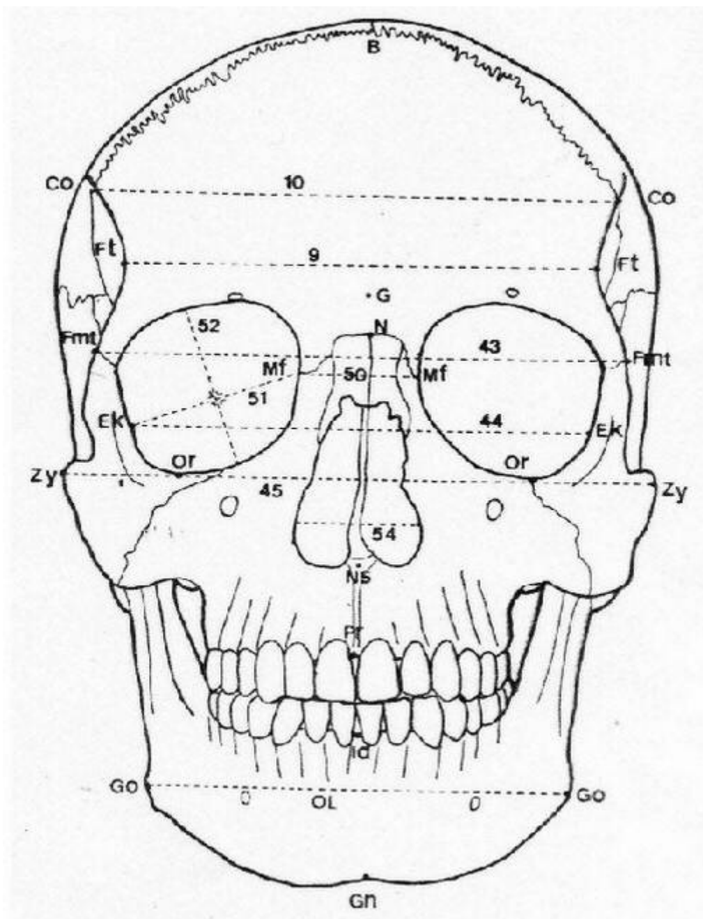
Figure 37 : Norma facialis
