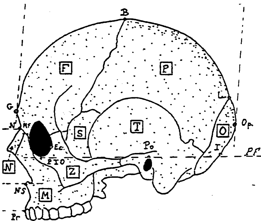
Figure 39 : Norma lateralis
