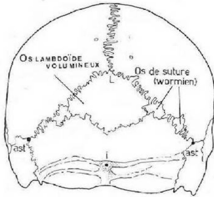
Figure 40 : Norma occipitalis
